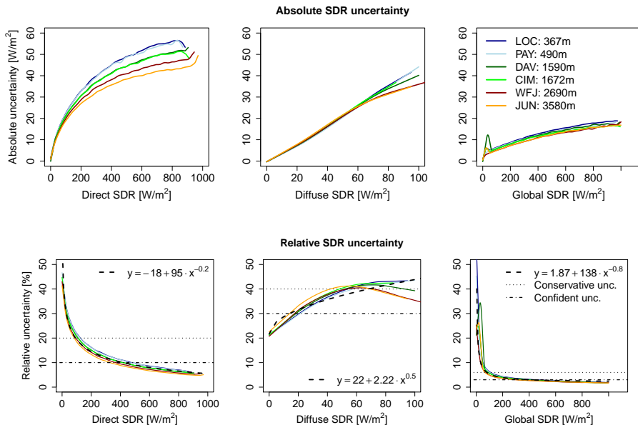
Fig. 6. Uncertainty expressed as smoothed mean lengths of the standard deviation of clear-sky direct, diffuse and global SDR, as a function of radiation [ \text{W m}^{-2} ]. The graphs were obtained by estimating the mean standard deviation of each 5 \text{ W m}^{-2} radiation interval. Smoothing was performed using non-parametric regression. The dashed black line denotes the fit of the function f(\text{SDR}) = \sigma_{\text{SDR},\text{rel}} , where x := \text{SDR}_i and y := \sigma_{\text{SDR}_i,\text{rel}} . The coefficients of the function f(x) = y were obtained by non-linear least-squares regression.
