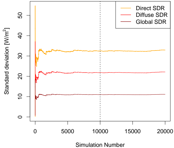
Fig. 2. Standard deviations of the model simulations at Cimetta. 10 000 model simulations result sufficient to reach stable standard deviations of the output frequency distribution.
