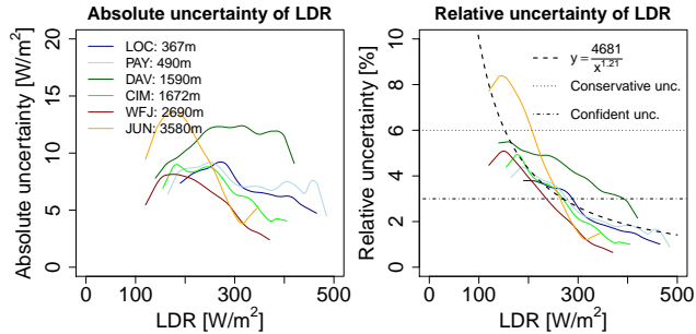
Fig. 11. Absolute and relative uncertainty of the modeled LDR. The clear-sky emissivity is estimated according to Konzelmann et al. (1994), and the all-sky parameterization is found in Eq. 23. The dashed black line denotes the fit of the function f(\text{LDR}) = \sigma_{\text{LDR,rel}} , where x := \text{LDR} and y := \sigma_{\text{LDR,rel}} .
