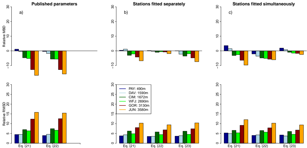
Fig. 8. MBD and RMSD for the LDR parameterizations using a) the published parameter values by Pirazzini et al. (2001), b) the parameter values when fitting the parameterizations to each station separately and c) when fitting all stations together simultaneously. Clear-sky emissivity is estimated based on the Konzelmann et al. (1994) parameterization, using the parameters fitted for all stations simultaneously.
