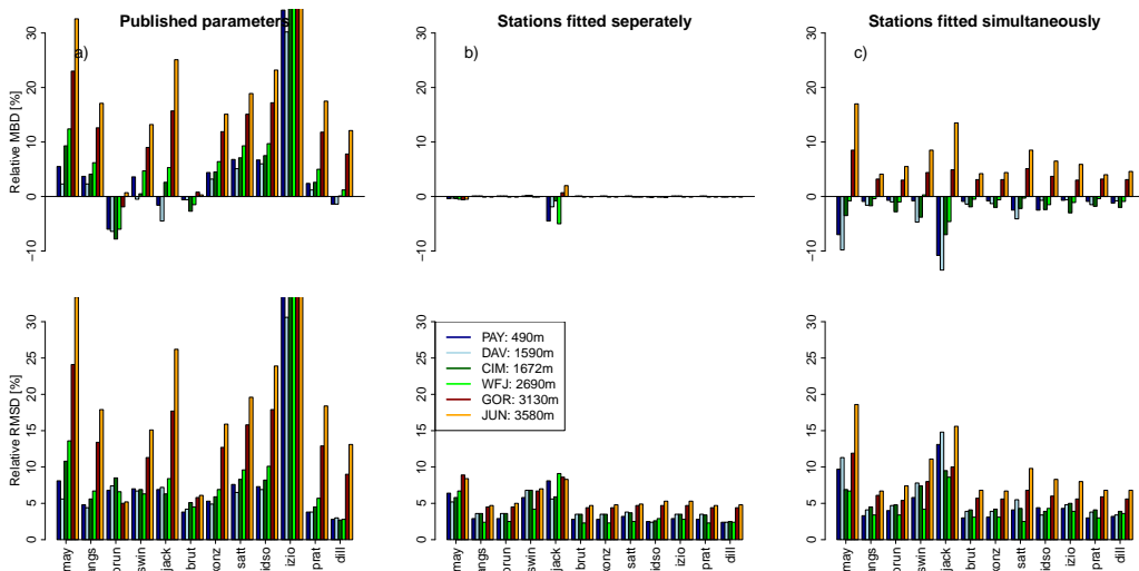
Fig. 7. MBD and RMSD for the LDR parameterizations using a) the published parameter values, b) the parameter values when fitting the parameterizations to each station separately and c) when fitting all stations together simultaneously.
