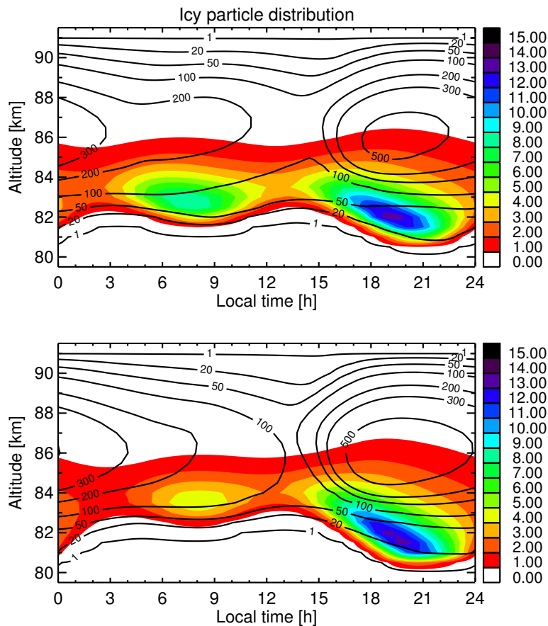
Fig. 1. Modelled icy particles at 75°N the period of one day (14 January). Upper panel: Simulation with 2 K diurnal amplitude. Lower panel: Simulation with 4 K diurnal amplitude
