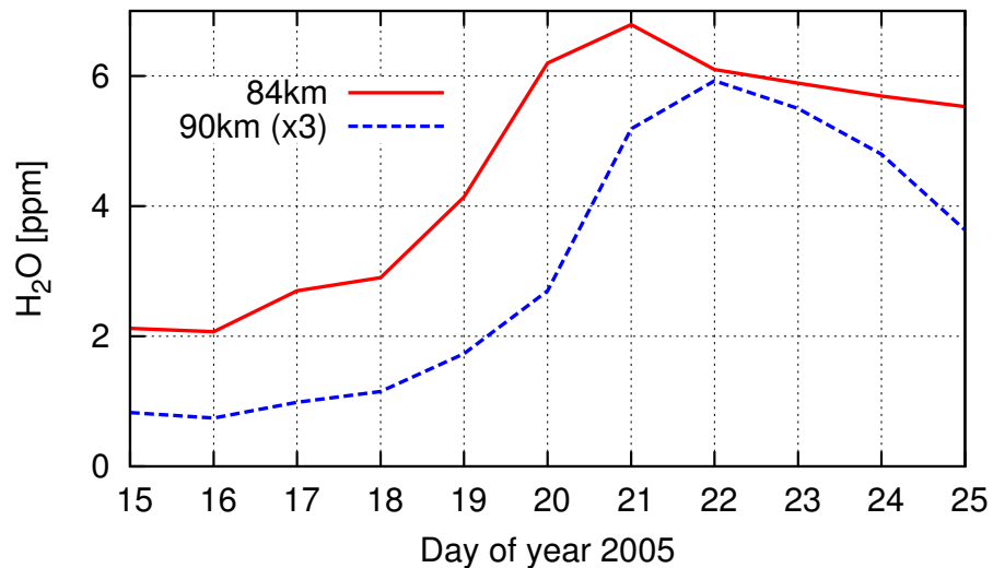
Fig. 3. Modelled H 2 O [ppm] at two altitudes, the solid red line shows water at 84 km, and the dashed blue line water at 90 km increased by a factor of three.
