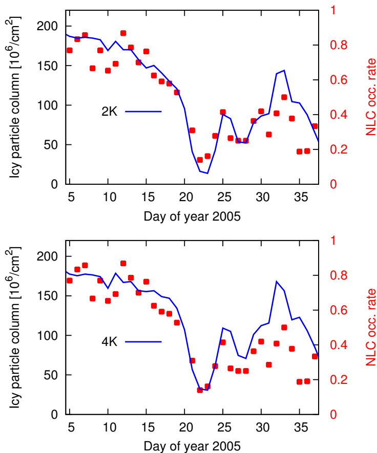
Fig. 2. Total column of icy particles. Upper panel: Simulation with 2\,K diurnal amplitude. Lower panel: Simulation with 4\,K diurnal amplitude
