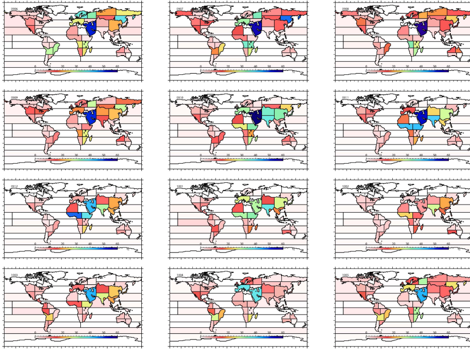
Fig. 3. Fig C Uncertainty reduction rate by month
