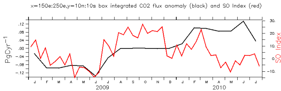
Fig. 4. Fig D IAV of oceanic flux in Trop. Pacific
