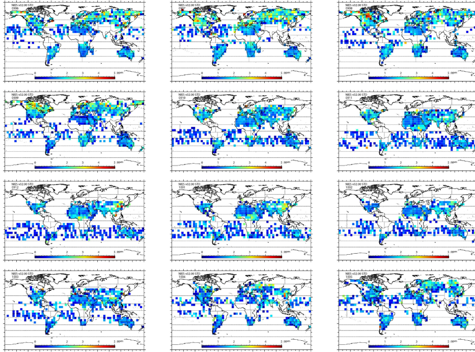
Fig. 1. Fig A Distribution of GOSAT L2 standard deviations
