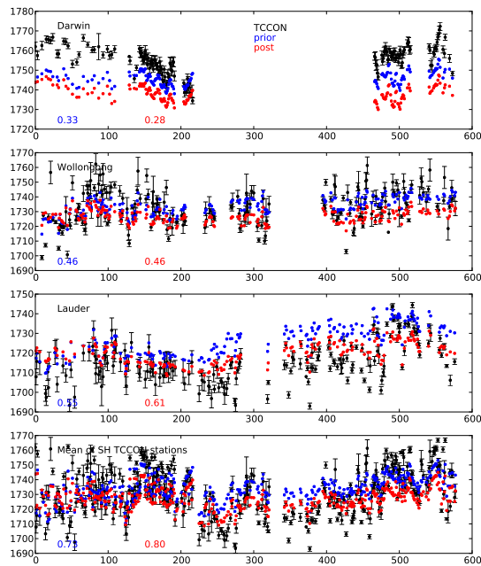
Fig. 3. Measured and modelled TCCON XCH 4 at Southern Hemisphere stations. Numbers on the figures are r-squared values of the correlation between observations and the model.
