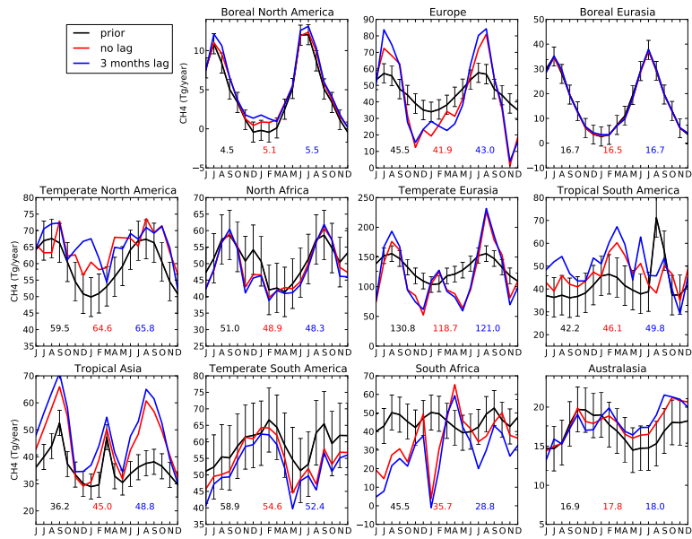
Fig. 2. Effect of lag window on inversion results. The inset numbers are the average flux in the region from the prior (black), no lag (red), and 3 month lag (blue) fluxes.
