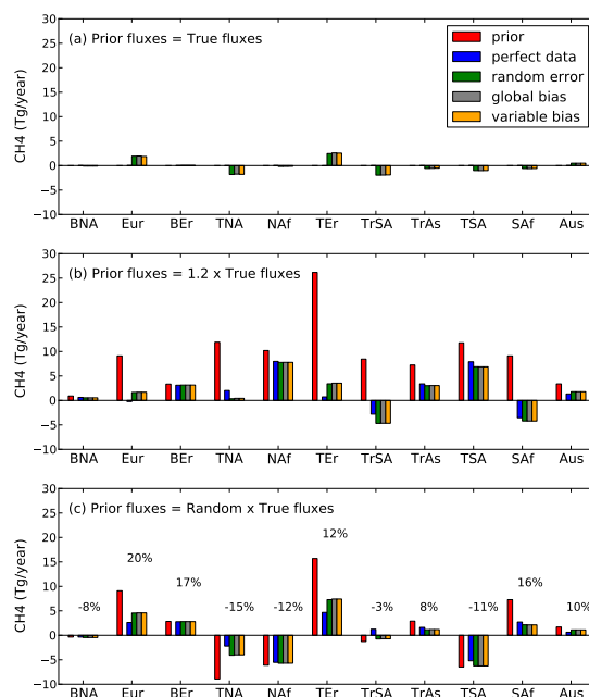
Fig. 1. New Figure 8, showing results of all the experiments adjusting the prior fluxes.
