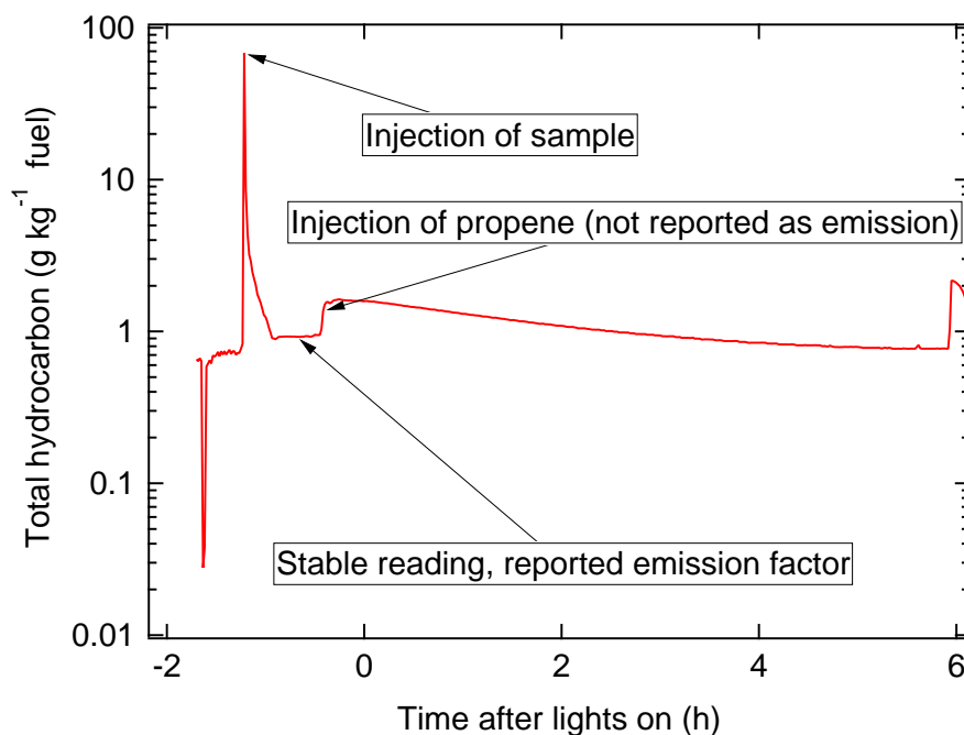
Fig. 1. : Total hydrocarbon (g kg -1 fuel) as a function of time after lights on in the smog chamber during experiment two.
