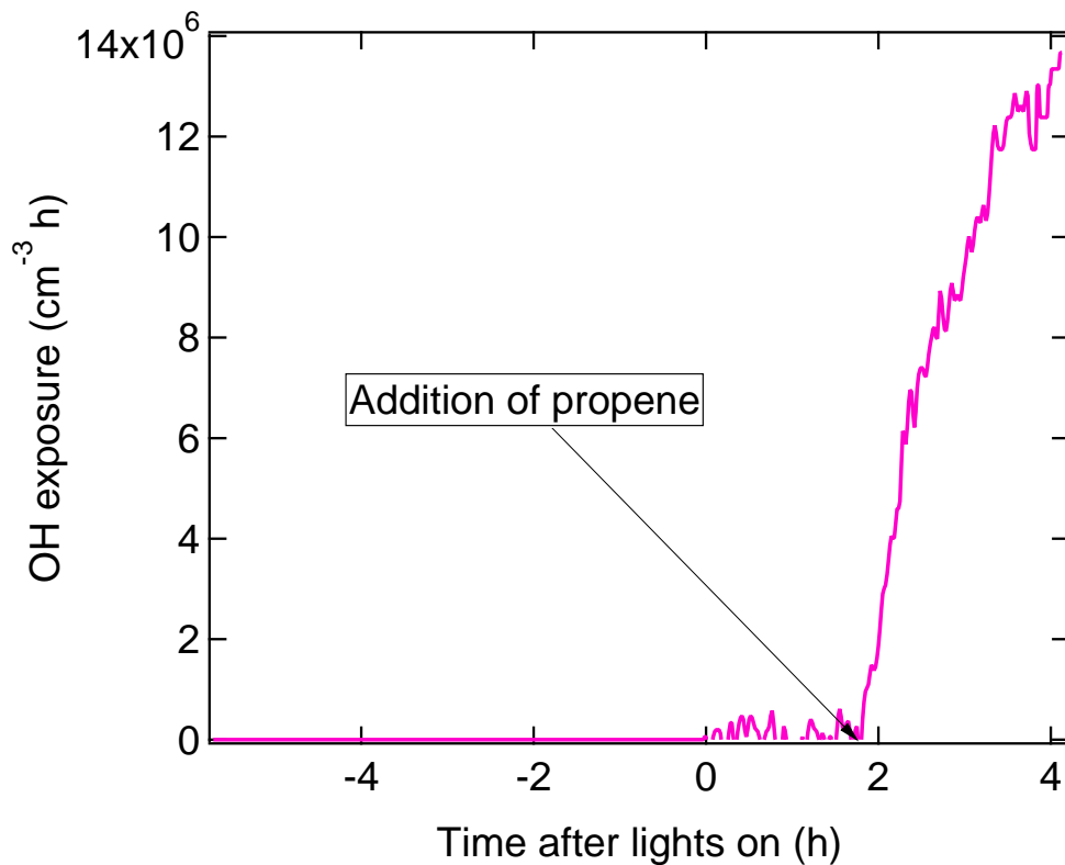
Fig. 6. OH exposure ( \text{cm}^{-3} \text{ h} ) in the smog chamber during Exp. 1. The addition of propene two hours after lights on was observed to significantly enhance photochemistry in the chamber.
