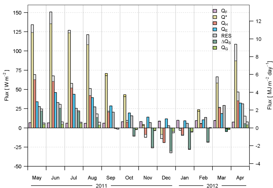
Fig. 1. Monthly mean fluxes for all available data (average of 24 h median values for each month), as for Figure 4 (colours), and for all concurrent data (unfilled bars). (Note the y-axis has been adjusted.)
