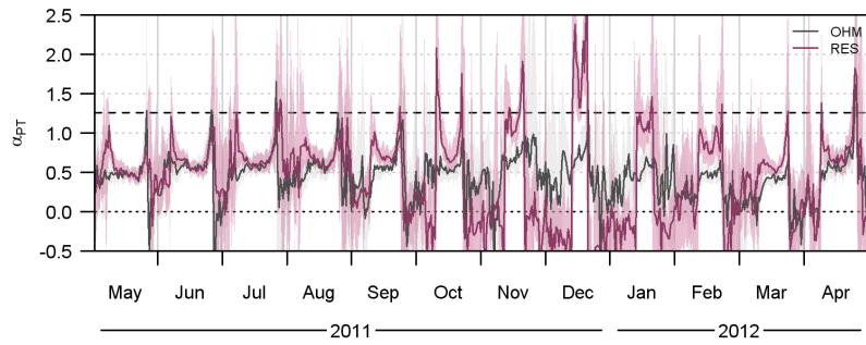
Fig. 2. Monthly median diurnal cycles (lines) and inter-quartile ranges (shading) of the aridity parameter, \alpha_{PT} , calculated using OHM or RES as the storage heat flux.
