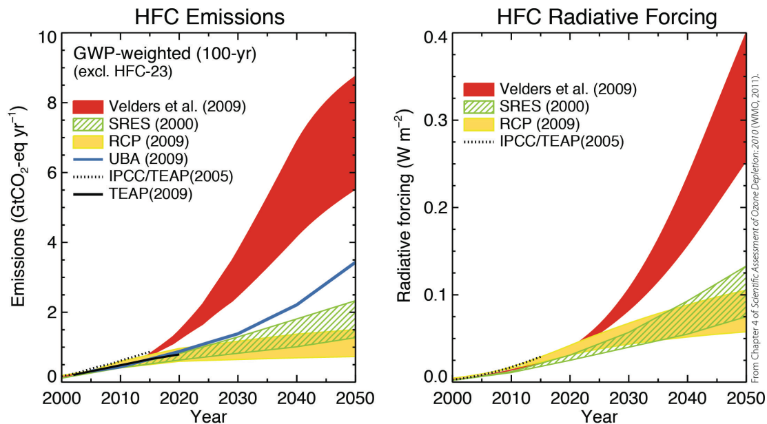
Fig. 1. Figure 5-5 in the WMO (2011) assessment
