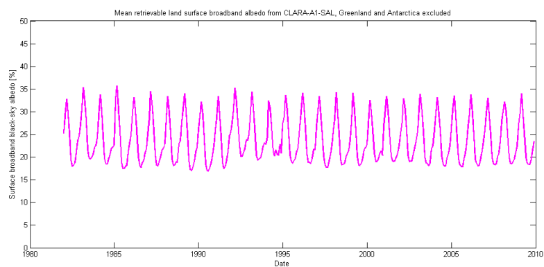
Fig. 3. Mean retrievable land surface albedo from CLARA-A1-SAL. Greenland and Antarctica have been excluded from the analysis.
