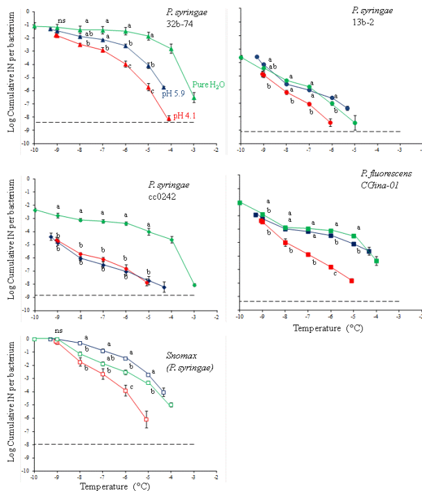
Fig. 2. Ice nucleation spectra of Pseudomonas strains submitted to different pH: pH=4.1 (red), pH=5.9 (blue) and in distilled water as a control (green). Data were corrected for water activity of the buffer and linearly interpolated. The horizontal line corresponds to the lower limit of detectable activity depending on the initial bacterial concentration of each experiment. Symbols are as in Fig. 1. At each temperature, values associated with different letters are significantly different ( p < 0.05 ) based on Tukey's test. Errors bars indicate standard errors ( n = 4 ).
