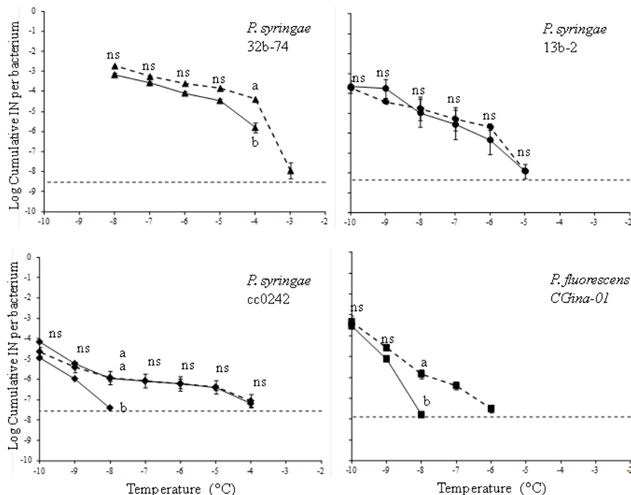
Fig. 3. Ice nucleation spectra of Pseudomonas strains exposed to synthetic gases with (solid line) and without (dotted line) NO 2 and O 3 . The horizontal line corresponds to the lower limit of detectable activity depending on the initial bacterial concentration of each experiment. Symbols are as in Fig. 1. Each symbol corresponds to the mean value of 4 replicates except for P. syringae CC0242 that was exposed to gases with NO 2 and O 3 , where symbols correspond to the mean value of 2 replicates. At each temperature, values associated with different letters are significantly different ( p < 0.05 ) based on Tukey's test. Errors bars are standard errors ( n = 4 , except for P. syringae CC0242 where n = 2 ).
