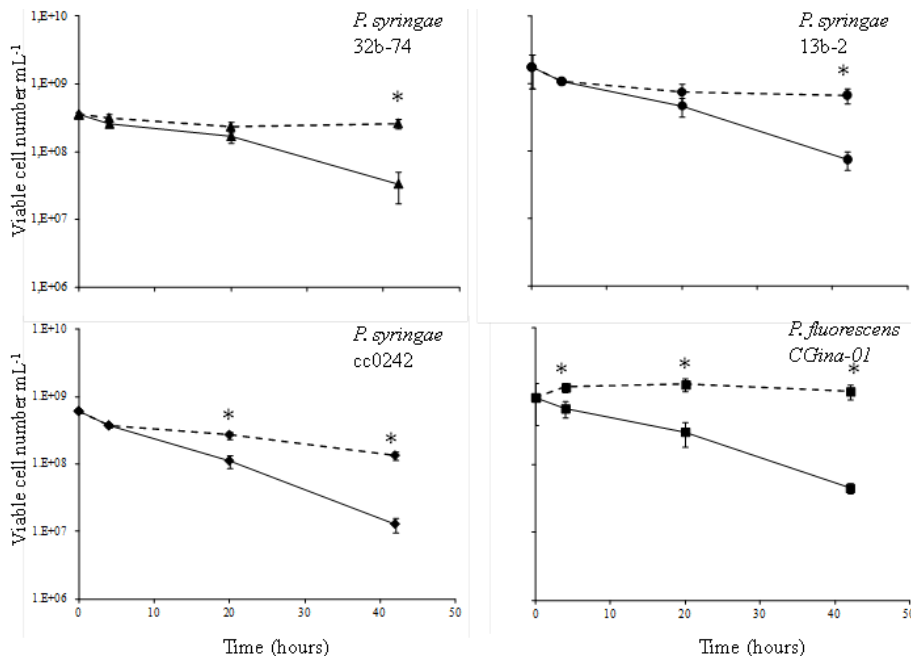
Fig. 4. , Viable cell number (CFU) of the Pseudomonas strains after UV exposure (solid line) or darkness (dotted line). Symbols are as in Fig. 1. At each time point, values associated with an asterisk are significantly different ( p < 0.05 ) based on Tukey's test. Errors bars are standard errors ( n = 4 ).
