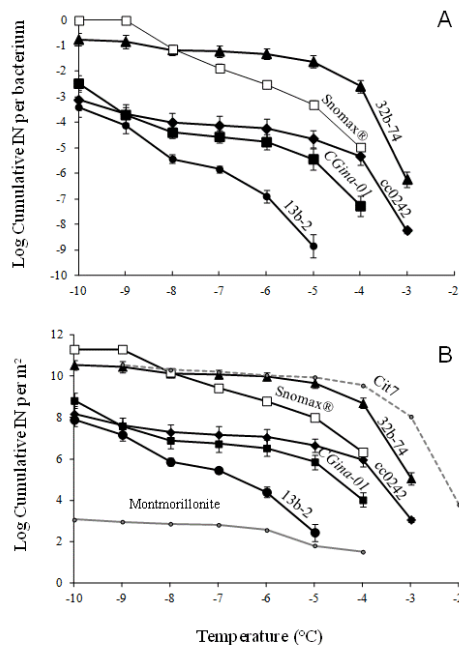
Fig. 1. Ice nucleation spectra of Pseudomonas strains in distilled water: P. syringae 32b-74 (filled triangle) and 13b-2 (filled circle), P. syringae cc0242 (filled diamond), P. fluorescens CGina-01 (filled box), the commercial Snomax ® (open box), P. syringae Cit7 (grey dotted line; data from Orser et al., 1985) and Montmorillonite (grey solid line, data from Mortazavi et al., 2008). (A) log (cumulative IN per bacterium); (B) log (cumulative IN per m 2 ). Errors bars indicate standard errors ( n = 6 ).
