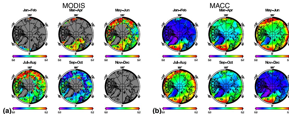
Fig. 4. Maps of average AOD in different periods of the year. Monthly means are calculated in the period 2003 to 2006, common to all datasets. Panels: (a) MODIS Terra, (b) MACC. Grey areas indicate missing data.
