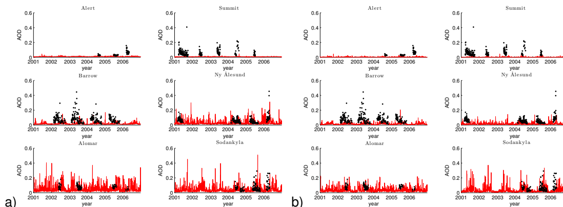
Fig. 2. Time series of daily mean of AOD (550 nm) at the indicated Arctic sites. The black symbols are the observations and the continuous lines the model results: panel (a) ECHAM5-HAM (EIPCC emissions) results; panel (b) results obtained using TM5. The station data for AOD were measured at 500 nm and interpolated to 550 nm using the observed Ångström parameters.
