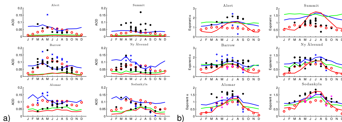
Fig. 3. Observed and modeled seasonal climatologies of AOD at 550 nm (panel (a) ) and of the Ångström parameter (panel (b) ) at the measurement sites. Observations are shown as black dots (to illustrate interannual variability, we report the individual values for each year). Model results are represented by the continuous lines: ECHAM5-HAM (EIPCC emissions) (green), ECHAM5-HAM with the correction suggested by Bourgeois and Bey (2011) (blue), TM5 (red). MACC data are shown for comparison (red circles) together with MODIS-Aqua (+) and MODIS-Terra (x) observations. For the Ångström parameter both the land (magenta) and the ocean (blue) MODIS products are reported. All model data and MODIS-Terra observations (where available) are averaged over the years 2001–2006. MODIS-Aqua observations are averaged over the years 2002–2007 and MACC data are averaged over the years 2003–2006. The station data for AOD were measured at 500 nm and interpolated to 550 nm using the observed Ångström parameters.
