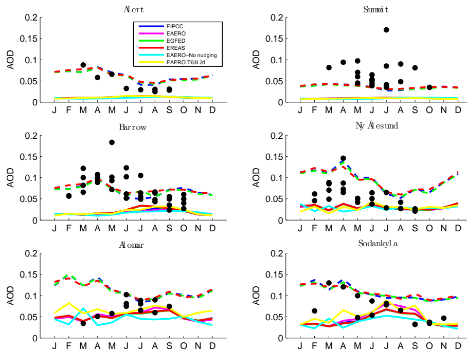
Fig. 7. Comparison of AOD modeled with ECHAM-HAM for different emission databases, averaged over the years 2001–2006. Emissions used are EAERO (continuous magenta line), EIPCC (blue), EGFED (green), EREAS (red). A simulation with the EAERO emissions and without nudging is reported in cyan. The same emissions, using also the Bourgeois and Bey (2011) parametrization are dashed. We also report one simulation (ECHAM-HAM, EAERO) at a higher resolution of T63L31 (in yellow- averaged over the years 2001–2003). Ground-based station observations are reported with black dots as in Fig. 3.
