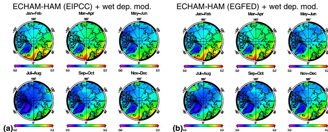
Fig. 6. Maps of average AOD in different periods of the year. Monthly means are calculated in the period 2003 to 2006, common to all datasets. Panels: (a) ECHAM-HAM (EIPCC) with the Bourgeois and Bey (2011) modification. (b) ECHAM-HAM (EGFED) with the Bourgeois and Bey (2011) modification.
