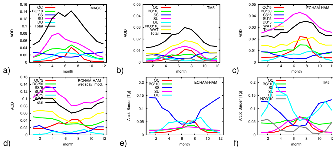
Fig. 8. (a) Averages over the Arctic (north of 60^\circ\text{N} ) of the contribution to total AOD of different compounds for the MACC reanalysis (these are ambient aerosol contributions, i.e. including water); (b) average AOD of different compounds in the TM5 model (ambient aerosols). (c) the same for the ECHAM-HAM (EIPCC) simulation (a direct comparison is not possible since diagnosed aerosol water is treated as a separate compound in HAM diagnostics and the dry aerosol contributions are shown); (d) the same as (c) for the ECHAM-HAM (EIPCC) simulation with the (Bourgeois and Bey, 2011) wet scavenging modification. (e) average total burdens (in Tg) over the Arctic for the ECHAM-HAM (EIPCC) simulation. (f) average total burdens (in Tg) over the Arctic for the TM5 simulation. A factor 1.4 has been used to convert particulate organic matter to organic carbon for TM5. MACC data are averaged over the years 2003–2006. TM5 and ECHAM-HAM data are averaged over the years 2001–2006. AOD and burdens of black carbon have been multiplied by 10 for clarity in all panels. An additional factor of 5 has been applied to show the seasonalities of dry AOD contributions of individual compounds for ECHAM-HAM in panels (c) and (d).
