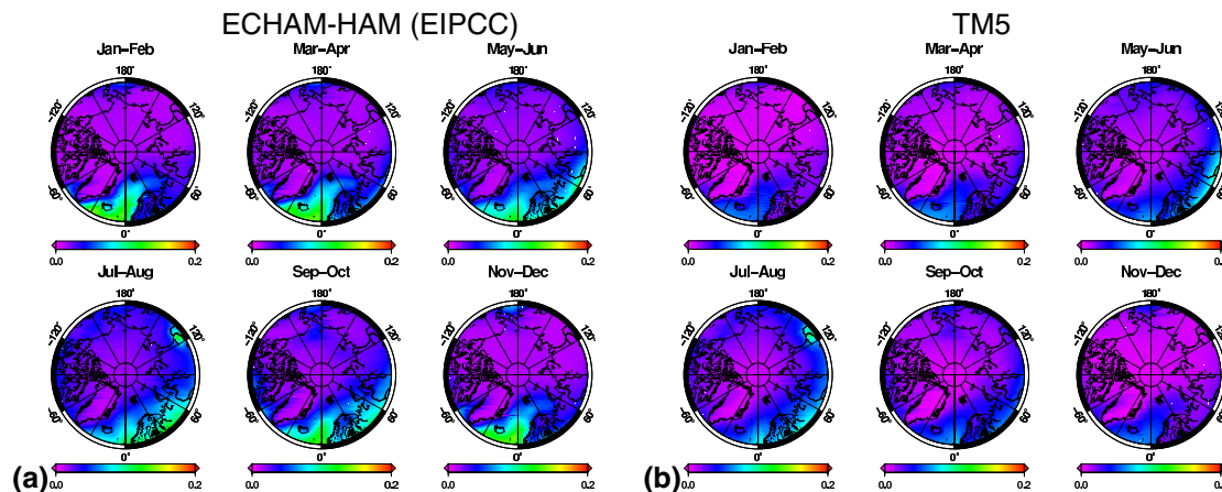
Fig. 5. Maps of average AOD in different periods of the year. Monthly means are calculated in the period 2003 to 2006, common to all datasets. Panels: (a) ECHAM-HAM (EIPCC emissions), (b) TM5.
