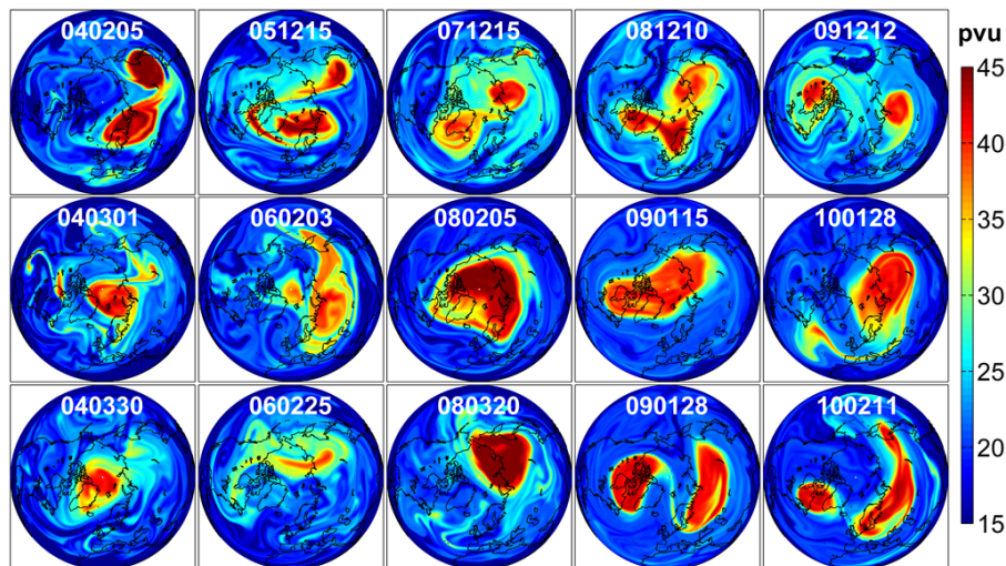
Fig. 5. Same as Fig. 4, but for 475 K.
