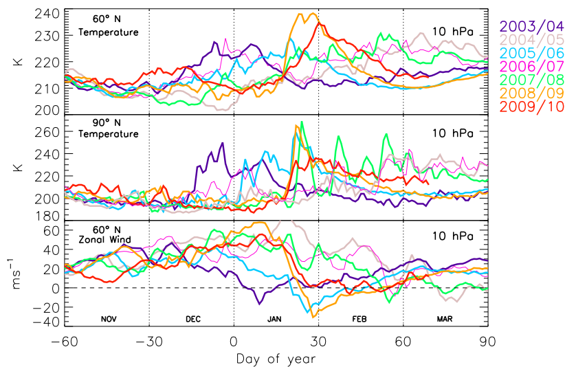
Fig. 1. Evolution of the zonally averaged temperature and zonal wind in the Arctic winters 2003/04–2009/10. The dashed horizontal line represents 0 \text{ ms}^{-1} and the dotted vertical lines separate each month.
