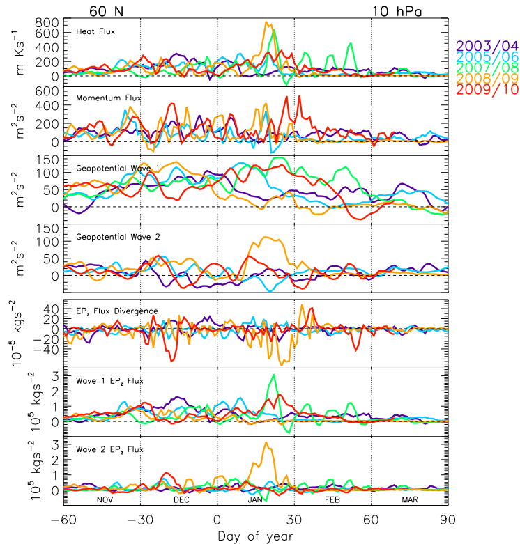
Fig. 3. Temporal evolution of various derived quantities for selected Arctic winters at 10 hPa and 60°N, where the MW criterion is considered. All derived quantities are zonally averaged. The quantity zero is marked with dashed horizontal lines. Since the warming was not severe in 2007/08, some entities are not shown for this winter for clarity reasons. The dotted vertical lines represent the month boundaries.
