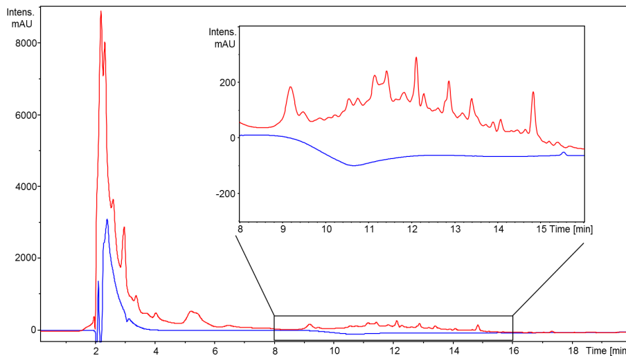
Figure 5. Temporal evolution of relatively apolar products in a Gly/AS mixture (1.5 M Gly, 3 M AS). The blue chromatogram was recorded immediately after mixing and the red chromatogram 116.05 h after mixing (sum of absorbances at wavelengths between 350 and 400 nm).
