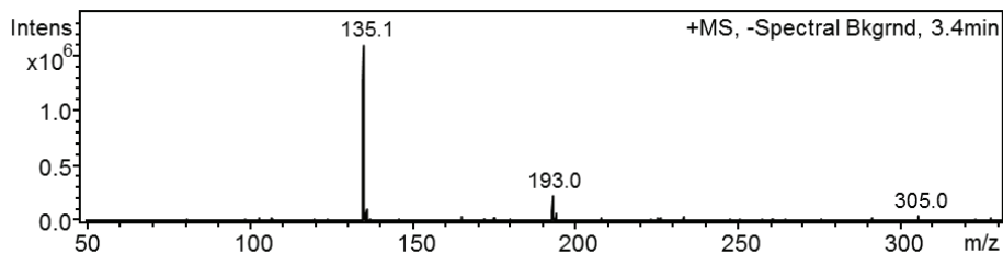
Figure 3. Typical MS of 0.01 M Gly in 3 M AS at 3.4 min retention time.
