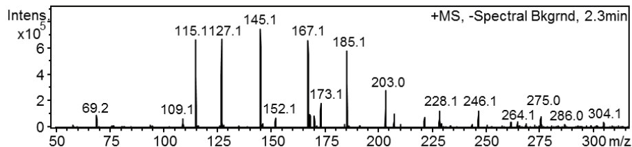
Figure 2. Typical MS of 1.5 M Gly in 3 M AS at 2.3 min retention time.
