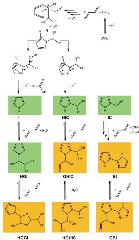
Figure 1. Proposed reaction pathways for imidazole formation in the glyoxal/ammonium sulfate system are shown. Green colored compounds were previously described in literature (Yu et al., 2011; Galloway et al., 2009); orange colored compounds were identified in this work.
