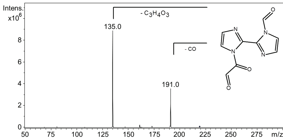
Figure 6. MS/MS of a compound with m/z 219 eluting at 10.6 min retention time. Proposed structure and neutral losses are shown.
