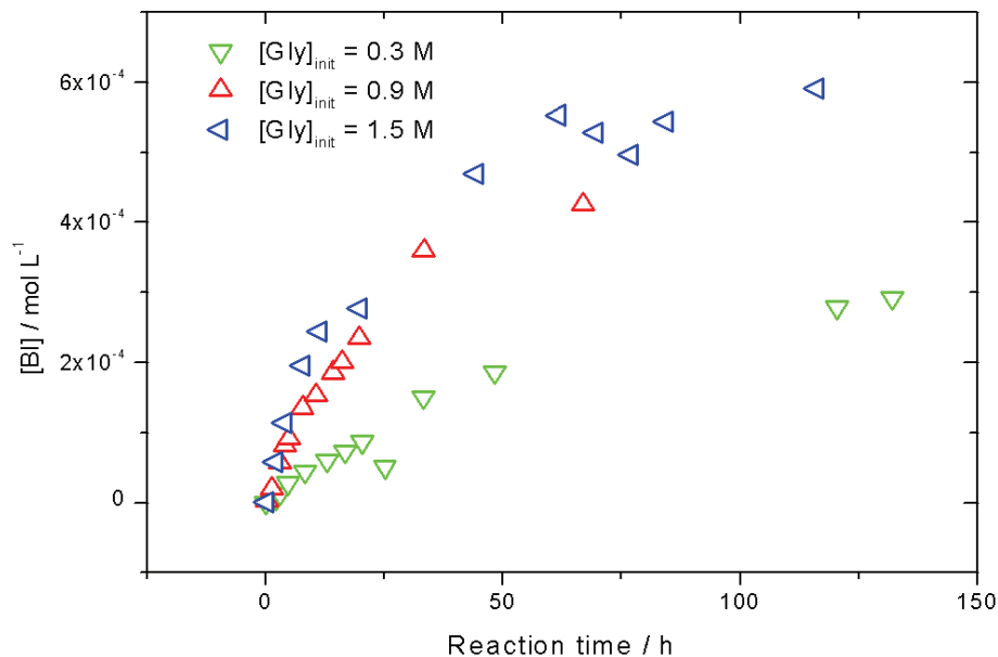
Figure 4. Concentration of BI in 3M AS at different initial glyoxal concentrations is shown as a function of reaction time. Concentrations were determined via 280 nm absorption band at 3.5 min retention time using HPLC-DAD.
