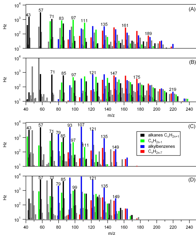
Fig. 5. Mass spectrum of #2 diesel fuel at 120 Td (A) and 80 Td (B) and gasoline at 120 Td (C) and 80 Td (D) . Ion signal has been color coded to assign ions to common fragmentation patterns that identify common organic compound classes. For diesel the ion signal is more evenly distributed across the 4 ion fragmentation groups than gasoline, while for the gasoline most of the ion signal was observed in the alkylbenzene group since the PTR-MS is insensitive to most of the light alkanes found in gasoline.
