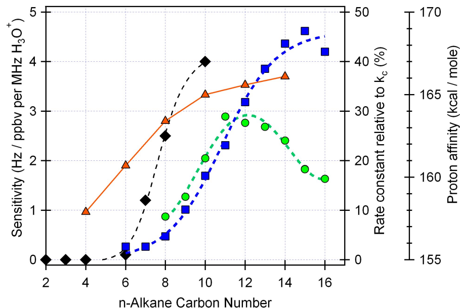
Fig. 4. Alkane sensitivity (left axis) for 120Td (blue squares) and 80Td (green circles) compared to measured \text{H}_3\text{O}^+ + alkane rate coefficients (black diamonds) by Arnold et al. (1998) expressed as a percentage of collision rate limit (right axis). Also shown is the proton affinity (red triangles) determined by Hunter and East (2002).
