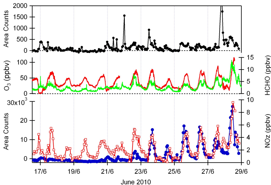
Fig. 11. Time series of m/z 161 area counts (upper panel), ozone (red trace) and formaldehyde (green trace) mixing ratios are shown in the middle panel, m/z 143 area counts (blue circles) and \text{NO}_z (red squares) are shown in the lower panel.
