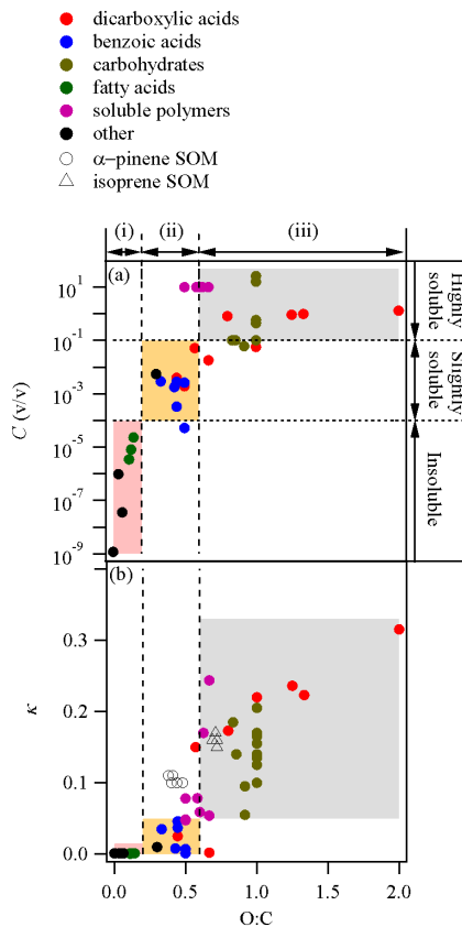
Fig. 3. Relationship of O : C ratio to C (a) and \kappa (b). The colored areas in the panels highlight clustering among insoluble, slightly soluble, and highly soluble compounds. The list of compounds is available in Supplement.
