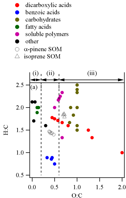
Fig. A2. Relationships between O : C and H : C ratios of pure compounds and SOM (van Krevelen diagram). The regions (i)–(iii) indicates (i) insoluble, (ii) slightly soluble, and (iii) highly soluble regimes, respectively (see the main text for detail).
