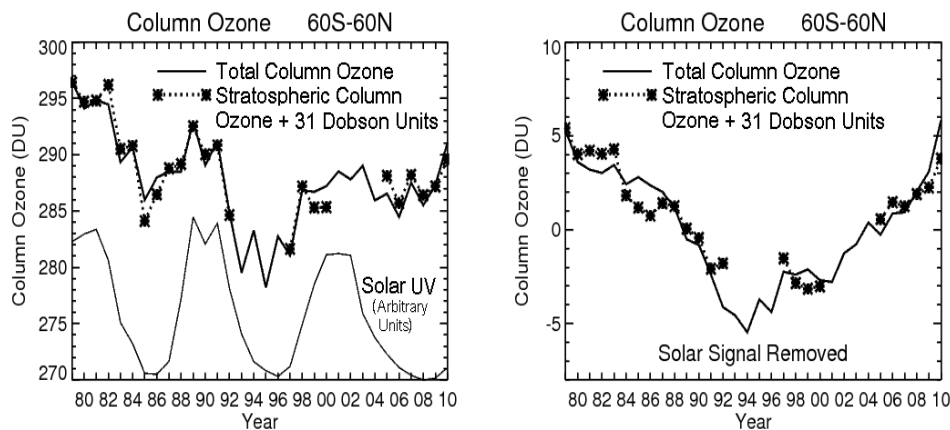
Fig. 16. (Left) Annual mean time series of TOMS/SBUV/OMI merged total column ozone (thick solid curve along top), TOMS+OMI CCD measurements of stratospheric column ozone (thick dotted curve along top), and solar F10.7 cm radio flux (thin solid curve along bottom) which has been rescaled for plotting. Stratospheric column ozone has had 31 Dobson Units added for visualization in plotting with total column ozone. Both ozone time series represent area-weighted measurements lying between latitudes 60° S and 60° N. (Right) Similar to ozone plotted in the left panel except that time averages have been removed and the 11-yr solar-cycle signals in the two ozone time series have been extracted by linear regression. The regression model used to remove 11-yr solar cycle variability in the two ozone time series is ( t is year index): \text{Ozone}(t) = C \cdot \text{Solar}(t) + \varepsilon(t) where C and is a constant, \text{Solar} is solar F10.7 cm annual mean time series (with time average removed) and \varepsilon = model residual error. (The two derived residual series \varepsilon(t) are plotted in the right panel.) A 3-yr running average was applied to both time series in the right panel for smoothing.
