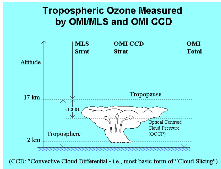
Fig. 1. Schematic illustration of the OMI/MLS tropospheric ozone residual method (OMI total column ozone minus MLS stratospheric column ozone) and the convective-cloud differential (CCD) residual method (OMI total column ozone minus OMI above-cloud column ozone).
