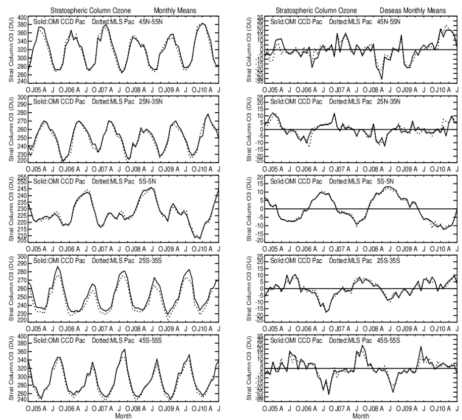
Fig. 10. (Left panels) Monthly averaged Pacific mean measurements of CCD SCO from OMI (solid curve) and MLS SCO (dotted curve) averaged over five indicated 10° latitude bands. The Pacific mean represents data averaged over the combined eastern and western Pacific (i.e., longitude range 120° W to 120° E about the dateline). All measurements are in Dobson Units. (Right panels) Same as left panels but with the data deseasonalized.
