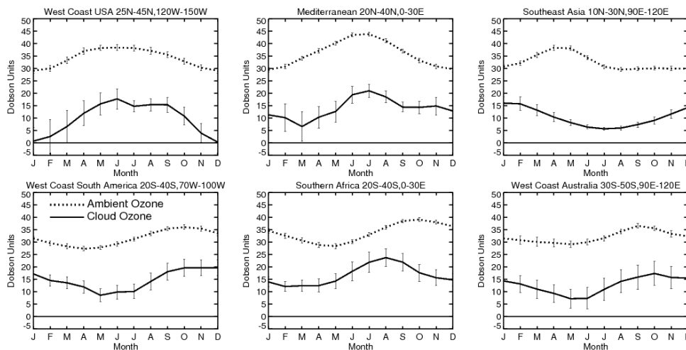
Fig. 7. Similar to Figs. 5 and 6 but instead for six broad regions of the globe where measured CCD cloud ozone is large with peak abundances of \sim 15 – 20 DU. These six regions are from upper left to lower right (compare these regions with Fig. 4): West Coast of the USA, Mediterranean, Southeast Asia, West Coast of South America, Southern Africa, and West Coast of Australia.
