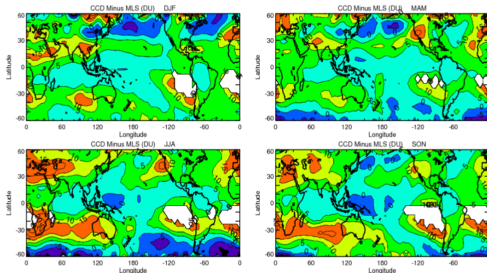
Fig. 4. Three-month seasonal averages (December–February, March–May, June–August, and September–November) of CCD above-cloud column ozone minus MLS stratospheric column ozone over the time record 2004–2010. Contour numbers represent Dobson Units. The colors violet/blue to orange represent negative to positive values, respectively. We denote these measurements in this figure as “cloud ozone”, the amount of column ozone lying between the tropopause and cloud OCCP under conditions of deep convection. White regions denote areas where there is insufficient number of deep convective clouds for the CCD method.
