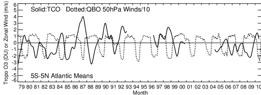
Fig. 14. Tropospheric column ozone from the CCD method in Dobson Units (solid curve) plotted versus 50 hPa zonal winds from Singapore ( 1^{\circ} N, 104^{\circ} E) in units \text{m s}^{-1} but divided by 10 for scaling (dotted curve). The ozone time series was averaged over the equatorial Atlantic region ( 5^{\circ} S– 5^{\circ} N, 60^{\circ} W– 60^{\circ} E). The ozone time series was deseasonalized and detrended, and then smoothed using a recursive low-pass digital filter with one-half filter response at 12-month period (filter response of about 0.8–0.9 for 24–36 month QBO time periods).
