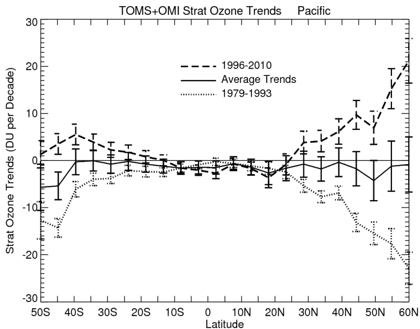
Fig. 15. Trends (units \text{DU decade}^{-1} ) of CCD stratospheric column ozone for the 1979–1993 beginning 15-yr record (bottom dotted curve) and 1996–2010 ending 15-yr record (top dashed curve). As comparison, trends for these two 15-yr records are averaged together (middle solid curve). Trends were derived for the two 15-yr records using a linear multivariate regression model (see text). All data were averaged over the Pacific ( 120^\circ \text{W} to 120^\circ \text{E} about dateline) within 5^\circ latitude bands. Vertical bars indicate \pm 2\sigma annual mean trend uncertainties calculated from the regression model. The trend uncertainty bars include an additional 2 DU ( 2\sigma ) long-term inter-instrument calibration/drift uncertainty. Values of 2\sigma for the averaged trends were derived by taking the square root of the sum of the variances for the two 15-yr record variances \times 2 .
