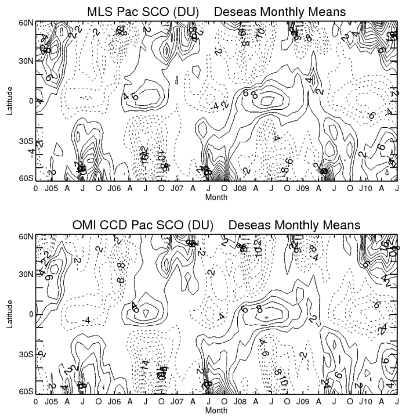
Fig. 9. Contour diagrams of the same stratospheric column ozone (in Dobson Units) plotted in Fig. 8, but instead with all of the data deseasonalized.
