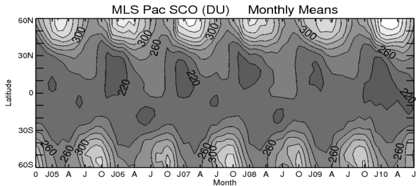
Fig. 8. Latitude versus month contour diagrams of monthly mean stratospheric column ozone (in Dobson Units) averaged over the Pacific (120° W–120° E) from OMI CCD (top) and MLS (bottom). Dark to light shading designates smaller to higher column amounts, respectively. The contour values for both diagrams begin at 200 Dobson units and increment by 20 Dobson Units.
