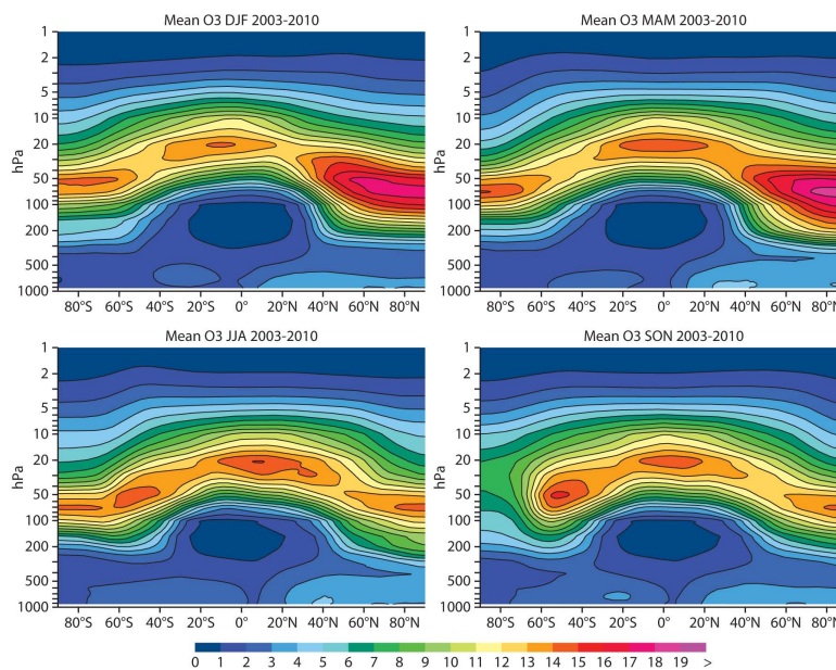
Fig. 12. Seasonal mean zonal average ozone cross sections from the MACC reanalysis in mPa for DJF (top left), MAM (top right), JJA (bottom left) and SON (bottom right) averaged over the years 2003 to 2010. Red indicates higher values of the field, blue lower values.
