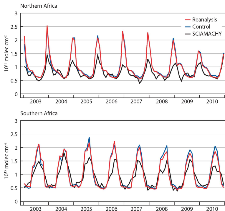
Fig. 27. Time series of monthly mean area averaged tropospheric NO 2 columns in 10 15 molec cm -2 from the MACC reanalysis (red), the control run (blue) and from IUP-SCIAMACHY data (black) for the period 2003 to 2010 for Northern Africa (top) and Southern Africa (bottom). Only land points were used in these calculations.
