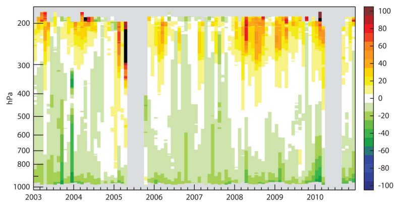
Fig. 8. Time series of monthly mean CO biases (MACC reanalysis minus MOZAIC) in % at Frankfurt airport (50.0° N, 8.6° E) for the period January 2003 to December 2010.
