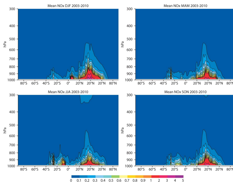
Fig. 28. Seasonal mean zonal average NO x cross sections from the MACC reanalysis in ppb for DJF (top left), MAM (top right), JJA (bottom left) and SON (bottom right) averaged over the years 2003 to 2010. Red indicates higher values of the field, blue lower values.
