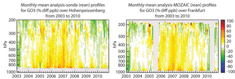
Fig. 19. Time series of monthly mean ozone biases (MACC reanalysis minus observations) with respect to ozone sondes at Hohenpeissenberg (left, 47.5° N, 11° E) and MOZAIK profiles at Frankfurt airport (right, 50.0° N, 8.6° E) for the period January 2003 to December 2010 in %.
