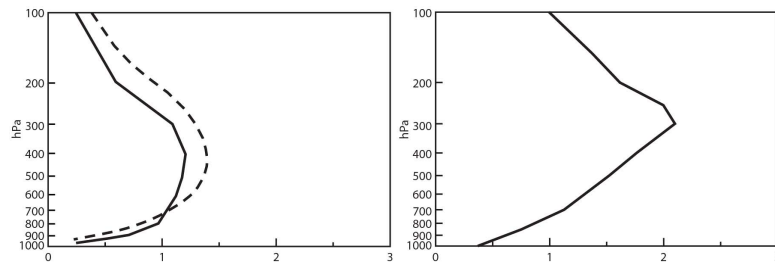
Fig. 1. Left panel: mean averaging kernels for MOPITT (solid) and IASI (dashed) day time total column CO retrievals for July 2009 averaged over a 5^\circ \times 25^\circ box over Europe ( 46\text{--}51^\circ\text{N} , 3\text{--}28^\circ\text{E} ). Right panel: global mean averaging kernels for tropospheric column \text{NO}_2 from SCIAMACHY averaged over the period June 2009 to May 2010.
