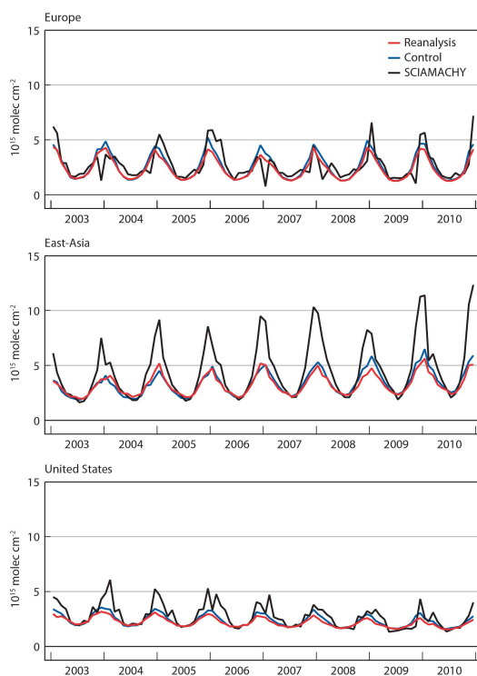
Fig. 26. Time series of monthly mean area averaged tropospheric NO 2 columns in 10^{15} molecules \text{cm}^{-2} from the MACC reanalysis (red), the control run (blue) and IUP-SCIAMACHY data (black) for the period 2003 to 2010 for Europe (top), East-Asia (middle) and the US (bottom). Only land points were used in these calculations.
