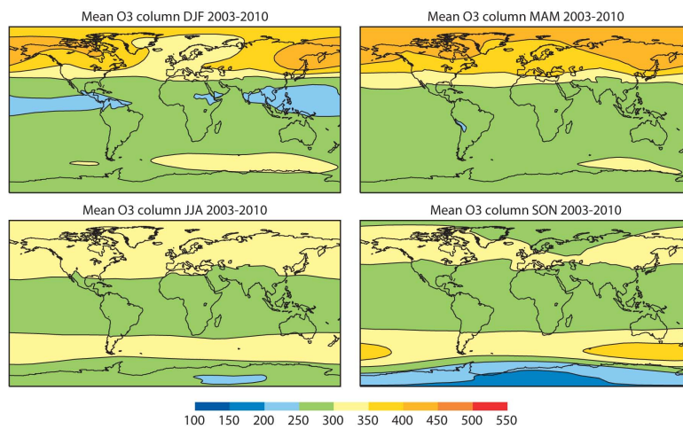
Fig. 11. Seasonal mean total column ozone field from the MACC reanalysis in DU for DJF (top left), MAM (top right), JJA (bottom left) and SON (bottom right) averaged over the years 2003 to 2010. Red indicates higher values of the field, blue lower values.
