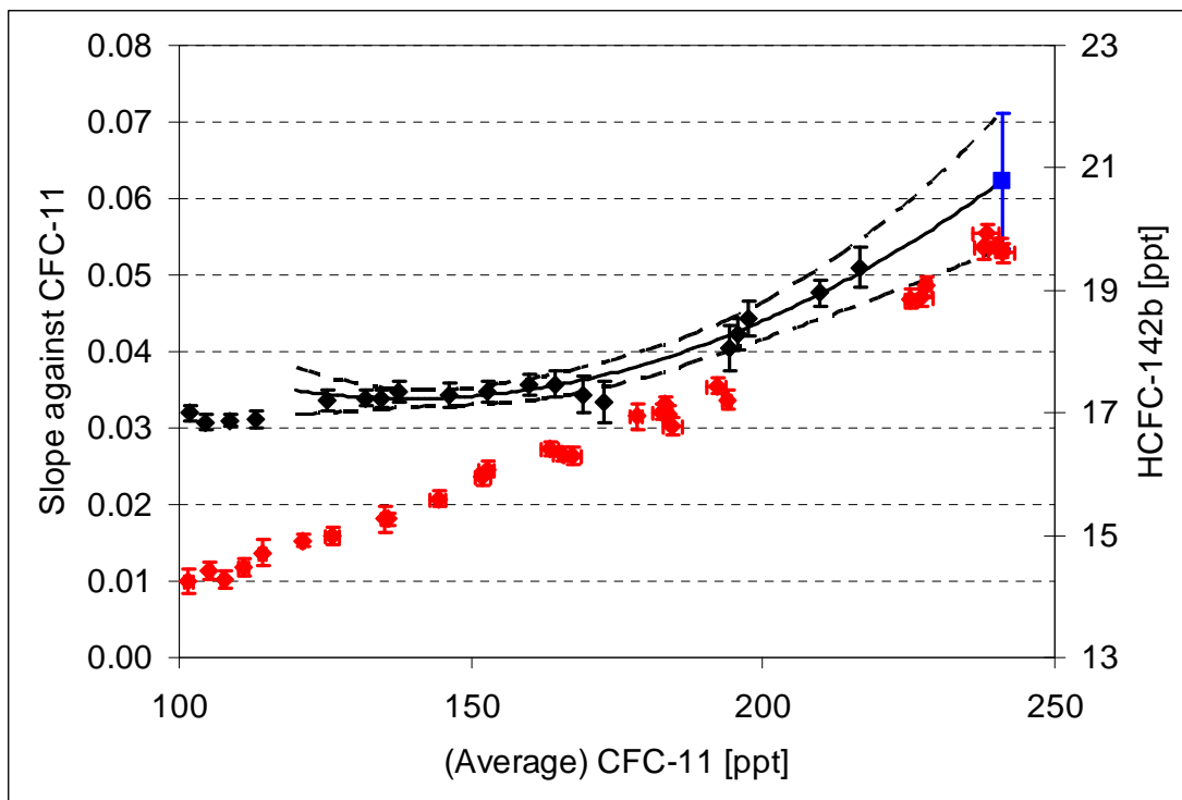
Figure S7. The same as in Figure S4 but for HCFC-142b.
