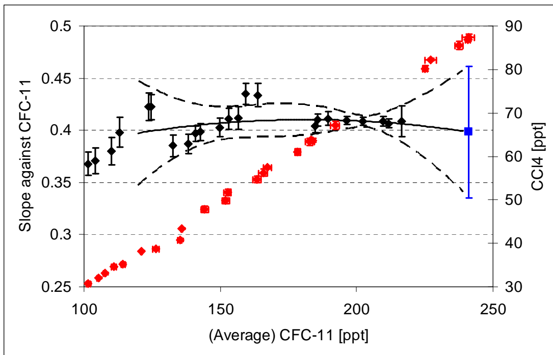
Figure S11. The same as in Figure S4 but for \text{CCl}_4 . 90 ppt windows of CFC-11 were used here to infer the individual slopes.
