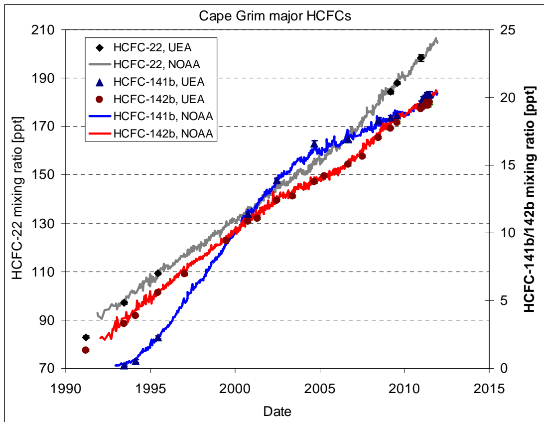
Figure S2. The same as in Figure S1 but for HCFC-141b, HCFC-142b, and HCFC-22.
