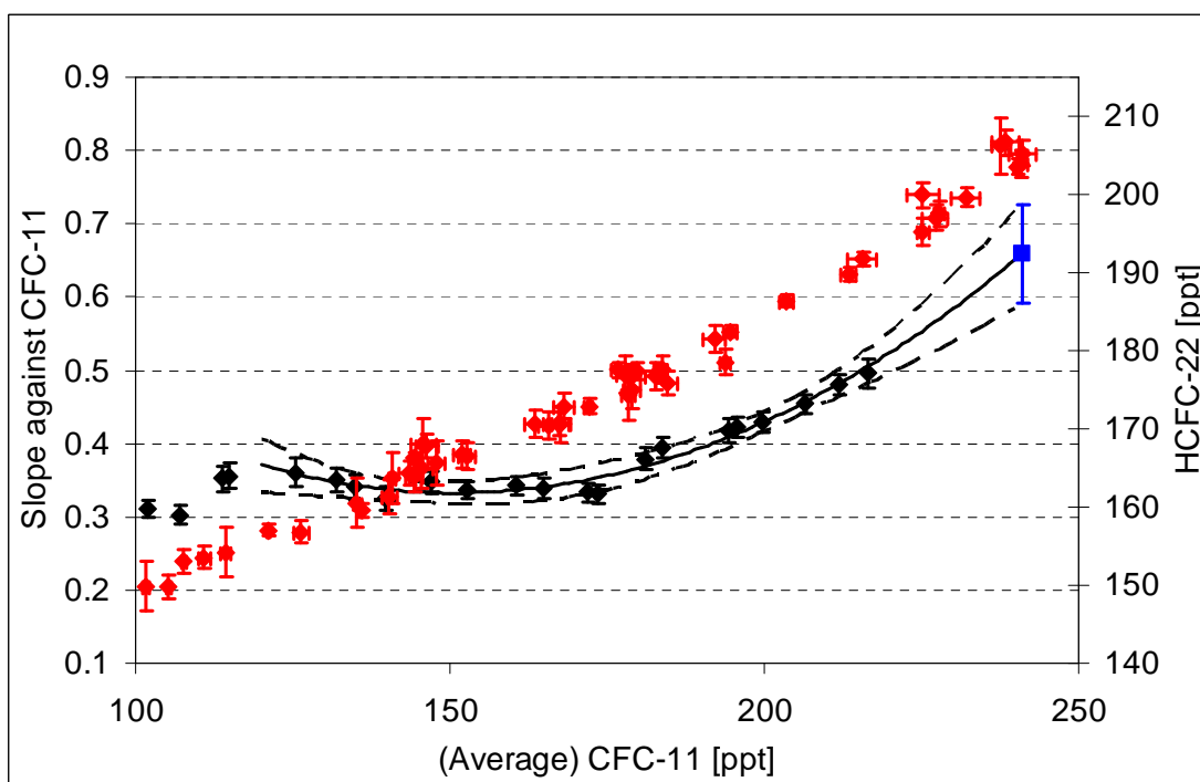
Figure S8. The same as in Figure S4 but for HCFC-22.
