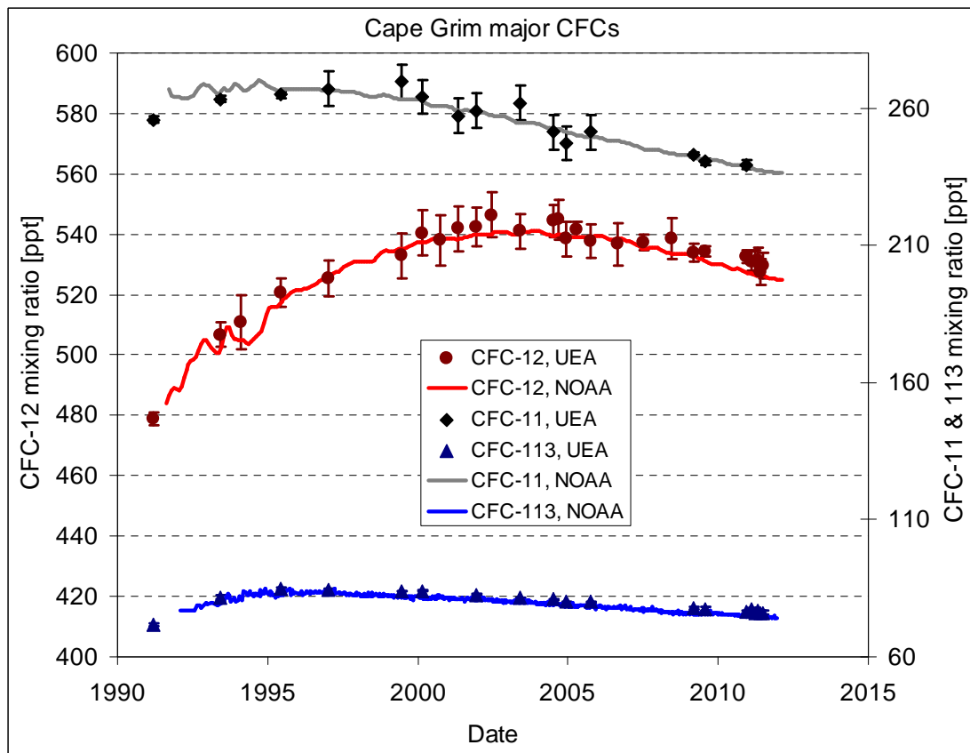
Figure S1. Comparison between mixing ratios of CFC-11, CFC-113, and CFC-12 as observed at the remote ground-based station at Cape Grim, Tasmania by the NOAA Global Monitoring division (lines) and UEA (symbols representing individual samples) between 1991 and 2011.
