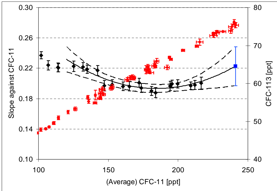
Figure S4. Evolution of correlation slopes of the mixing ratios of CFC-113 against the average mixing ratio of CFC-11. The black diamonds each represents the bivariate error-weighted slope of the correlation inferred over a range of \pm 35 ppt CFC-11. The error bars represent the 1 \sigma slope uncertainties. The black lines are the error-weighted quadratic polynomial fitted between 120 and 220 ppt and its respective uncertainty envelopes as inferred via the “bootstrap” method from Volk et al., 1997. Extrapolation of these polynomials to the tropopause at 241.0 ppt of CFC-11 results in the slopes and uncertainties (blue) given in Table S2. Note, that only data from the campaigns in late 2009 and early 2010 are combined for the calculation of these slopes. Displayed in red is the correlation of mixing ratios that was utilised to infer the slopes.
