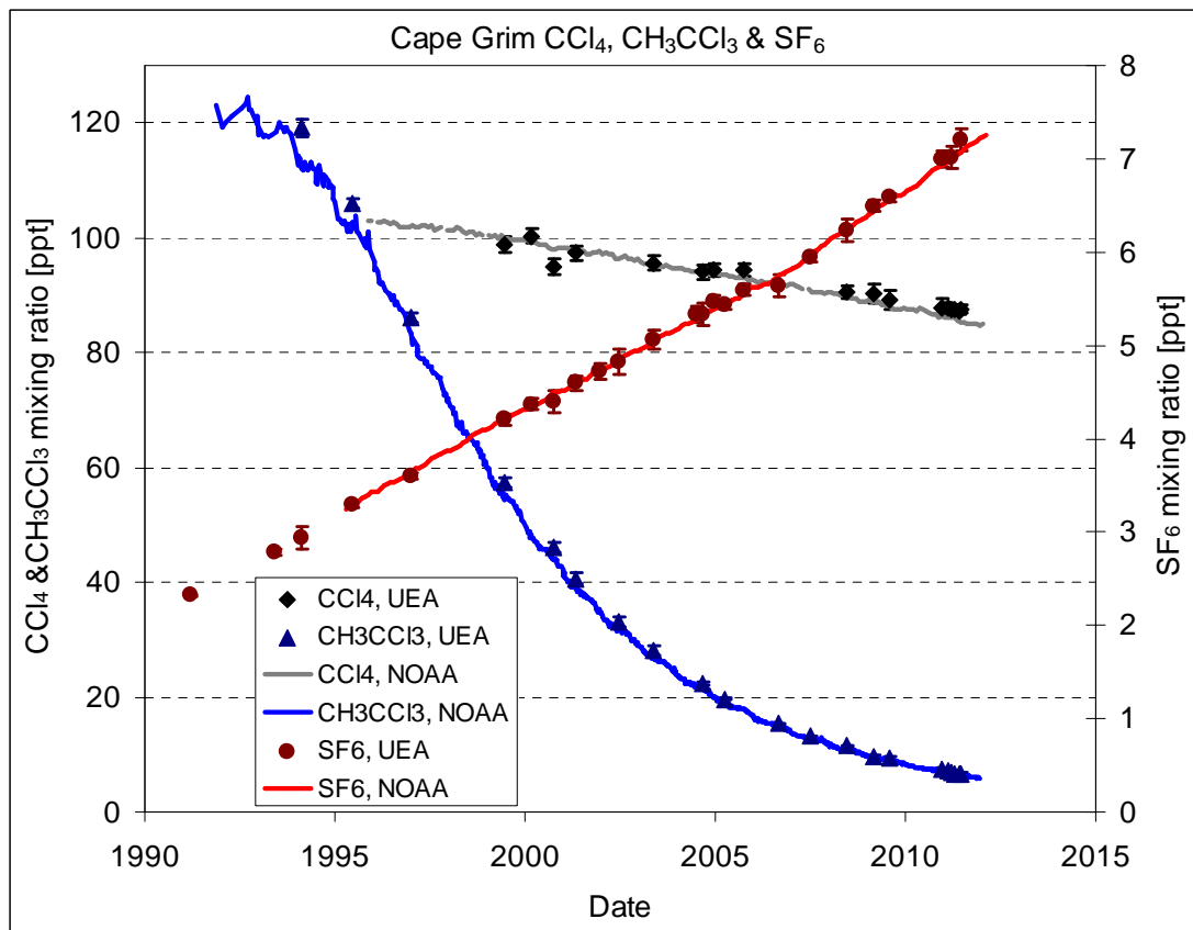
Figure S3. The same as in Figure S1 but for \text{CCl}_4 , \text{CH}_3\text{CCl}_3 , and \text{SF}_6 .
