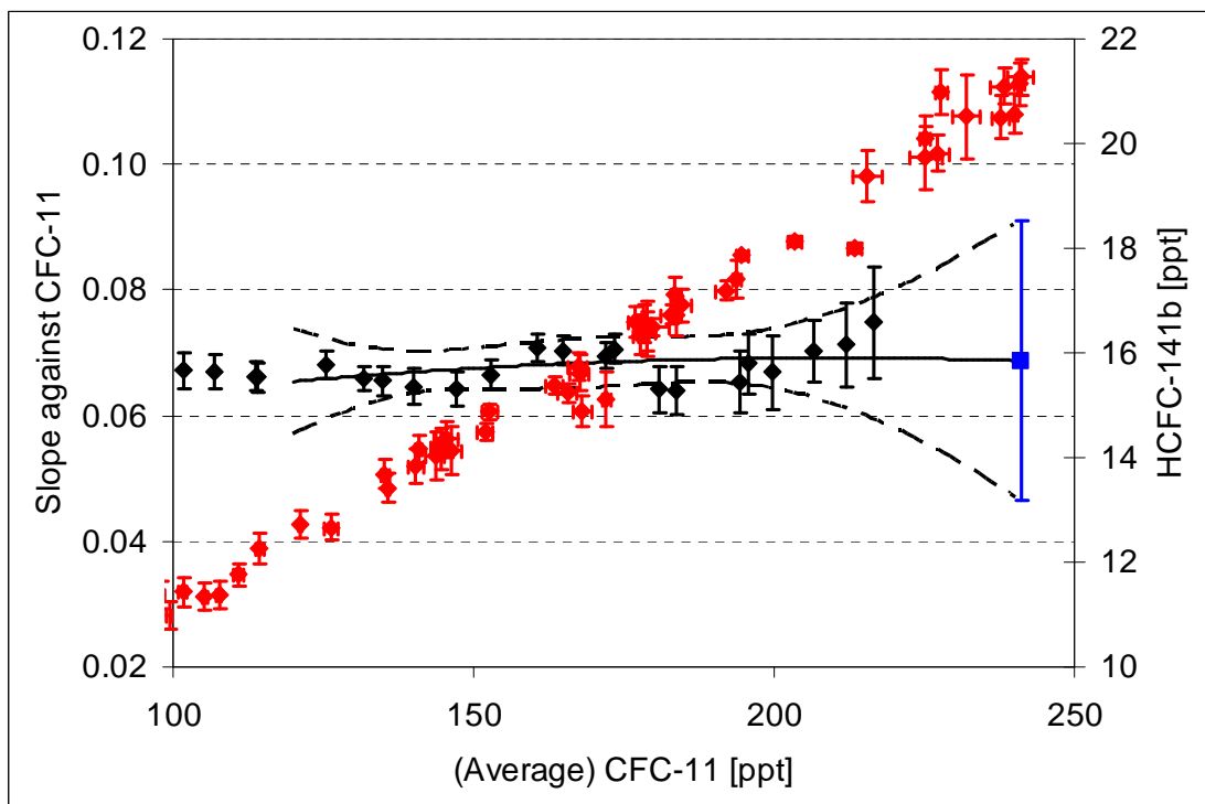
Figure S6. The same as in Figure S4 but for HCFC-141b.
