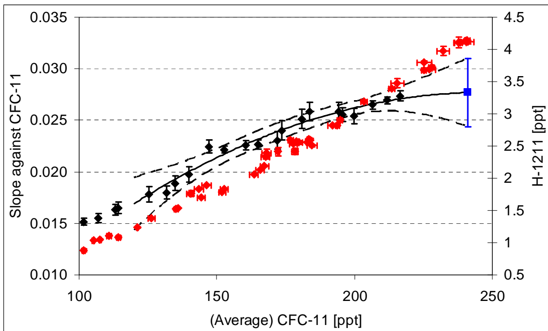
Figure S10. The same as in Figure S4 but for H-1211.
