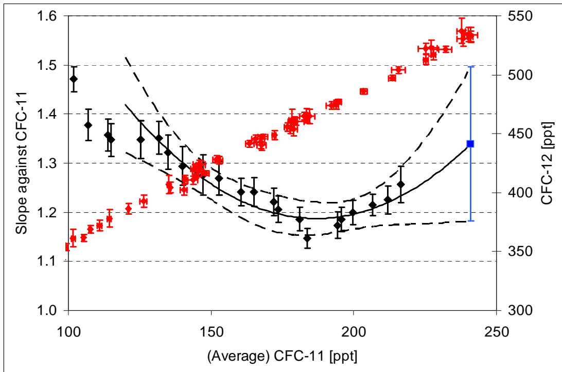
Figure S5. The same as in Figure S4 but for CFC-12.
