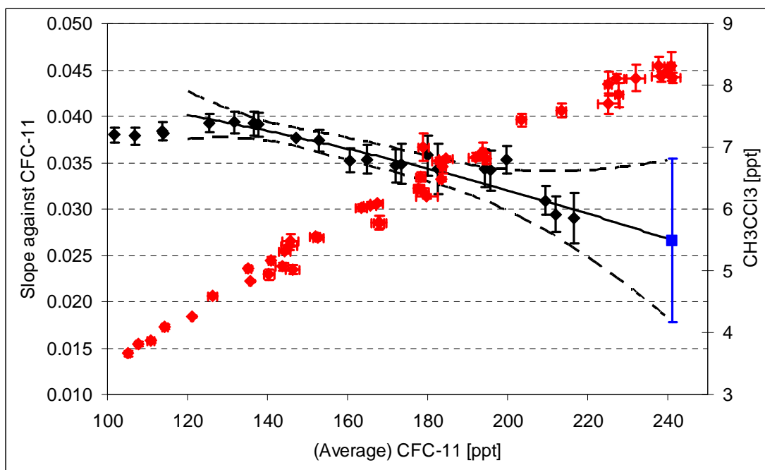
Figure S12. The same as in Figure S4 but for \text{CH}_3\text{CCl}_3 .
