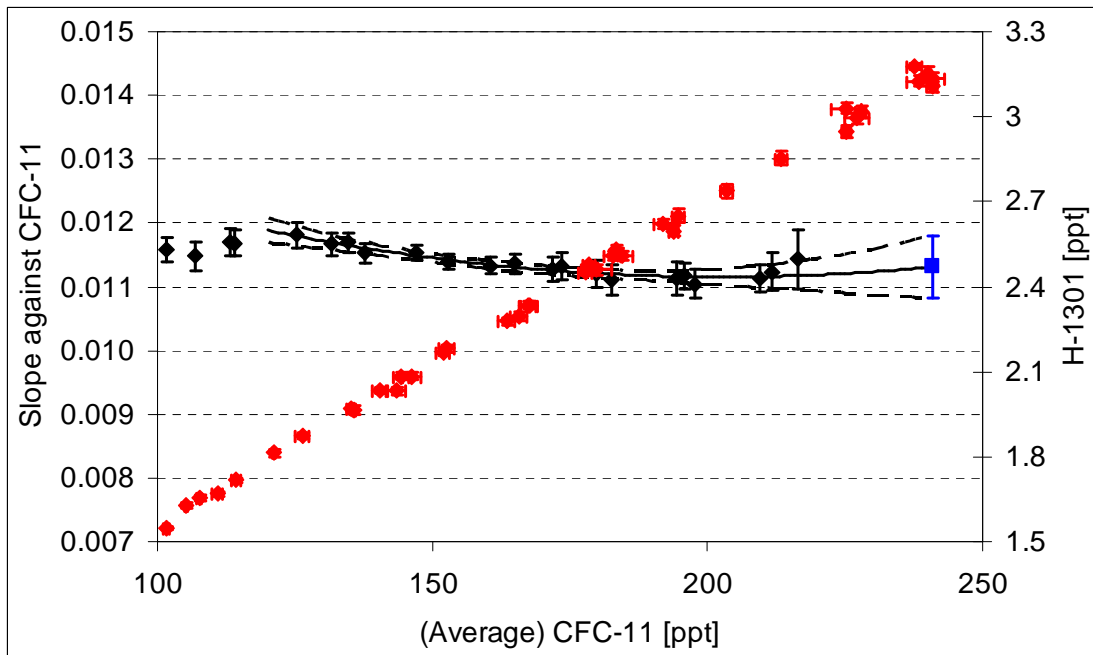
Figure S9. The same as in Figure S4 but for H-1301.
