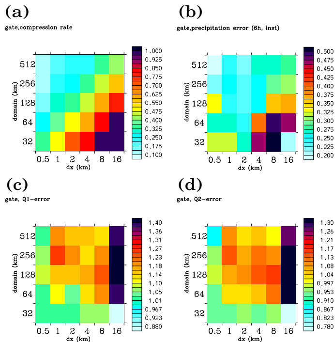
Fig. 11. Summary of stand-alone GATE case: (a) compression rate, along with the normalized RMS errors for (b) precipitation, (c) Q_1 , and (d) Q_2 shown as function of the horizontal resolution, \Delta x (horizontal axis) and the domain size, L (vertical axis). Errors are normalized against the ACCESS default cases.
