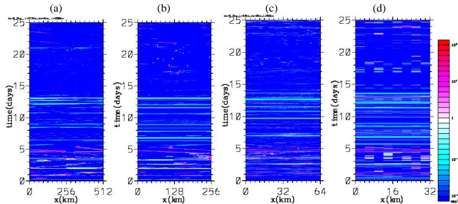
Fig. 18. The precipitation rate plotted as a function of the longitude and time for the cases for the stand-alone TWP-ICE cases: (a) \Delta x = 0.5 km, L = 512 km, (b) \Delta x = 4 km, L = 256 km, (c) \Delta x = 0.5 km, L = 64 km, and (d) \Delta x = 2 km, L = 32 km. The precipitation rates are shown in logarithmic scale for the range of 10^{-2} mm h ^{-1} to 10^2 mm h ^{-1} with the color ranging from blue (lowest) to red (highest) with a middle value shown in white.
