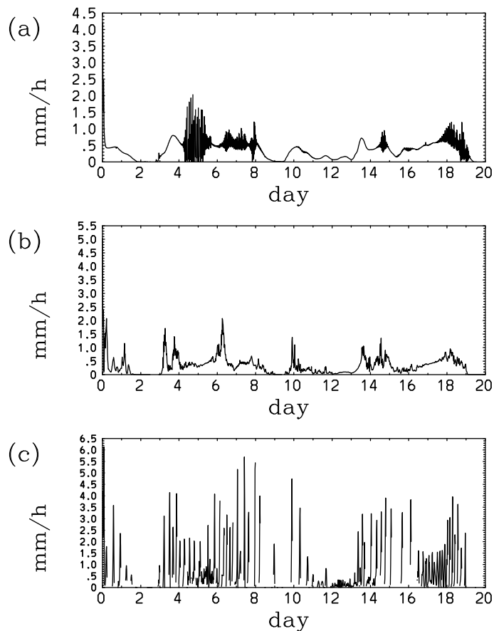
Fig. 24. The same as Fig. 12 but for the GATE case obtained by ACCESS simulations with NAM-SCA. From top to bottom: (a) \Delta x = 16 km, L = 32 km (best simulated precipitation); (b) \Delta x = 0.5 km, L = 512 km; (c) \Delta x = 8 km, L = 64 km (the worst case).
