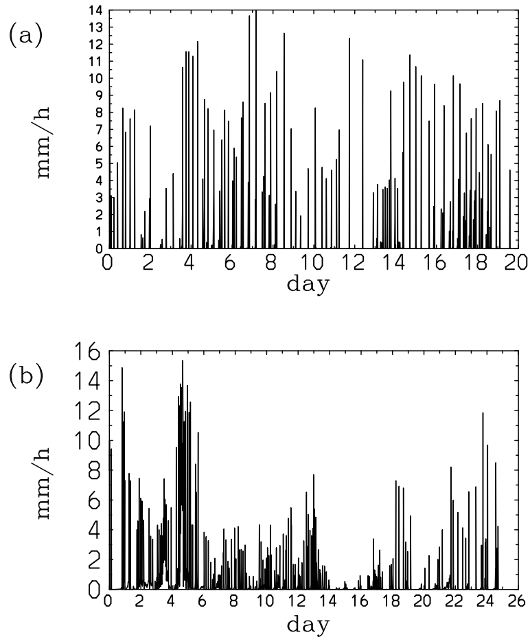
Fig. 6. The precipitation time series simulated by ACCESS-SCM with default physics for (a) the GATE Phase III and (b) the TWP-ICE periods. Here, data is plotted for every time step.
