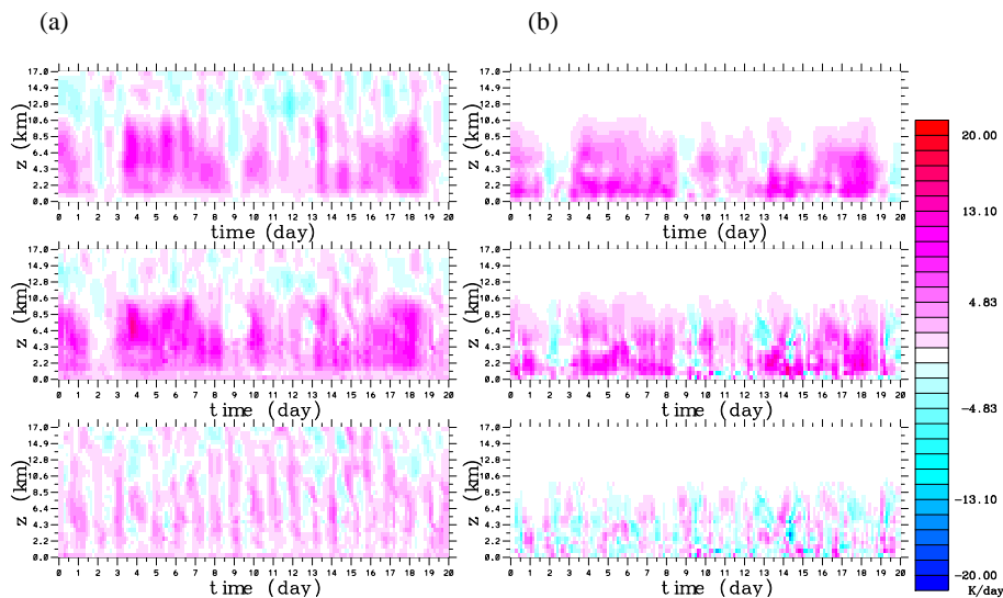
Fig. 7. The time-height section of apparent heat source, Q_1 (a), and apparent moisture sink, Q_2 (b) for the GATE Phase III period from (top) observations, (middle) as simulated by ECHAM-SCM default physics and (bottom) the difference.
