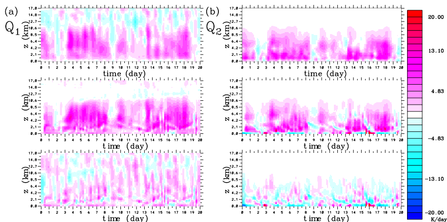
Fig. 13. Time-height section for (a) apparent heat source, Q_1 and apparent moisture sink, Q_2 during the GATE Phase III. From top to bottom: observation, the NAM-SCA stand-alone case with \Delta x = 16 km, L = 32 km, and the difference of the two.
