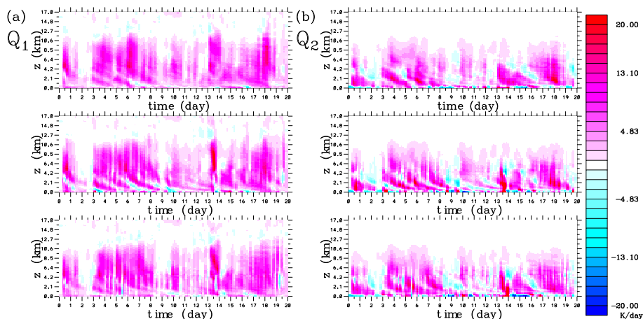
Fig. 14. Further examples of time-height sections for (a) apparent heat source, Q_1 and (b) apparent moisture sink, Q_2 during the GATE Phase III from NAM-SCA stand-alone simulations. The cases are from top to bottom: \Delta x = 0.5 km, L = 512 km (top), \Delta x = 1 km, L = 256 km (middle), \Delta x = 4 km, L = 256 km (bottom).
