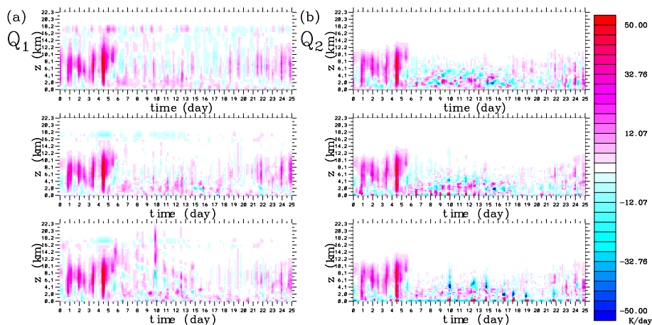
Fig. 19. The time-height section of the TWP-ICE case for the observation (top), the best simulation (middle), and one of the worst simulations (bottom) in term of the errors for (a: left) apparent heat source, Q_1 , and for (b: right) apparent moisture sink, Q_2 , respectively. The cases shown are: (a: middle) \Delta x = 2 km, L = 32 km, (a: bottom) \Delta x = 0.5 km, L = 64 km, (b: middle) \Delta x = 0.5 km, L = 64 km, (b: bottom) \Delta x = 16 km, L = 256 km.
