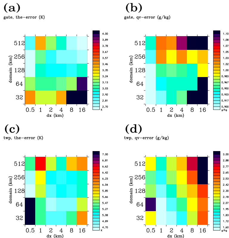
Fig. 27. Summary of the prediction errors in stand-alone (a, b) GATE and (c, d) TWP-ICE cases. RMS prediction errors for the potential temperature (K: a, c ) and the moisture mixing ratio ( \text{g kg}^{-1} : b, d ) are shown as functions of the resolution, \Delta x (horizontal axis) and the domain size, L (vertical axis).
