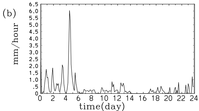
Fig. 5. The precipitation time series simulated by ECHAM-SCM with default physics for (a) the GATE Phase III and (b) the TWP-ICE periods. Plots use outputs averaged over every 1 h and 3 h, respectively.
