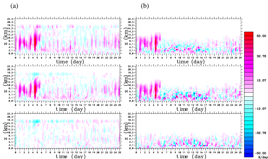
Fig. 9. The time-height section of apparent heat source, Q_1 (a), and apparent moisture sink, Q_2 (b) for the TWP-ICE period from (top) observations, (middle) as simulated by ECHAM-SCM default physics and (bottom) the difference.
