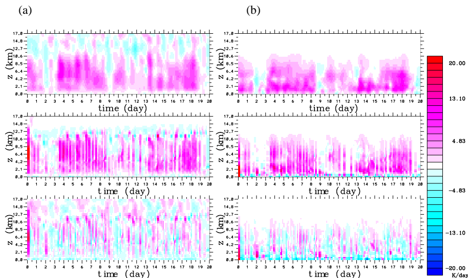
Fig. 8. The time-height section of apparent heat source, Q_1 (a), and apparent moisture sink, Q_2 (b) for the GATE Phase III period from (top) observations, (middle) as simulated by ACCESS-SCM default physics and (bottom) the difference.
