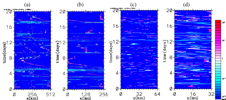
Fig. 21. The same as Fig. 15 but for NAM-SCA with ECHAM SCM for the GATE case: the precipitation rate from ECHAM GATE simulations with NAM-SCA plotted as a function of the longitude and time with: (a) \Delta x = 0.5 km and L = 512 km, (b) \Delta x = 4 km and L = 256 km, (c) \Delta x = 0.5 km and L = 64 km, and (d) \Delta x = 2 km and L = 32 km. The precipitation rates are shown in logarithmic scale for the range of 10^{-2} \text{mm h}^{-1} to 10^2 \text{mm h}^{-1} with the color ranging from blue (lowest) to red (highest) with a middle value shown in white.
