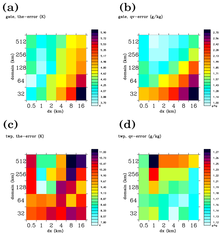
Fig. 28. Summary of the prediction errors under implementation into ECHAM for (a, b) GATE and (c, d) TWP-ICE cases. RMS prediction errors for the potential temperature (K: a, c ) and the moisture mixing ratio ( \text{g kg}^{-1} : b, d ) are shown as functions of the resolution, \Delta x (horizontal axis) and the domain size, L (vertical axis).
