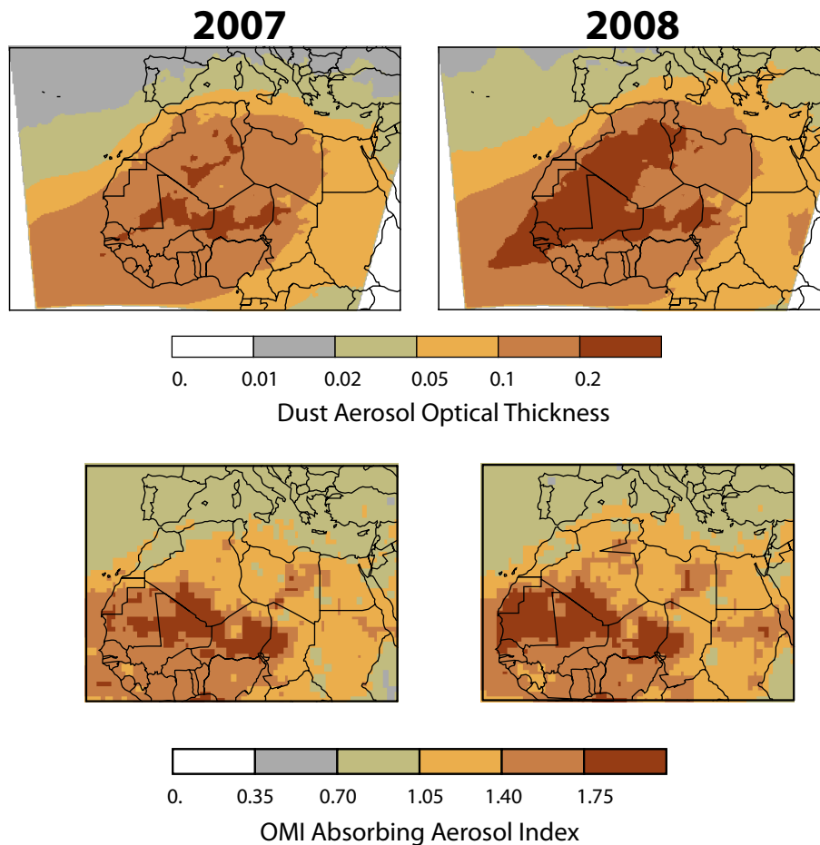
Fig. 4. Annual averaged dust optical thickness for the years 2007 (left panels) and 2008 (right panels) computed with COSMO-MUSCAT ( a, b ); annual averaged absorbing aerosol index from the OMI satellite instrument ( c, d ).
