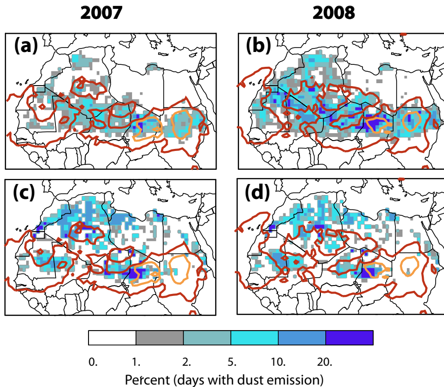
Fig. 3. Number of days per month with dust emission derived from the MSG SEVIRI IR dust index (a, b) and simulated with the COSMO-MUSCAT model (c, d); for year 2007 (left) and 2008 (right). The red and orange contours indicate areas where the occurrence of low level jets in the model is higher than 5 and 10 days per months, respectively.
