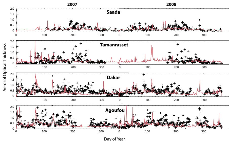
Fig. 5. Time series of daily modeled dust aerosol optical thickness (red line) and AOT measurements at 440 nm from AERONET at the stations Tamanrasset (22.8° N, 5.5° E), Saada (31.6° N, 8.2° W) Dakar (14.4° N, 17.0° W) and Agoufou (15.3° N; 1.5° W) (black plus signs) for 2007 and 2008. The black dots represent AOT measurements for Ångström parameters larger than 0.7 where dust AOT is not dominant.
