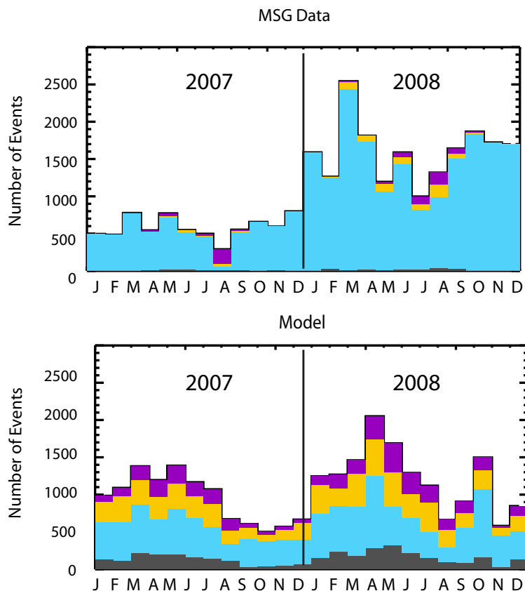
Fig. 1. Number of dust emission events in the Sahara for the years 2007 and 2008 derived from the MSG infrared dust index (top) and computed with the COSMO-MUSCAT model (bottom). The colors indicate the time of day when dust emission starts. Grey: 00:00–06:00 UTC, blue: 06:00–12:00 UTC, orange: 12:00–18:00 UTC, purple: 18:00–00:00 UTC.
