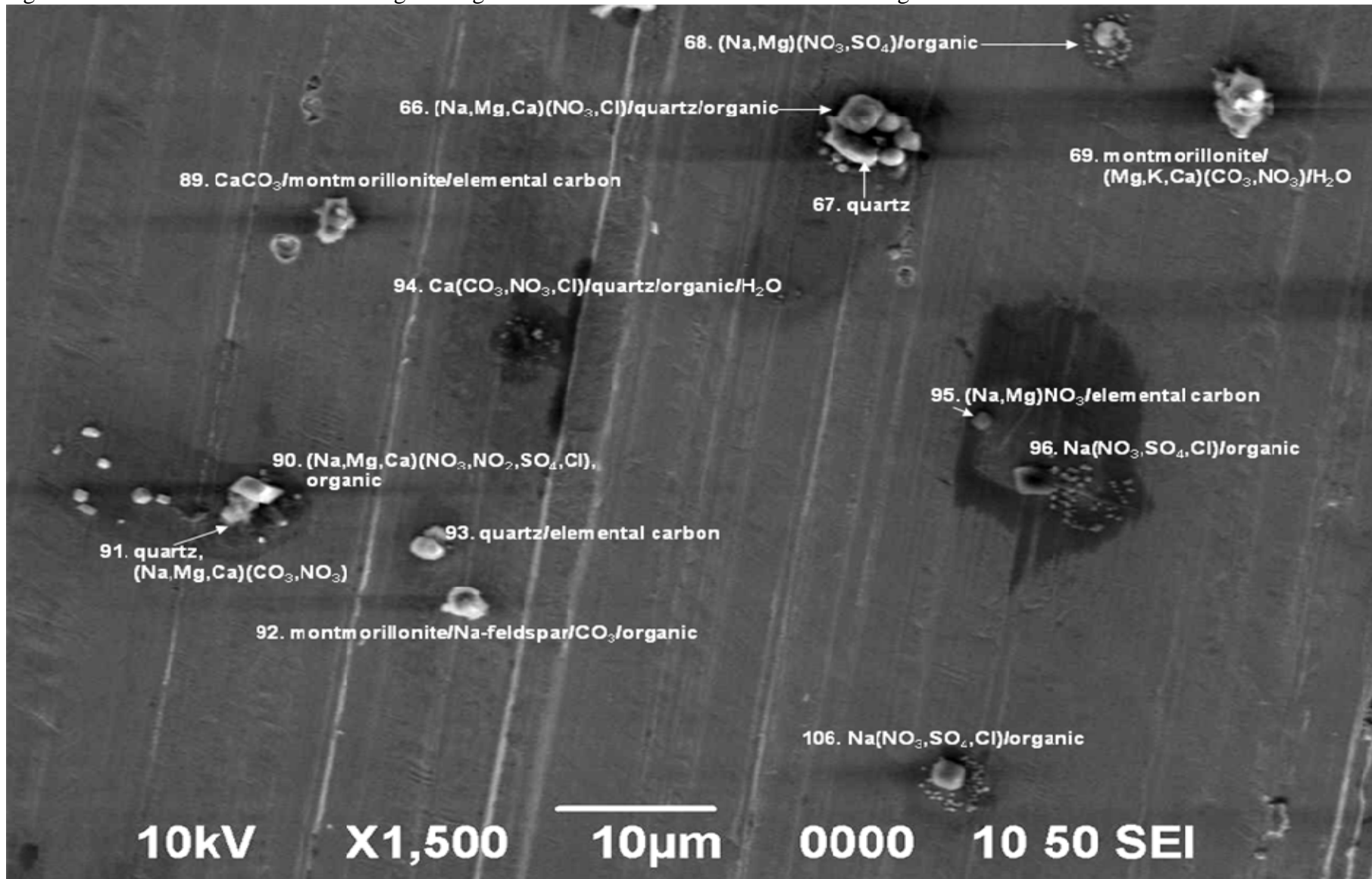
Figure S4. The fifth SEI obtained in a higher magnification than the overall SEI shown in Figure 1.
