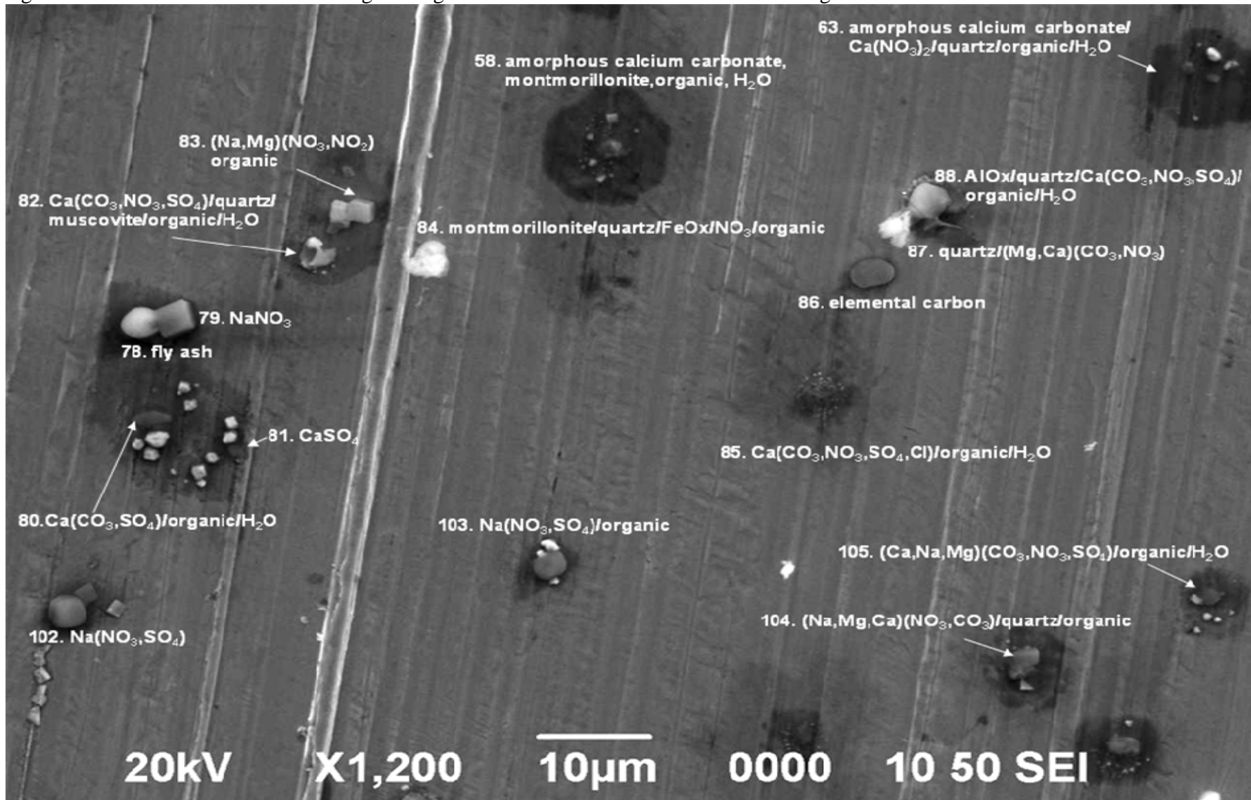
Figure S2. The third SEI obtained in a higher magnification than the overall SEI shown in Figure 1.
