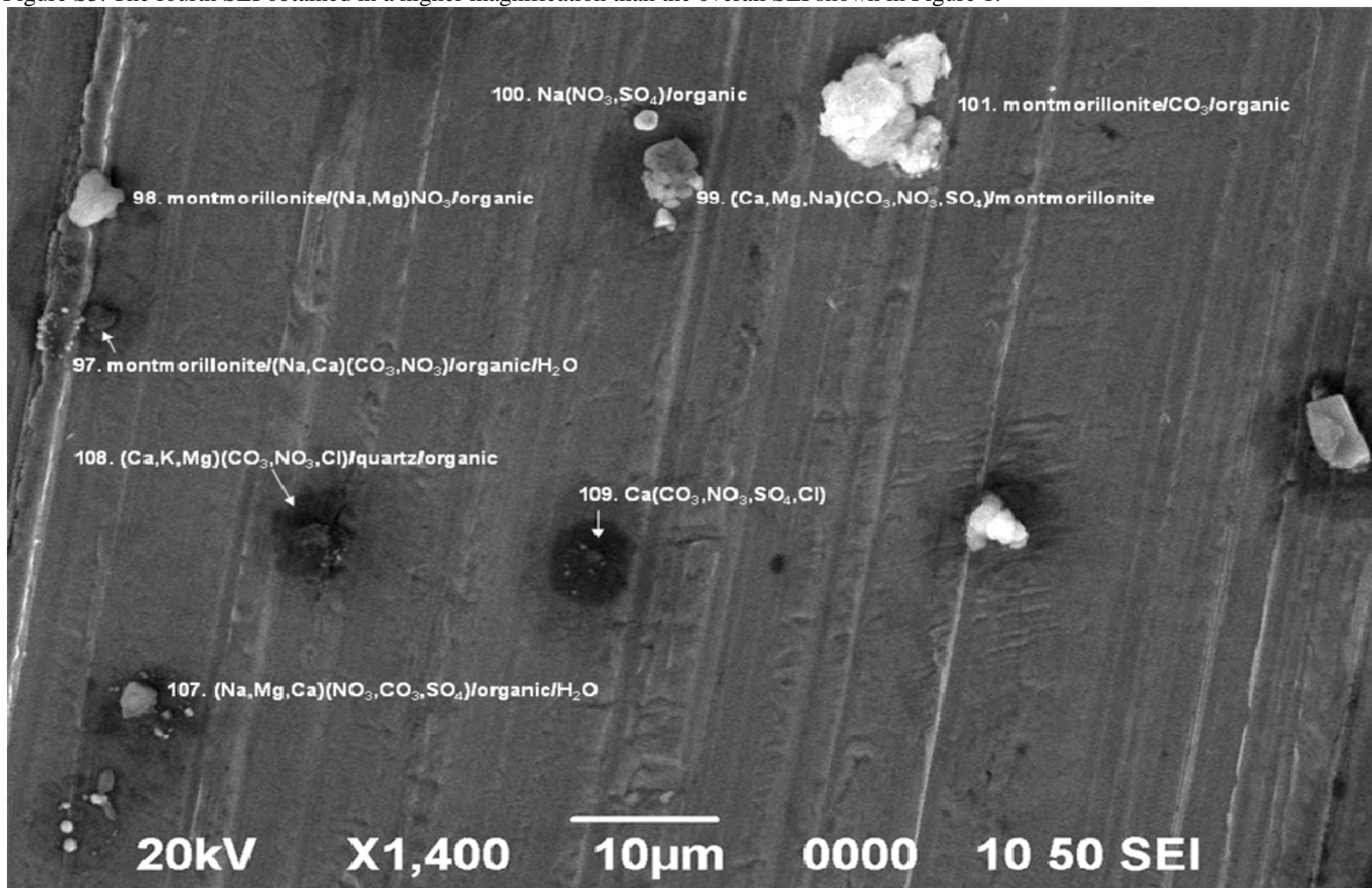
Figure S3. The fourth SEI obtained in a higher magnification than the overall SEI shown in Figure 1.
