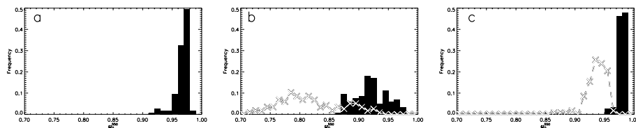
Fig. 7. Histograms of single scattering albedo values at 550 nm from SLRs during Fennec: (a) from observations as measured by the nephelometer and PSAP behind Rosemount inlets; (b) calculated using the full size distributions as shown in Fig. 5; (c) calculated using size distributions adjusted for inlet and pipe losses and enhancements, i.e. with reduced coarse mode. Solid bars in (b) and (c) assume m = 1.53 - 0.001i , dashed lines and crosses assume m = 1.53 - 0.003i .
