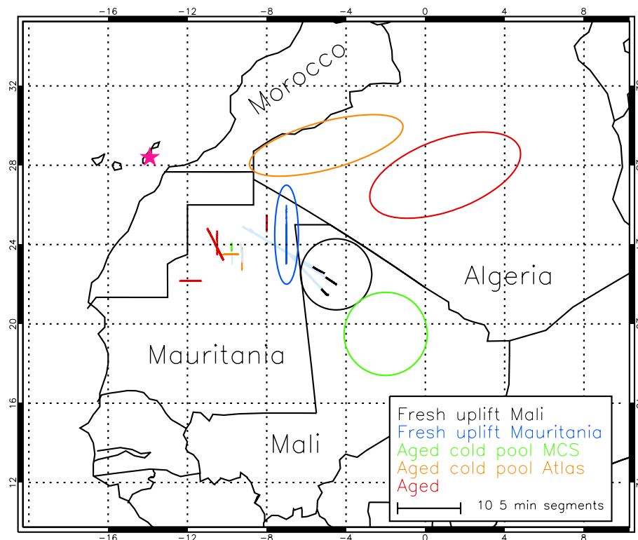
Fig. 1. Map showing locations of in-situ measurements and dust source regions. Straight lines show locations of in-situ straight and level runs (SLRs) used in this study. Circles indicate likely source areas of the dust sampled during the flights. Pink star indicates the location of Fuerteventura, Canary Islands, Spain, where the FAAM aircraft was based. Different colours correspond to the event categories described in Sect. 5 and Fig. 11. SLRs in grey are not included in Fig. 11.
