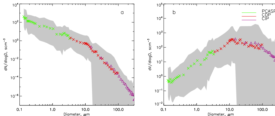
Fig. 5. Mean size distributions measured during Fennec 2011 SLRs, for number distribution (a) and volume distribution (b) . Data from the PCASP (green crosses), CDP (red crosses) and CIP (purple triangles) have been used. Grey shading represents minimum and maximum values measured during Fennec SLRs.
