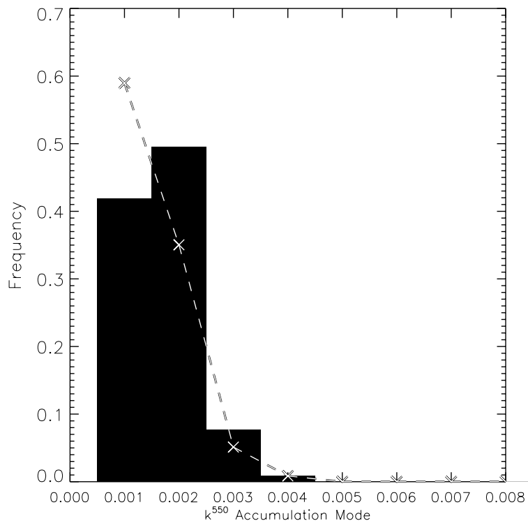
Fig. 9. Histogram showing derived k^{550} values for the accumulation mode for SLRs during Fenec. Solid bars show derivations using size distributions corrected using k^{550} = 0.001i , dashed line and crosses show derivations using size distributions corrected using k^{550} = 0.003i .
