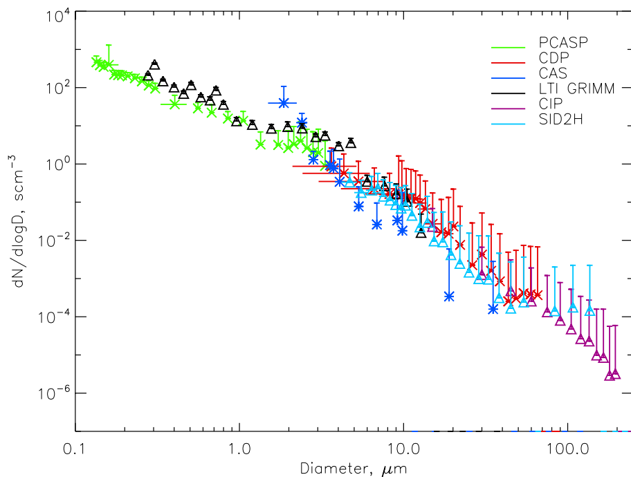
Fig. 3. Size distributions as measured by different instruments during Fennec 2011 for SLRs where all were operational, including refractive index corrections for m = 1.53 - 0.001i . Colours represent PCASP (green), LTI-GRIMM (black), CAS (dark blue), SID2H (light blue), CDP (red), CIP (purple). Vertical error bars indicate one standard deviation of the data. Upwards error bars only are shown for clarity. Horizontal error bars show uncertainty due to the non-monotonic relationship of scattering cross-section with particle size from refractive index corrections.
