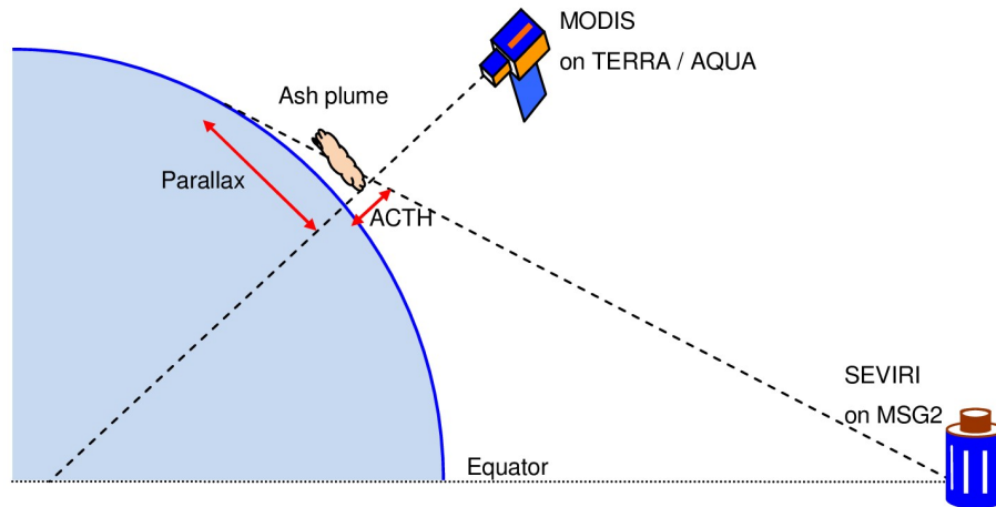
Fig. 1. If an ash cloud is observed simultaneously from two satellites the position of the cloud seems to be shifted for a parallax when comparing both datasets. The parallax is a consequence of viewing geometries of both satellites and the height of the ash cloud.
