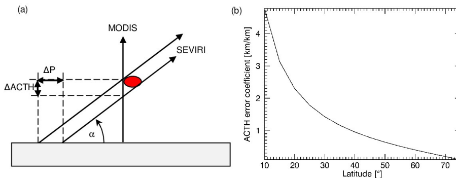
Fig. 8. ACTH error coefficient as a function of the latitude.
