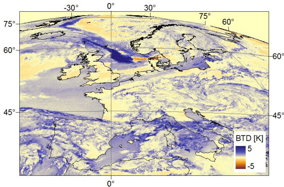
Fig. 4. BTD (data for 15 April at 20:00 UTC) reveals plumes dispersing at two different heights. Highly positive BTD values in dark blue over North Sea indicate ice crystals. Below it spreads a reddish plume with negative BTD.
