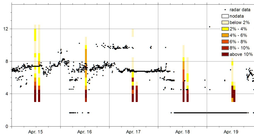
Fig. 7. Vertical distribution of ACTH for the period between 15 and 19 April. All pixels are classified according to their ACTH in one of the 500 m height classes. Colours represent the relative amount of pixels within a class (in percent) – dark colours show that there are many pixels in a height class. Because of two daytime MODIS overpasses two ACTH estimations can be done per day. On 16 April only one estimate is presented because of the unfavourable satellite's swath characteristics. The highest measured heights by the radar (Marzano et al., 2011) are shown for the comparison.
