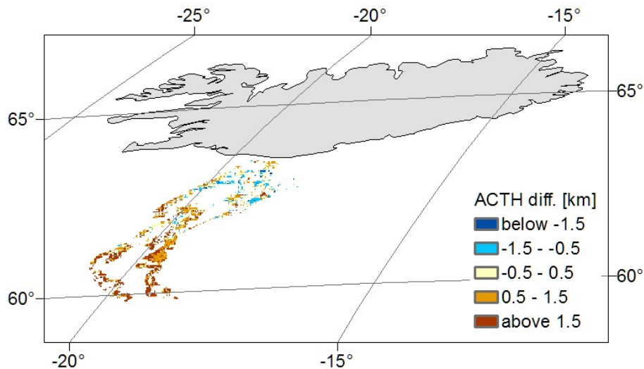
Fig. 9. ACTH difference between the case study estimate and MISR measurements on 19 April at 12:50 UTC.
