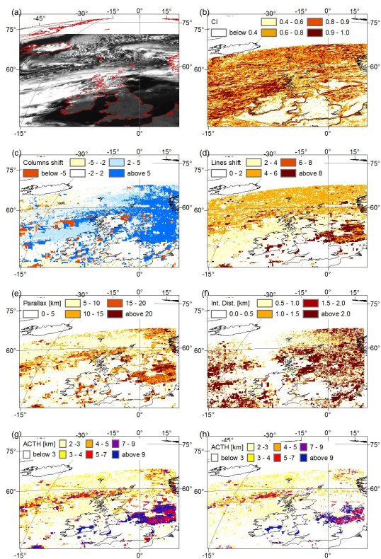
Fig. 5. SEVIRI data on 17 April at 13:12 UTC (a) ; the cross-correlation index between the SEVIRI image and MODIS image retrieved at 13:15 UTC (b) ; optimal matching shift between both datasets in column direction (c) ; optimal matching shift between both datasets in line direction (d) ; parallax between both datasets (e) ; intersection distance between lines of sight projected to the north direction (f) ; ACTH for all available pixels (g) ; ACTH for pixels where intersection distance projected to the north direction is lower than 1.5 km.
