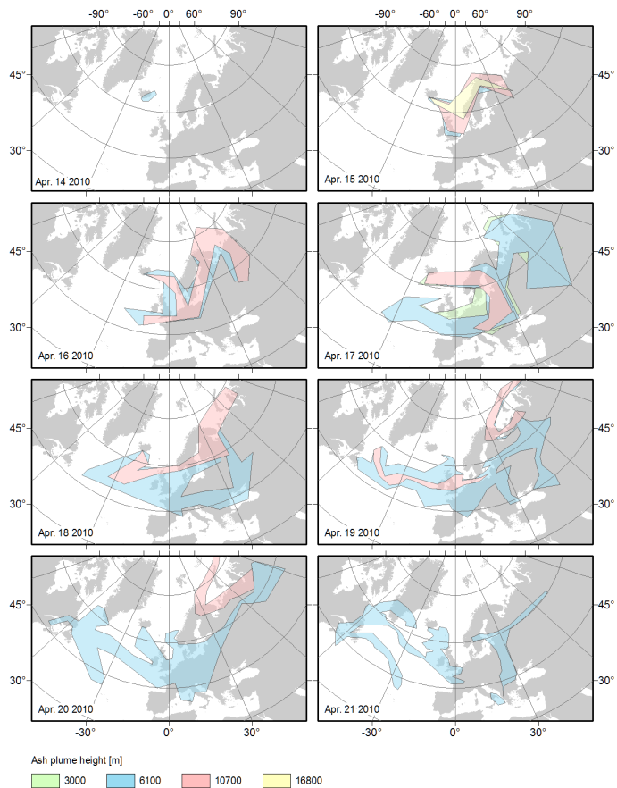
Fig. 3. Volcanic ash dispersion on standard Flight Levels (3000 m – FL100, 6100 m – FL200, 10700 m – FL350, 16800 m – FL550) for the eruption of Eyjafjallajökull in April 2010. These ash dispersion data are a product of the VAAC London.
