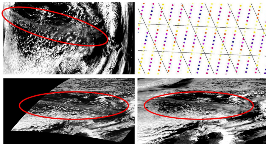
Fig. 2. Aggregation of MODIS data into SEVIRI's grid system; the ash cloud is marked by the red oval. Left above: an example of original MODIS data (part of MODIS band 1 data showing the Eyjafjalljökull ash cloud over the North Sea on 15 April 2010 at 11:35 UTC). Right above: a scheme of SEVIRI's point spread function – each dot represents a MODIS measurement, thus it is coloured according to its position within the SEVIRI pixel (dark purple dots represent greater weight than pale yellow dots). Left below: MODIS data transformed in the SEVIRI grid system (see the difference in the overall geometry that is a consequence of a difference in viewing angles of both instruments). Right below: SEVIRI data retrieved at approximately the same time as MODIS (11:27 UTC).
