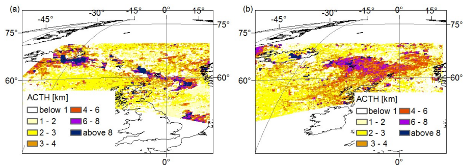
Fig. 6. Another example of ACTH on 15 April at 11:35 UTC (a) and on 19 April at 12:50 UTC.
