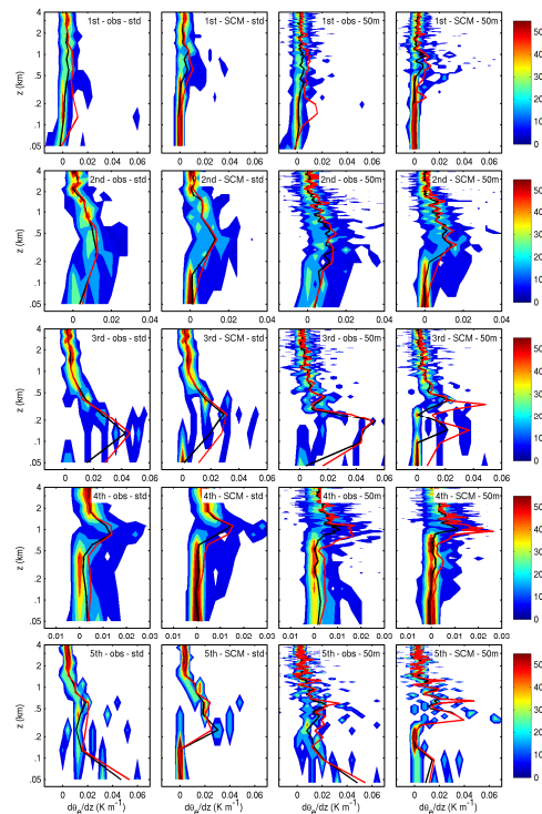
Fig. 5. Contours of the probability of static stability, given by the vertical derivative of equivalent potential temperature ( \partial\theta_e/\partial z ), as a function of height for the single-column model run initialised with observed surface temperature. The first and third columns show observations from the 6-hourly soundings for each regime, averaged onto the standard and 50 m vertical resolutions of the SCM, respectively. The second and fourth columns show SCM diagnostics at t + 6 h, run at standard and 50 m vertical resolution, respectively. The red and black lines are the mean and median static stability at each vertical level, respectively. Note the logarithmic height scale and the change in scale on the x axis.
