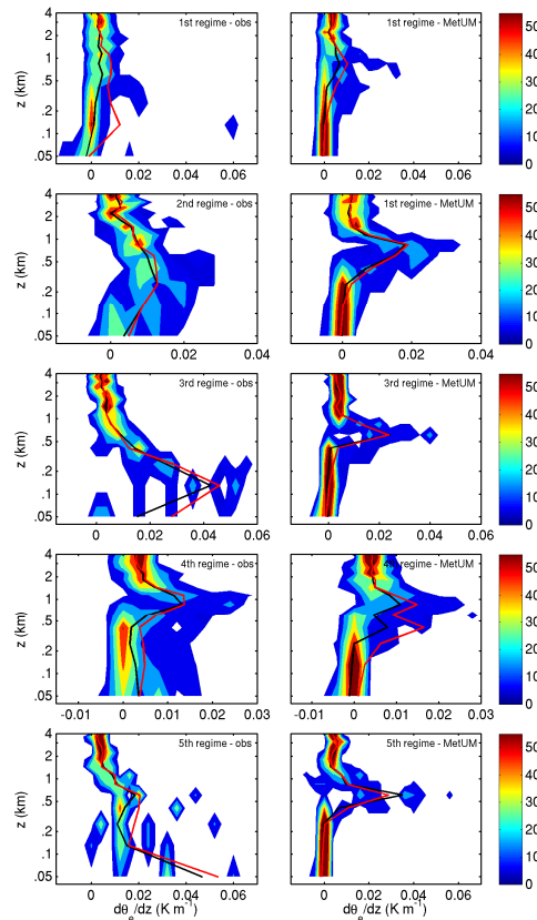
Fig. 4. Contours of the probability of static stability, given by the vertical derivative of equivalent potential temperature ( \partial\theta_e/\partial z ), as a function of height. Observations are from the 6-hourly soundings and the model data are from 3-hourly diagnostics. The red and black lines are the mean and median static stability at each vertical level, respectively. Note the logarithmic height scale and the change in scale on the x axis.
