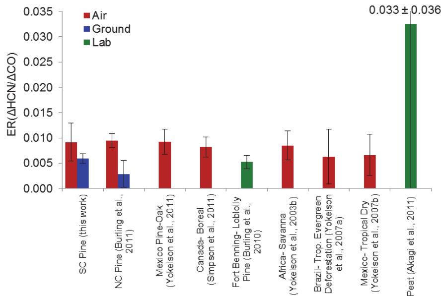
Fig. 10. Comparison of \Delta\text{HCN}/\Delta\text{CO} study-average emission ratios ( \text{mol mol}^{-1} ) measured from airborne (red), ground-based (blue), and laboratory (green) platforms from five North American studies in pine-forest fuels (leftmost bars). We also show four \text{ER}(\Delta\text{HCN}/\Delta\text{CO}) in other fuel types for comparison. Error bars ( 1-\sigma ) are included for all data. The large variation shown for peat is due to a very large value for Indonesian peat that is included in the calculation.
