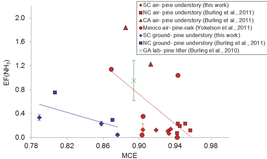
Fig. 9. EF(NH 3 ) (g kg -1 ) as a function of MCE for the South Carolina pine burns of this study (diamonds) measured from both airborne (red) and ground-based (blue) platforms. Error bars (1-σ) are included for data from this work (error bars from other works are included when available). We also show airborne and ground-based measurements in similar fuels from Burling et al. (2011) (squares), airborne data from Mexican pine-oak forests from Yokelson et al. (2011) (red circles), and pine litter laboratory data from Fort Benning, GA (Burling et al., 2010) (green). Negative correlations of EF(NH 3 ) vs. MCE for ground-based (blue line) and airborne (red line) measurements are also shown.
