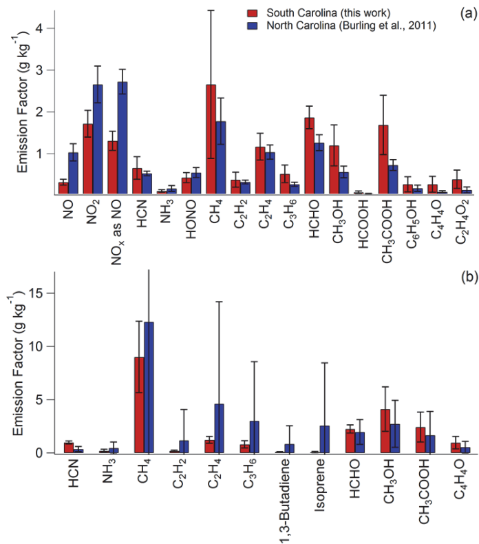
Fig. 6. Comparison of emission factors from this work (red) with Burling et al. (2011) (blue) from (a) airborne and (b) ground-based platforms.
