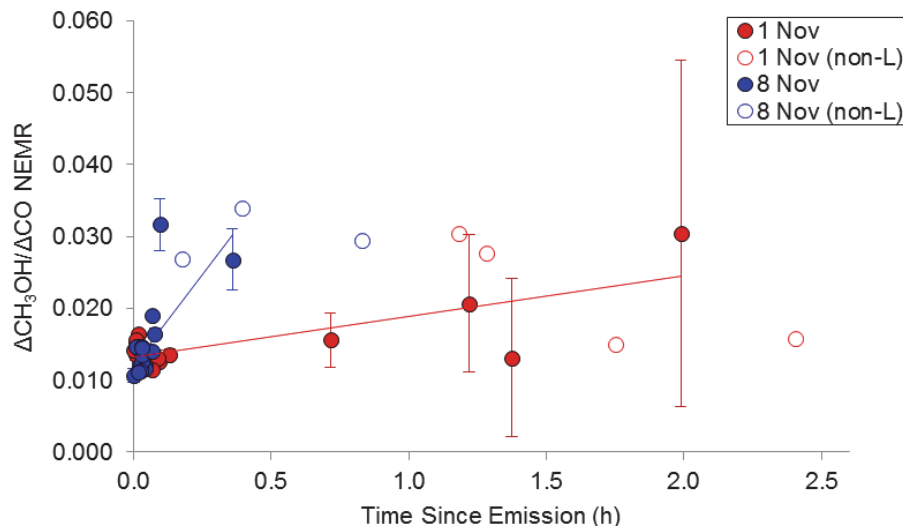
Fig. 14. \Delta\text{CH}_3\text{OH}/\Delta\text{CO} vs. time since emission (h). Airborne measurements were collected up to \sim 2.5 h downwind. Fires on which we were able to collect downwind data with good SNR, Block 9b (1 November, red) and Francis Marion (8 November, blue), are included here. The y-intercept of the trendlines is forced to the average \text{ER}(\text{CH}_3\text{OH}) at time t = 0 for each fire. Solid circles reflect data that were considered Lagrangian while open circles labeled “non-L” represent non-Lagrangian samples collected on that respective day. Vertical error bars reflect instrument uncertainty in methanol (500 ppt).
