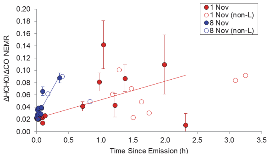
Fig. 15. \Delta\text{HCHO}/\Delta\text{CO} vs. time since emission (h). Airborne measurements were collected up to \sim 2.5 h downwind. Fires with good downwind data, Block 9b (1 November, red) and Francis Marion (8 November, blue), are included here. The y-intercept of the trendlines is forced to the average ER(HCHO) at time t = 0 for each fire. Solid circles reflect data that were considered Lagrangian while open circles labeled “non-L” represent non-Lagrangian samples collected on that respective day. Vertical error bars reflect instrument uncertainty in formaldehyde (1 ppb).
