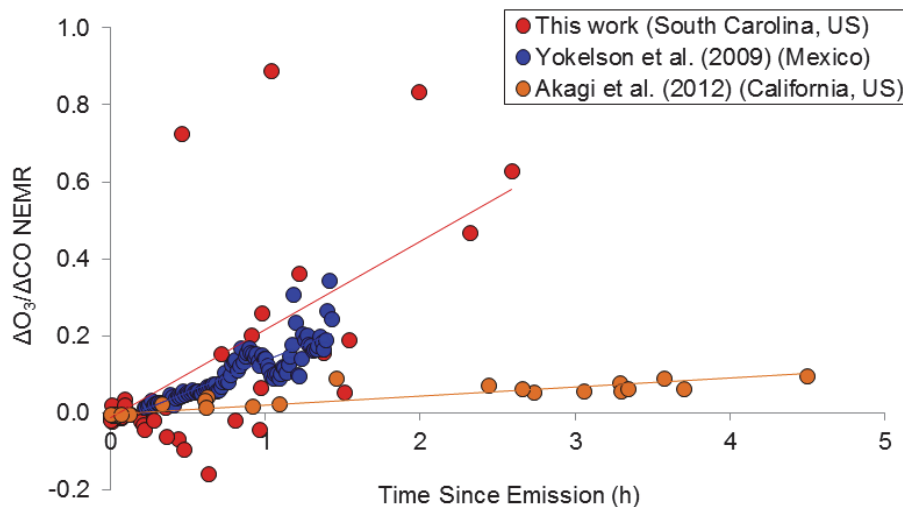
Fig. 13. \Delta O_3 / \Delta CO vs. time since emission from this study (red), Yokelson et al. (2009) (blue), and Akagi et al. (2012) (orange).
