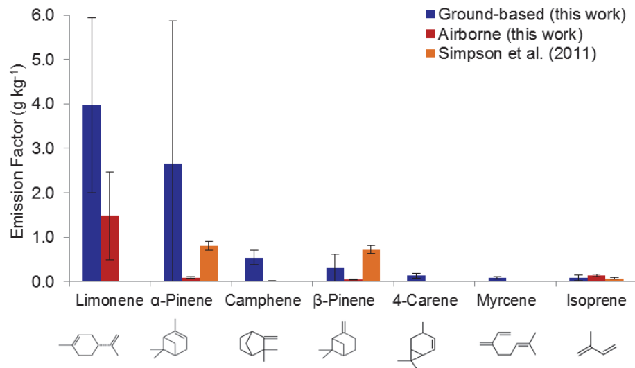
Fig. 7. Emission factors ( \text{g kg}^{-1} ) of monoterpenes and isoprene measured in this work from ground-based (blue) and airborne (red) platforms. Molecular structures are shown below each compound. We compare with data from Simpson et al. (2011) who measured \alpha -pinene, \beta -pinene and isoprene only from an airborne platform (orange). Error bars represent the 1 - \sigma standard deviation in EF.
