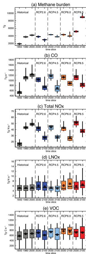
Fig. 1. Burdens and emissions of ozone precursors used in the ACCMIP scenarios and time slices, showing (a) the tropospheric methane burden, and yearly total (b) CO emissions, (c) total NO x emissions, (d) lightning NO x emissions and (e) VOC emissions. The spread of the emissions/burden in each model is indicated for each scenario and time slice, with filled box showing the interquartile range, the whiskers indicating the full range, and the dot and line indicating the mean and median respectively. Not all models completed all the scenarios.
