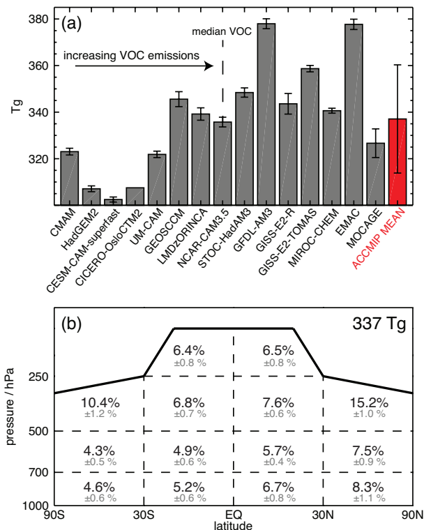
Fig. 3. (a) Tropospheric ozone burdens for the ACCMIP models from the Hist 2000 simulations. Error bars for the models indicate the variability in the burden between different years of a model’s time slice ( \pm 1 std. dev.). The error bar on the ensemble mean burden indicates the inter-model spread of the burden ( \pm 1 std. dev.). Models are arranged in order of increasing VOC emissions. (b) Distribution of the mean ozone burden throughout the troposphere for the mean model, using the “boxes” recommended by Lawrence et al. (2001) for reporting OH concentrations. The solid line indicates the tropopause (see text for definition).
