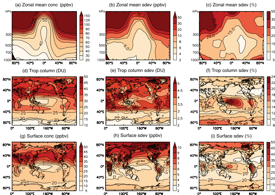
Fig. 2. ACCMIP ensemble mean, annual mean ozone climatologies and their inter-model variability, for the 2000 time slice of the Historical simulation. Top row shows zonal mean ozone, the middle row shows the tropospheric ozone column, and the bottom row shows surface ozone. For each row, the left hand panels show the absolute values of the ozone variable: ppbv for the zonal mean and surface concentrations, and Dobson units (DU) for the tropospheric column. The middle panels show the absolute standard deviations in the same units. The right hand column expresses the standard deviation as a percentage of the ensemble mean value (also known as the coefficient of variation). Note that each panel has a different scale.
