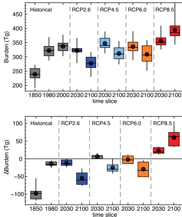
Fig. 7. (a) Modelled tropospheric ozone burdens for the different scenarios and time slices. (b) Change in the tropospheric burden, relative to the Hist 2000 simulation. The box, whiskers, line and dot show the interquartile range, full range, median and mean burdens and differences, in a similar style to Fig. 1.
