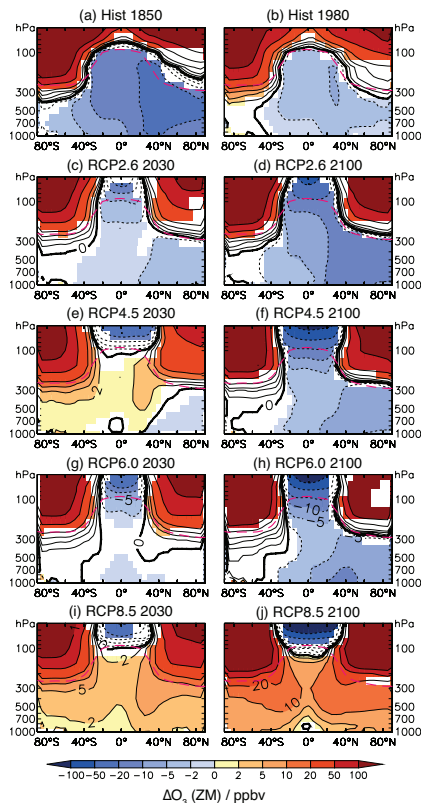
Fig. 9. Absolute change in annual zonal mean ozone for the ACCMIP ensemble mean compared to the Hist 2000 simulation (ppbv). Top row shows the difference for the Hist 1850 and 1980 time slices. The next four rows show the difference for the 2030 and 2100 time slices of the RCP simulations. Non-white regions indicate where the change is significant at the 5% level, based on the spread of the differences between the models. The dashed red line indicates the position of the annual zonal mean 150 ppbv ozone contour from the Hist 1850 simulation.
