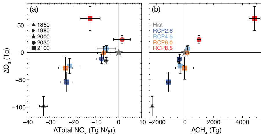
Fig. 12. ACCMIP ensemble mean change in the tropospheric ozone burden compared to the Hist 2000 simulation as a function of (a) changes in total \text{NO}_x emissions and (b) changes in the tropospheric methane burden. Error bars indicate \pm 1 std. dev. of the changes in ozone, \text{NO}_x emissions and methane burdens, calculated from the spread of the models. Different colours represent the different scenarios, whereas different symbols represent the different time slices.
