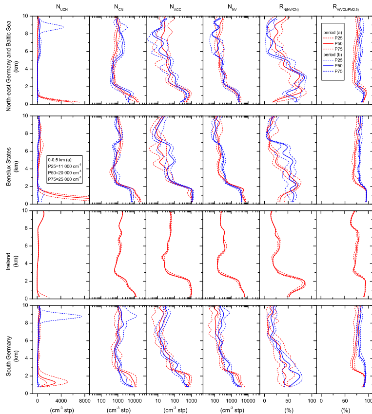
Fig. 5. Vertical profiles of number concentration of particles in diameter D_P 0.004\text{--}0.01\ \mu\text{m} N_{UCN} , D_P > 0.01\ \mu\text{m} N_{CN} , D_P 0.15\text{--}1.0\ \mu\text{m} N_{ACC} , and particles containing a non-volatile core N_{NV} ( 250^\circ\text{C} ). All number concentrations are reported in particles \text{cm}^{-3} at standard temperature and pressure (stp). In addition, number fractions of non-volatile particles R_{NV/CN} and volume ratios of volatile matter R_V\text{VOL}/\text{PM}_{2.5} are given in %. The red (blue) line shows values for the period between 1–15 (16–31) May, i.e. period (a) and (b). Each vertical profile contains Median and 1st and 3rd Quartiles.
