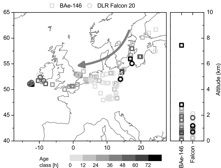
Fig. 7. Horizontal and vertical distribution of classified flight sequences using trajectory analysis. The arrow depicts the main air mass transport direction during the anticyclonic conditions. For detailed information see text.
