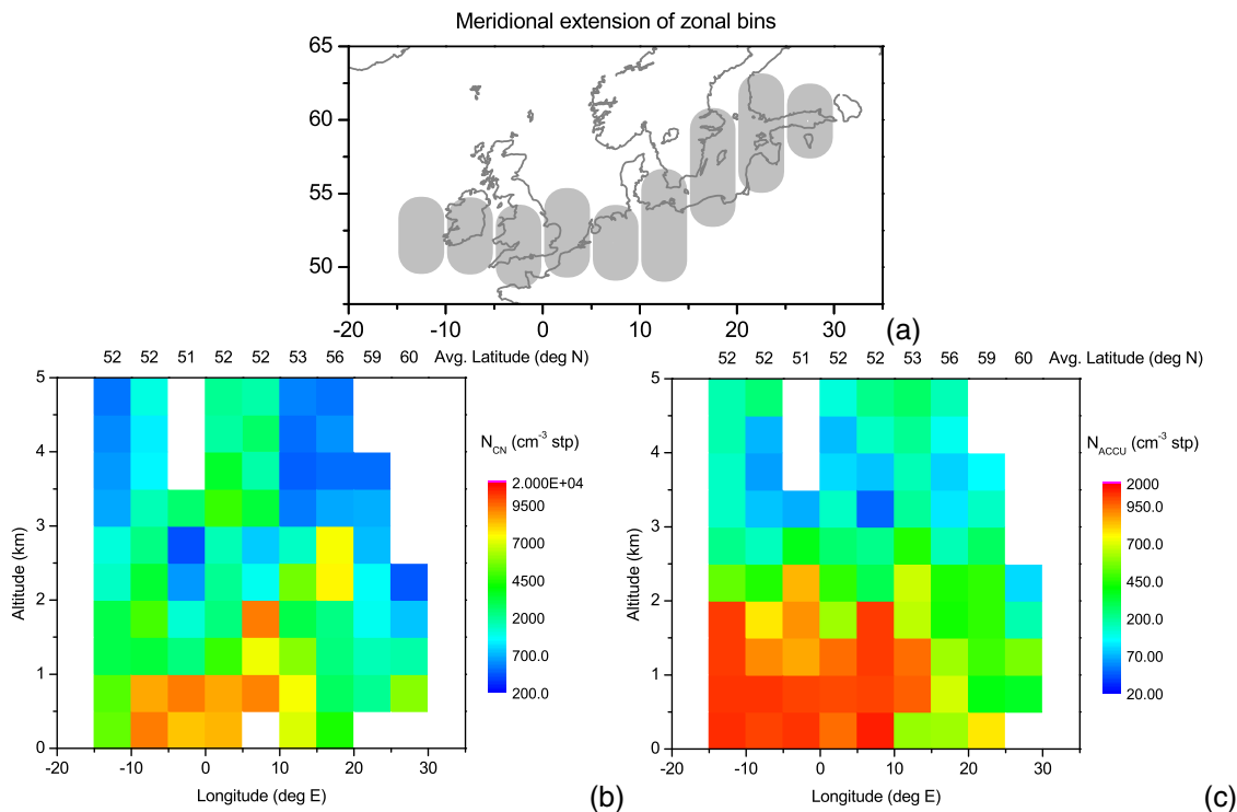
Fig. 4. Zonal distribution of binned vertical profiles (a) of CN (b) and ACC (c) number concentrations North of 50° N derived from DLR Falcon 20 and FAAM BAe-146 measurements. Please note the variable average latitude of the measurements and the logarithmic colour scale.
