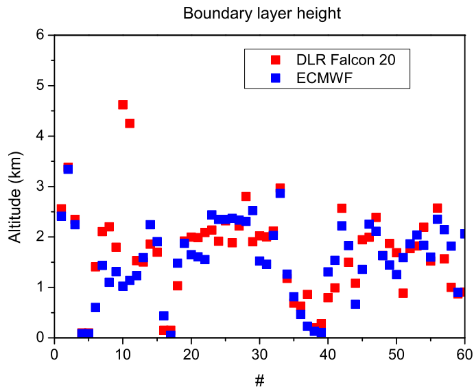
Fig. A2. Comparison of the boundary layer height (km a.s.l.) as observed during the in-situ measurements of DLR Falcon 20 (red) with the boundary layer height retrieved from the ECMWF model analysis (blue).
