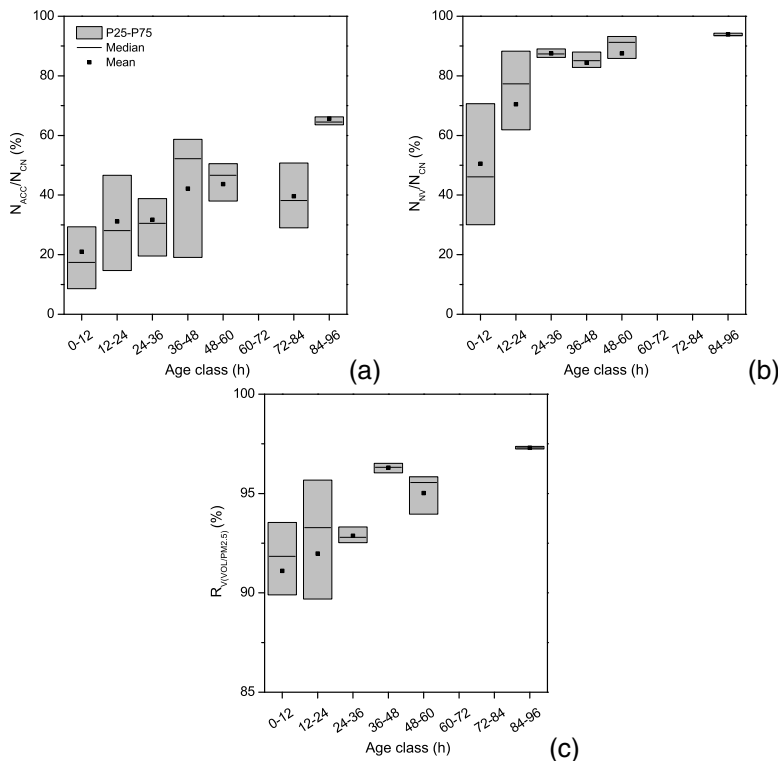
Fig. 8. Classification of measurements into time intervals of the maximum contribution of emissions along the air mass transport pathway within in the last 120 h. Panel (a) shows the ratio of accumulation mode particles to total number concentration, panel (b) the ratio of non volatile particles to total number concentration and panel (c) the ratio of the volatile aerosol volume to the total aerosol volume. Median, mean and 1st and 3rd Quartiles (P25, P75) are given.
