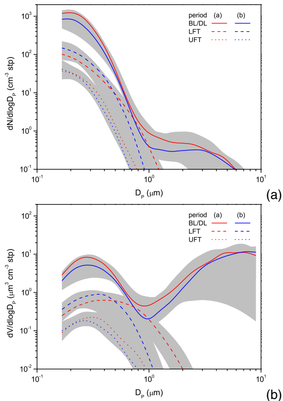
Fig. 6. Number size distributions (a) and volume size distributions (b) above all regions. Concentrations are given at standard temperature and pressure. The panels show measurements performed during horizontal flight legs within the boundary layer and decoupled layers (BL/DL), the lower free troposphere (LFT) and upper free troposphere (UFT). The red and blue lines show Median values for periods (a) and (b), respectively. The grey shade indicates the 1st and 3rd Quartiles.
