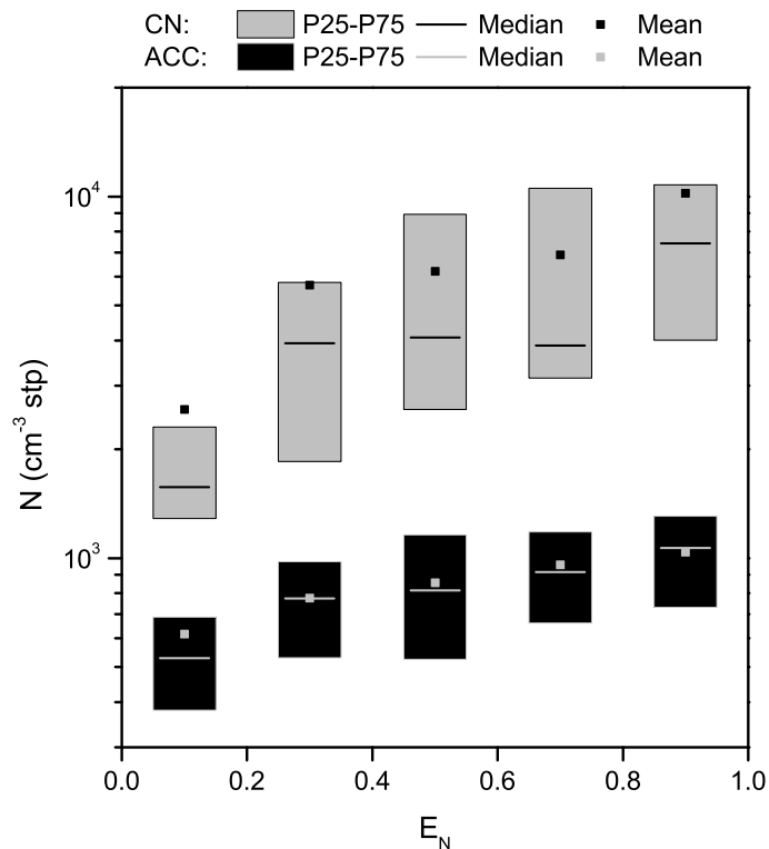
Fig. 3. Comparison of the normalized emission factor E_N with measured CN (grey) and ACC (black) number concentrations (see Fig. 2). The floating columns show the 1st and 3rd Quartiles (lower and upper column limits) and the Median (centre line) for 0.2 E_N bins.
