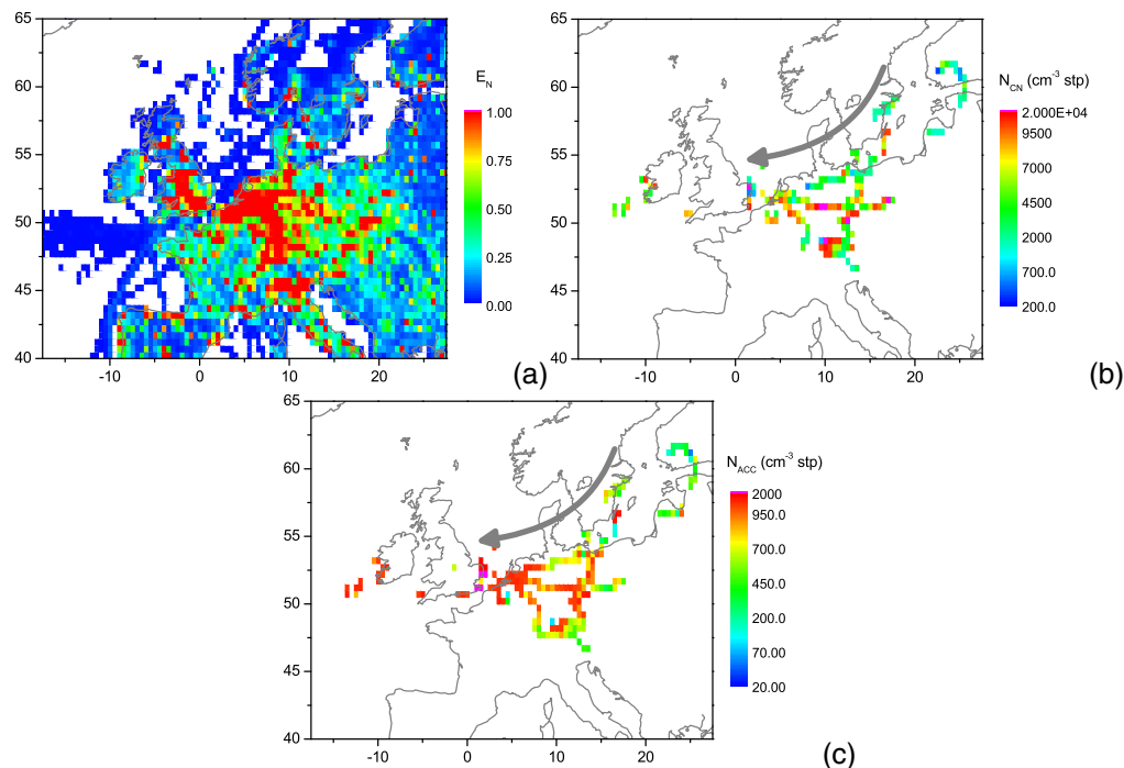
Fig. 2. Normalized emission factor E_N (a) based on the EDGARv4.1 emission database ( http://edgar.jrc.ec.europa.eu/ ) and horizontal distributions of CN (b) and ACC (c) number concentrations within the boundary layer derived from DLR Falcon 20 and FAAM BAe-146 measurements. Average values are given for a 0.5^\circ \times 0.5^\circ grid. The grey arrow (b, c) indicates the main air mass transport direction. Please note the logarithmic colour scale for the particle number concentrations.
