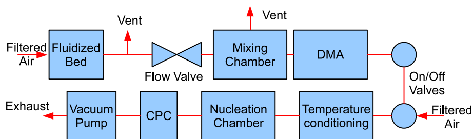
Fig. 1. Block diagram of the experiment. Aerosol particles are dispersed using a fluidized bed, then size selected with a differential mobility analyzer. The aerosol laden air stream is then cooled to a temperature close to the one selected for the experiment and pulled past the test droplet. The concentration is monitored with a condensation particle counter.
