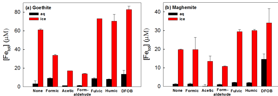
Fig. 1. Production of total dissolved iron from (a) goethite ( \alpha -FeOOH) and (b) maghemite ( \gamma -Fe 2 O 3 ) under dark condition in the presence of various organic complexing ligands in water (25 °C) and ice (-20 °C) after 72 h. Experimental conditions: [\alpha -FeOOH or \gamma -Fe 2 O 3 ] i = 0.2 g l -1 , [organic ligand] = 6 mM, [fulvic or humic acid] = 1 ppm, [DFOB] = 50 μM, and pH i = 3.00 ± 0.05.
