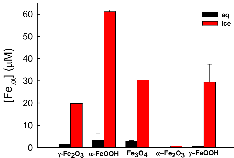
Fig. 2. Dissolved iron formation from various iron oxides in the absence of organic complexing ligand under dark condition. Aqueous samples (black) were maintained at room temperature and ice samples (red) at -20^{\circ}\text{C} for 72 h. Experimental conditions: [\text{iron oxide}] = 0.2 \text{ g l}^{-1} and \text{pH}_i = 3.00 \pm 0.05 .
