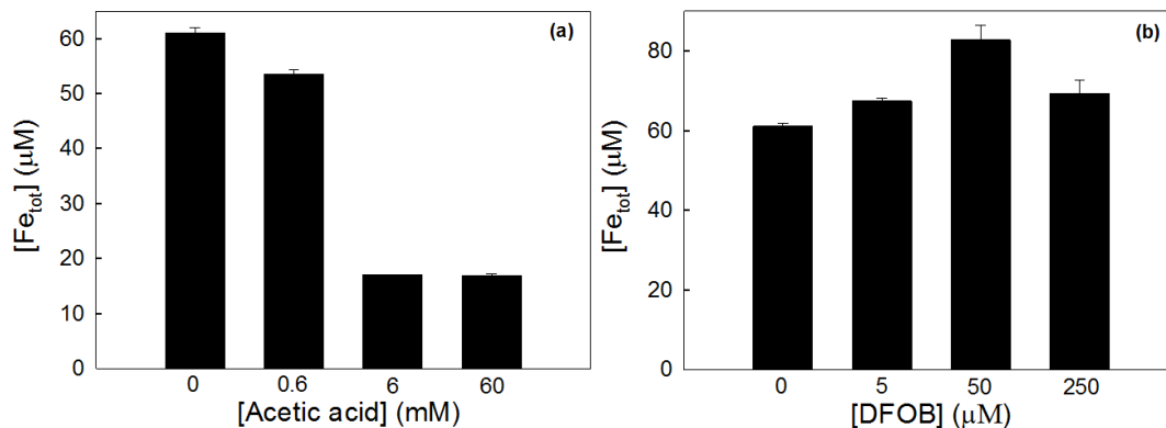
Fig. 4. Total dissolved iron generation from goethite in the presence of various concentrations of (a) acetic acid and (b) DFOB. Experimental conditions: [\alpha\text{-FeOOH}]_i = 0.2 \text{ g l}^{-1} , and \text{pH}_i = 3.00 \pm 0.05 .
