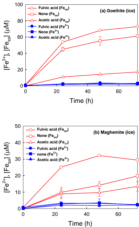
Fig. 3. The time profiles of dissolved iron ( \text{Fe}^{2+} and \text{Fe}_{\text{tot}} ) generation from iron oxides in ice: (a) goethite and (b) maghemite. Experimental conditions: [\alpha\text{-FeOOH} or \gamma\text{-Fe}_2\text{O}_3]_i = 0.2 \text{ g l}^{-1} , [\text{fulvic acid}] = 1 \text{ ppm} , [\text{acetic acid}] = 6 \text{ mM} , and \text{pH}_i = 3.00 \pm 0.05 .
