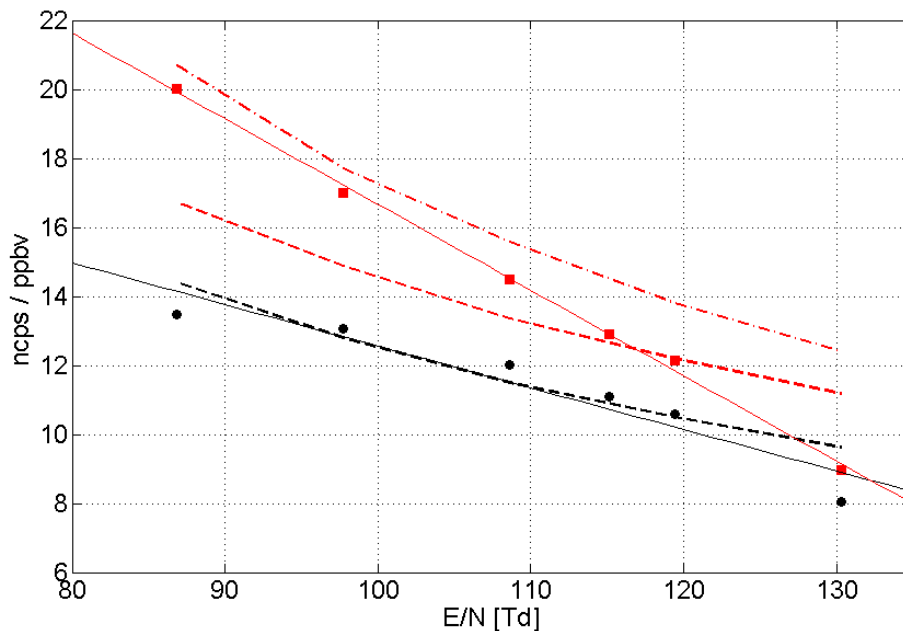
Fig. 3. Normalized sensitivities plotted as a function of E N^{-1} . Isoprene (black) and 232 MBO (red) exhibit higher sensitivities at lower collisional energies. The dashed lines indicate a theoretically calculated response curve based on a change in reaction time for a constant rate coefficient; the red dashed dotted line indicates the case using a varying rate coefficient for 232 MBO; the thin solid lines depict a linear fit ( y = ax + b ) through measured data yielding the following fitting coefficients: isoprene: a = -0.12 , b = 24.6 and 232 MBO a = -0.25 , b = 41.5 .
