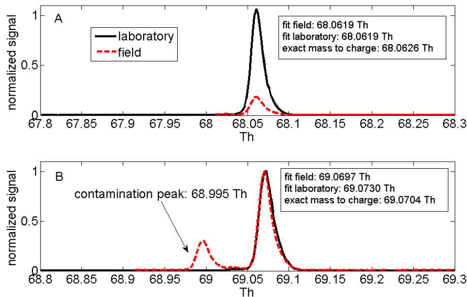
Fig. 1. Observed mass spectra for field and laboratory measurements depicting the molecular ion distribution on m/z^{-1} 68 + Th (A) and m/z^{-1} 69 + Th (B). Spectra are normalized by the 232 MBO count rate.
