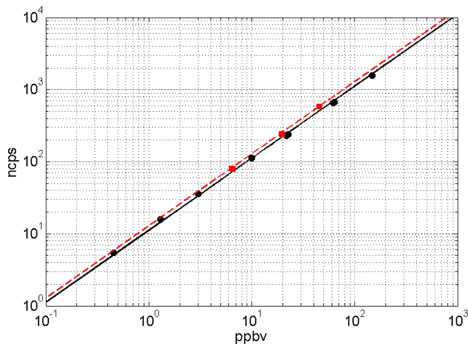
Fig. 2. Multipoint calibration curve for isoprene (black) and 232 MBO (red). Regression lines yield 11.1 \pm 0.1 ncps ppbv -1 and 12.9 \pm 0.1 ncps ppbv -1 for isoprene and 232 MBO, respectively.
