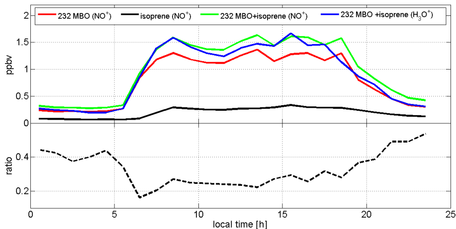
Fig. 5. Diurnal concentrations of isoprene and 232 MBO using two PTR-TOF-MS instruments (upper panel); one instrument was operated in \text{H}_3\text{O}^+ mode depicting 232 MBO + isoprene (blue trace); the other instrument was operated in \text{NO}^+ mode separating 232 MBO (red) and isoprene (black). The sum of the two is also plotted for comparison (green trace). The lower panel depicts the ratio between isoprene and 232 MBO.
