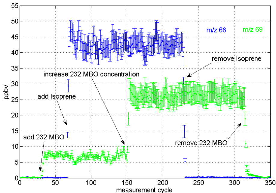
Fig. 4. Interference test: each measurement cycle represents a 1.5 s time interval; 232 MBO (green) and isoprene (blue) concentrations are varied as indicated in the graph. Error bars represent 1 \sigma .
