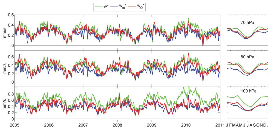
Fig. 3. Time series and mean seasonal cycles of the three upwelling estimates averaged over 18^{\circ} N–S at 70, 80 and 100 hPa (top to bottom panels). Green: residual circulation ( \bar{w}^* ), blue: momentum balance estimate ( \bar{w}_m^* ), and red: thermodynamic estimate ( \bar{w}_Q^* ). Time series are 11-days running means. The annual cycles are calculated as monthly means over 2005–2010 ( \text{mm s}^{-1} ).
