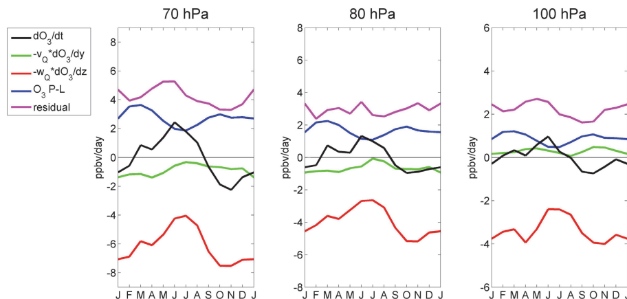
Fig. 6. Mean seasonal cycle for the period 2005–2010 of the terms in the continuity equation for ozone concentration (Eq. 5) averaged over 18^\circ N–S at the indicated levels. The purple line is the residual to the explicitly evaluated terms ( \text{ppbv day}^{-1} ).
