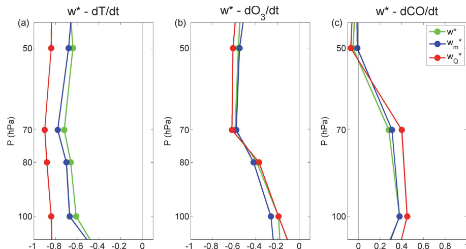
Fig. 10. Linear correlations as a function of altitude between the upwelling estimates and temperature (a) , ozone (b) and CO (c) tendencies. Results are shown for the three estimates ( \bar{w}^* in green, \bar{w}_m^* in blue and \bar{w}_Q^* in red). The correlations are calculated between the sub-seasonal time series (periods > 6 days and < 1 yr) as shown in Fig. 10 but for the entire period (2005–2010). The 95 % significance level is \sim 0.10 .
