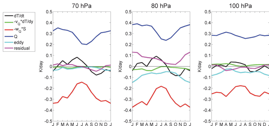
Fig. 5. Mean seasonal cycle (monthly means for the period 2005–2010) of the terms in the thermodynamic equation (Eq. 4) averaged over 18° N–S for the three pressure levels indicated. The purple line is the residual from the explicitly evaluated terms ( \text{K day}^{-1} ).
