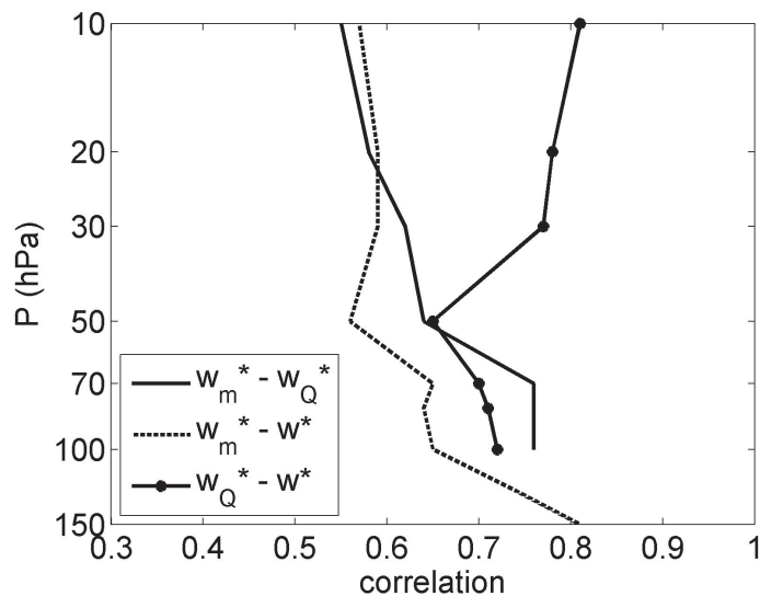
Fig. 4. Linear correlations among the time series of the three upwelling estimates as a function of log-pressure altitude.
