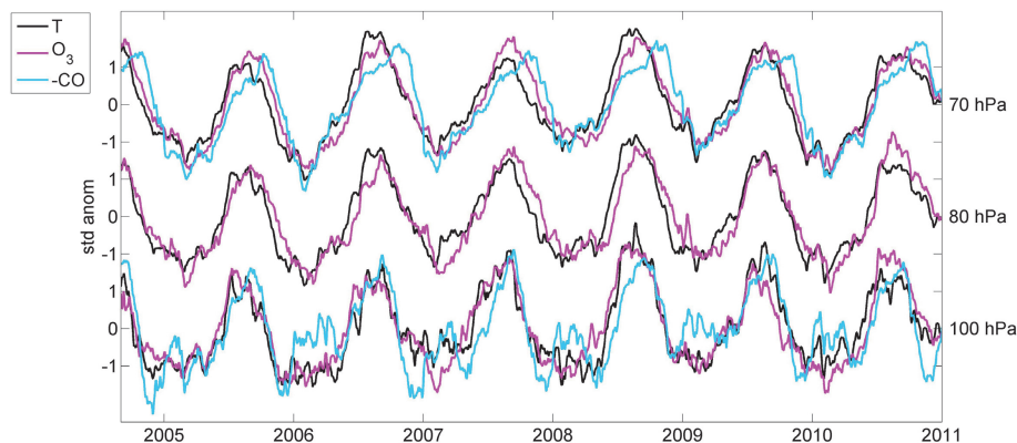
Fig. 1. Time series of standardized anomalies of daily temperatures from ERA-Interim and ozone and CO mixing ratio measurements from MLS averaged over 18^{\circ}\text{N}\text{--S} at three pressure levels across the tropical tropopause (70, 80 and 100 hPa from top to bottom). 3-days running means were applied to the daily series. CO concentrations are plotted on a reversed scale in order to highlight the common fluctuations.
