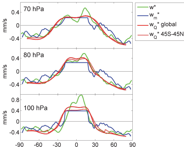
Fig. 2. Latitudinal structure of the three upwelling estimates at the indicated pressure levels. Green: residual circulation ( \bar{w}^* ), blue: momentum balance estimate ( \bar{w}_m^* ), and red: thermodynamic estimate ( \bar{w}_Q^* ). Two red lines are shown: the solid line is the thermodynamic upwelling estimate computed with the global adjustment and the dashed line adjusting only within the range 45° N–S (see text for details) ( \text{mm s}^{-1} ).
