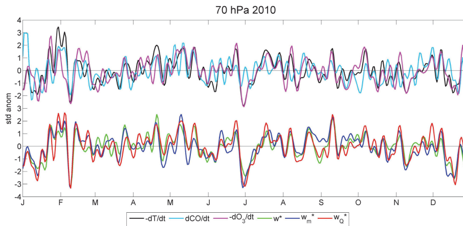
Fig. 9. Top curves show time series for the year 2010 of standardized anomalies of temperature (black), ozone (purple) and CO (light blue) tendencies. Lower curves show the three estimates of upwelling: \bar{w}^* (green), \bar{w}_m^* (blue) and \bar{w}_q^* (red) at 70 hPa. Temperature and ozone tendencies are plotted on a reversed scale. All series are filtered to remove timescales \geq 1 yr and \leq 6 days.
