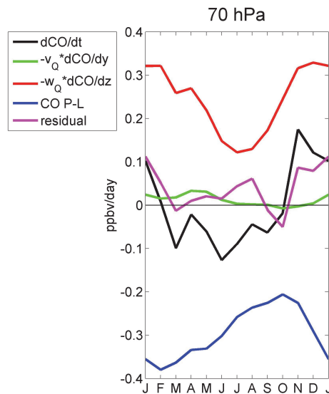
Fig. 7. Mean seasonal cycle for the for the CO continuity equation at 70 hPa (ppbv day -1 ).
