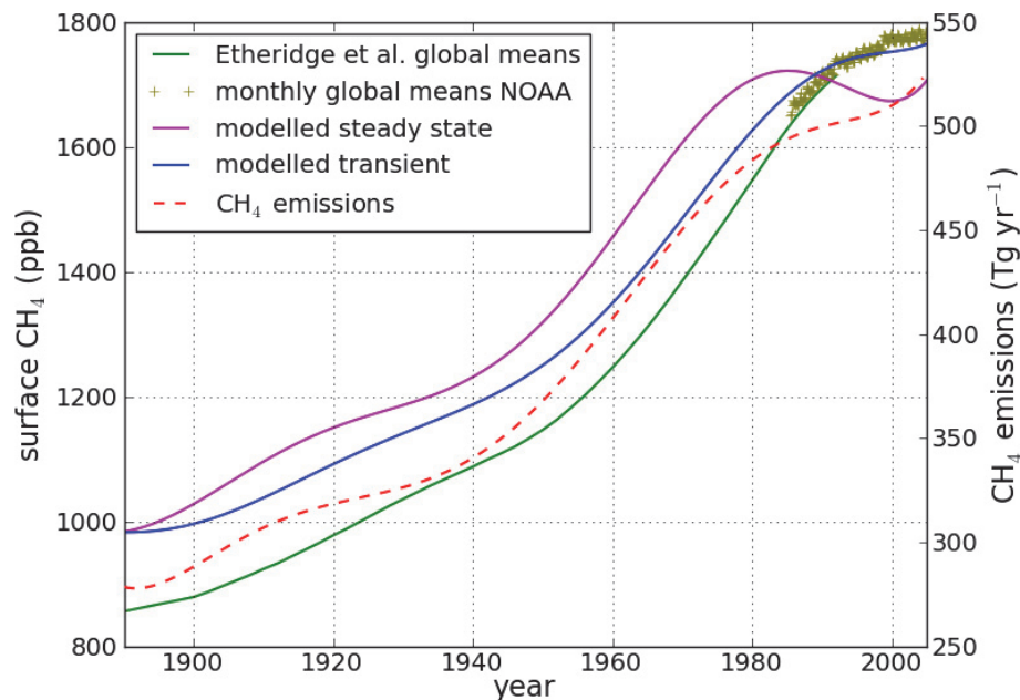
Fig. 3. Observed and modeled steady-state and transient evolution of methane surface concentrations between 1890 and 2005. Observation-based global means are calculated by Etheridge et al. (1998) based on ice-core data (green line), and more recent global means are calculated using measurements at South Pole and Alert NOAA stations (green crosses). Also methane emissions implemented in the model are shown (red dotted line, with scale on the right axis).
