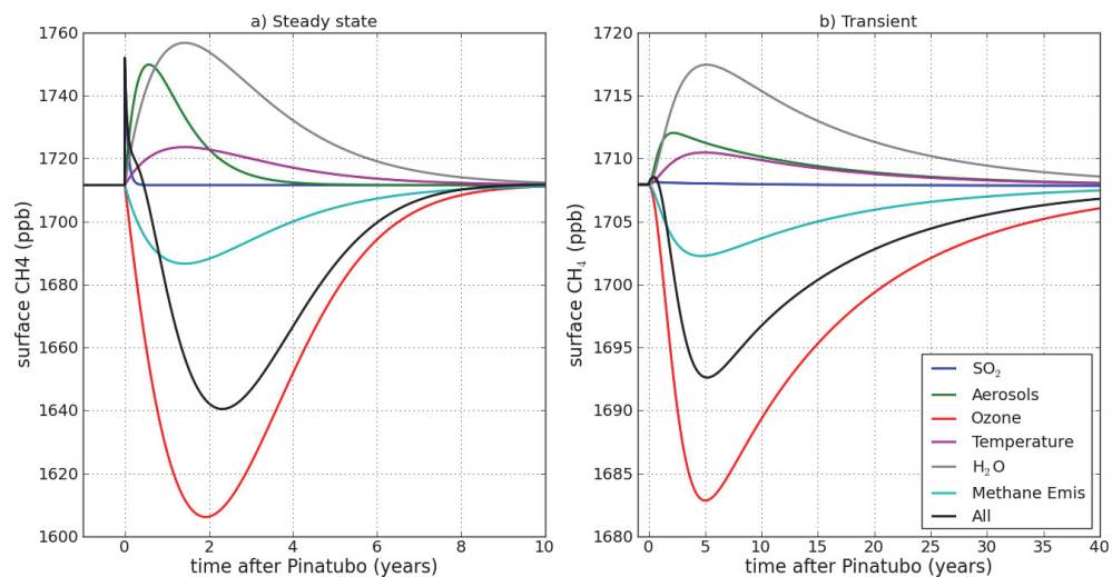
Fig. 5. Effect of the different Pinatubo forcings on surface methane (a) steady-state and (b) transient evolution.
