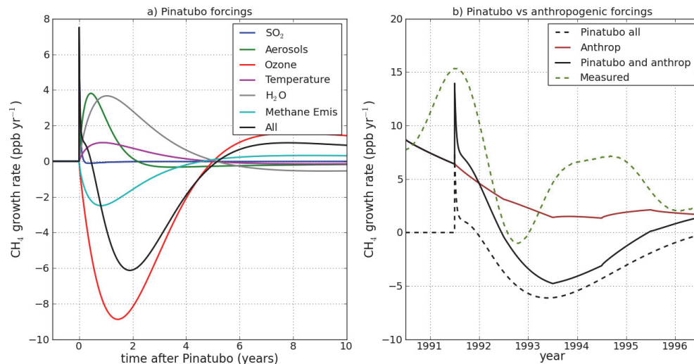
Fig. 6. Growth rate evolution after Pinatubo including (a) natural effects due to the eruption and (b) both natural effects due to the eruption and variation in anthropogenic emissions. Also shown in (b) is the global averaged growth rate obtained using the marine reference boundary matrix from GLOBALVIEW-CH 4 (2009).
