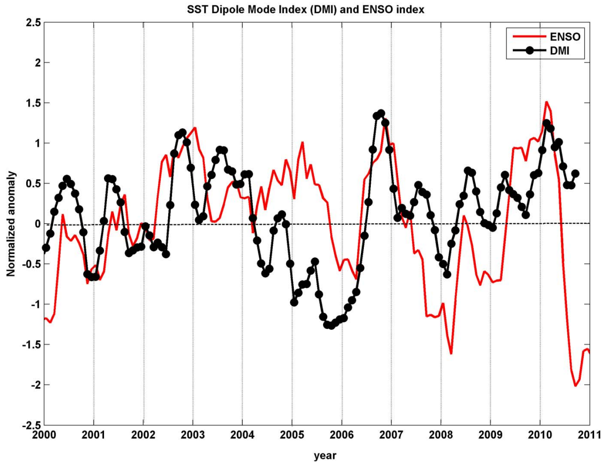
Figure S1: Time series of dipole mode index (DMI; Black) and Nino3.4 index (red) from 2000 to 2011. This is similar to Figure 4 of Field et al. (2009), but with a different time range.
