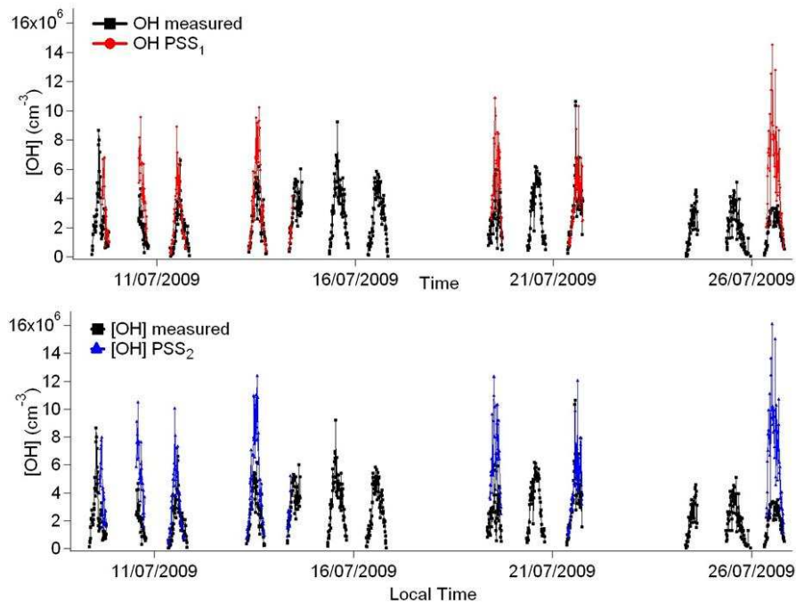
Fig. 4. Observed OH concentrations (black squares) compared with two PSS calculations including (PSS1) or not (PSS2) the ozonolysis of alkenes as OH source. The calculations of both PSS approaches are carried out only when all the parameters used in it are available.
