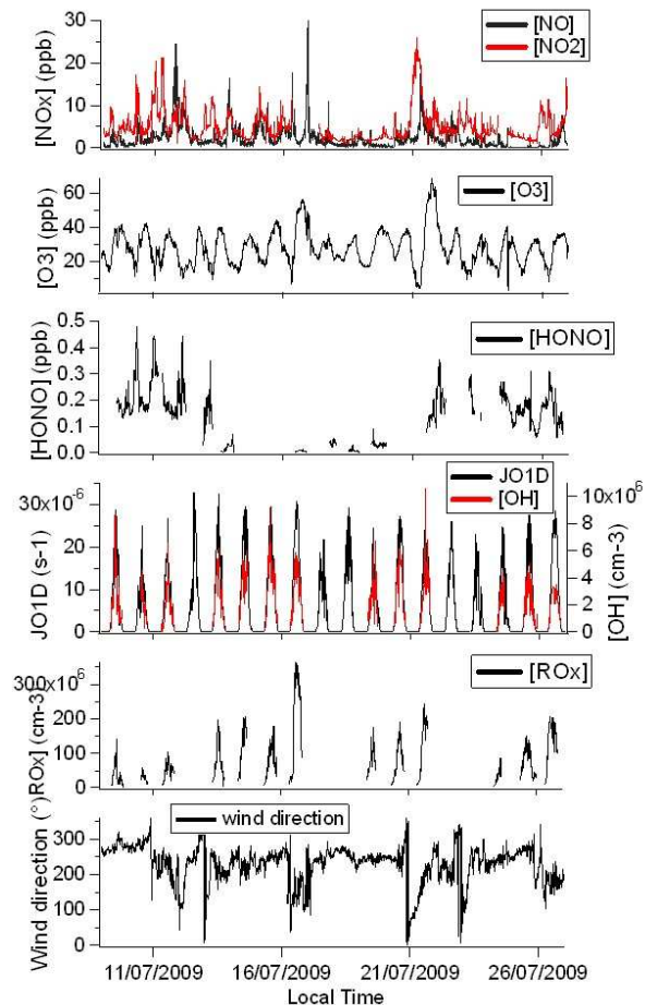
Fig. 2. 10 min data of NO x , O 3 , HONO, J(O 1 D), OH, RO x and wind direction during the MEGAPOLI summer field campaign in Palaiseau, 9–26 July 2009.
