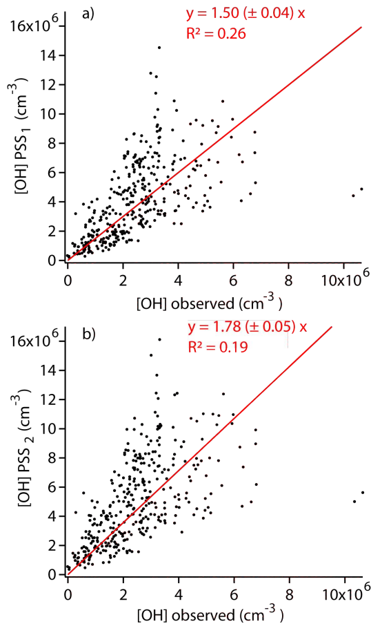
Fig. 6. Correlations between observed OH concentrations and OH PSS1 (panel a) and OH PSS2 (panel b) for the whole study period.
