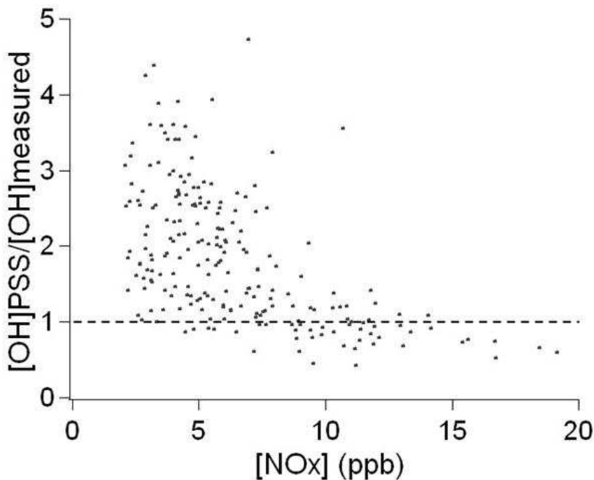
Fig. 7. Variation of the ratio between PSS calculated and observed OH concentrations with \text{NO}_x concentrations. The PSS calculated OH concentrations correspond to calculation from Eq. (12) (OH PSS1). The dotted line represents a ratio between calculated and measured OH of 1.
