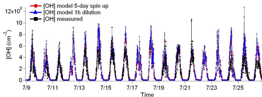
Fig. 8. Observed [OH] concentrations (black squares) compared with simulated [OH] concentrations by 5-day spin up scenario (red circles) and by 1h-dilution scenario (blue triangles) by MCM v3.1 implemented in a 0D boxmodel (see Sect. 3.2).
