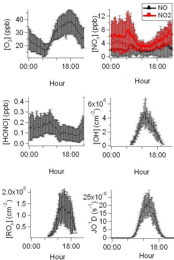
Fig. 3. Average diurnal 10 min profiles for O_3 , NO_x , HONO, OH, RO_2 and J(O^1D) during the MEGAPOLI summer campaign. Error bars correspond to standard deviation for the day to day variability.
