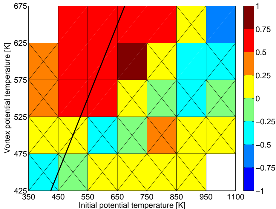
Fig. 10. Same as Fig. 9, but now the origin tracer is the fraction of vortex air in early winter originating from the potential temperature interval given at the horizontal axis on 1 September. Correlation coefficients not significant at the 95% level are crossed out. The black line is the line of zero subsidence.
