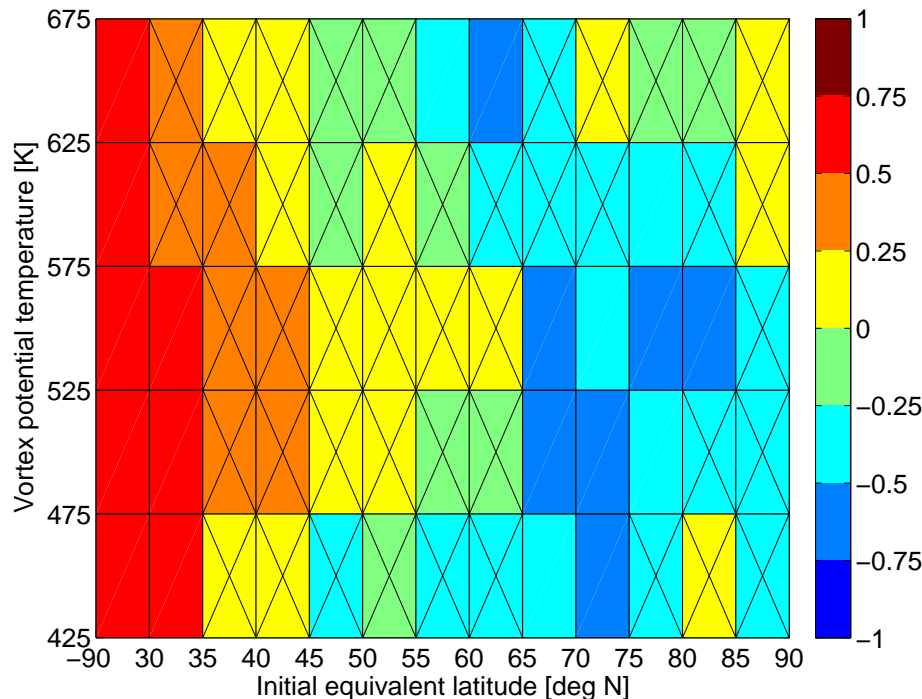
Fig. 14. Correlation of the origin of air inside the polar vortex and EP flux through mid latitudes in autumn. Each colored box shows the correlation coefficient of a time series of EP flux through a layer in autumn and a time series of an origin tracer in early winter at the same layer (1992–2009). The EP flux time series is the vertical component of the flux through the layer given at the vertical axis averaged over 45–75° N and from August to November. The origin tracer is the fraction of vortex air in early winter originating from the equivalent latitude intervals given at the horizontal axis on 1 September and averaged over the potential temperature intervals given at the vertical axis. Correlation coefficients not significant at the 95 % level are crossed out.
