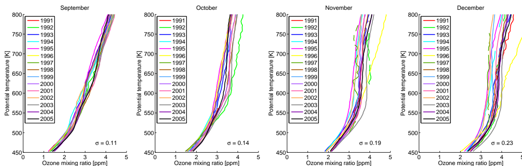
Fig. 1. Monthly mean profiles of ozone mixing ratios in the polar vortex for the months from September to December and the years 1991–2005. The vortex is defined as the area north of 65° N equivalent latitude. Measurements are from satellites and ozone sondes (see text for details). The standard deviation of the monthly mean ozone mixing ratios in the vortex at 550 K is shown for every month in the lower right corner.
