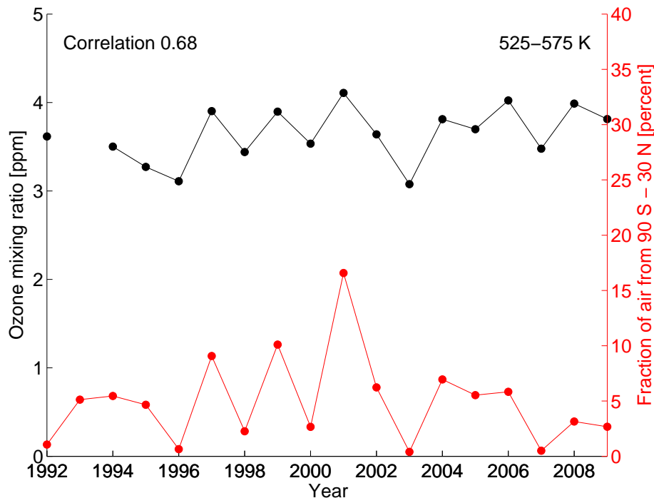
Fig. 6. Time series of vortex mean ozone mixing ratios at 525–575 K in early winter (30 December–8 January, 1992–2009, black), superimposed by a time series of the fraction of air in the polar vortex at 525–575 K which is originating south of 30° N equivalent latitude on 1 September (red).
