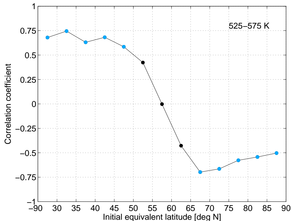
Fig. 8. Correlation of the origin of air inside the polar vortex and vortex mean ozone mixing ratios at 525–575 K. Correlation of a time series (1992–2009) of vortex mean ozone mixing ratios in early winter at 525–575 K and a time series of the fraction of air in the vortex in early winter at 525–575 K originating from the equivalent latitude intervals given at the horizontal axis on 1 September. Correlation coefficients significant at the 95% level are shown in blue.
