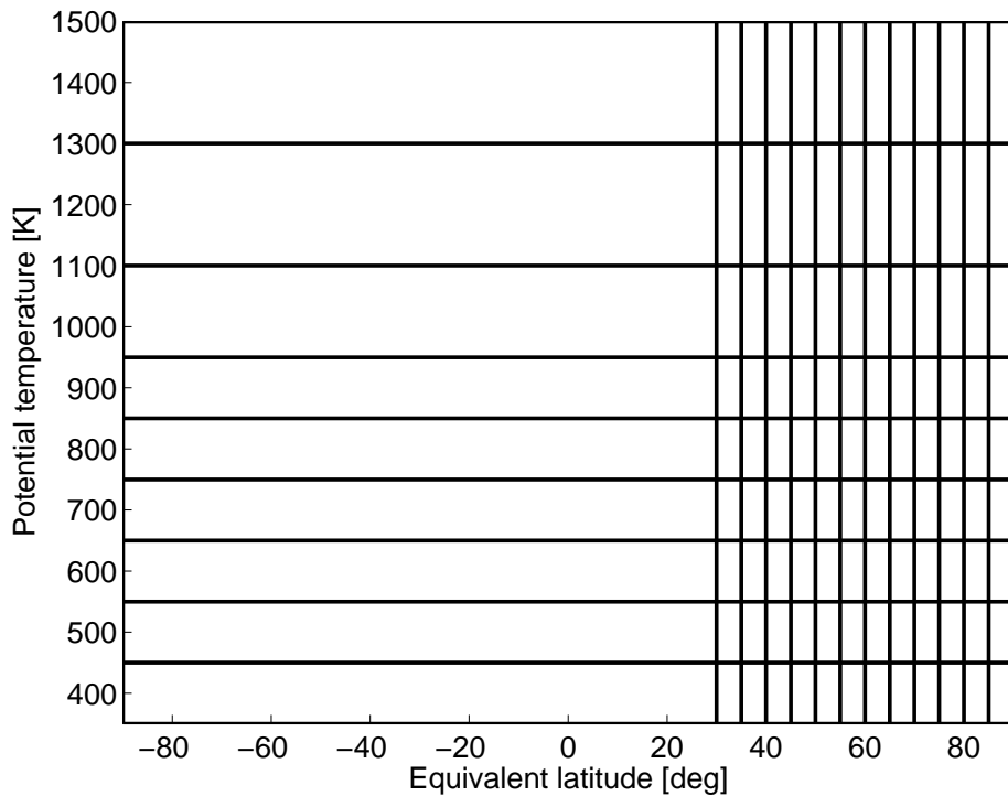
Fig. 4. Setup of the tracers at the start of the model run.
