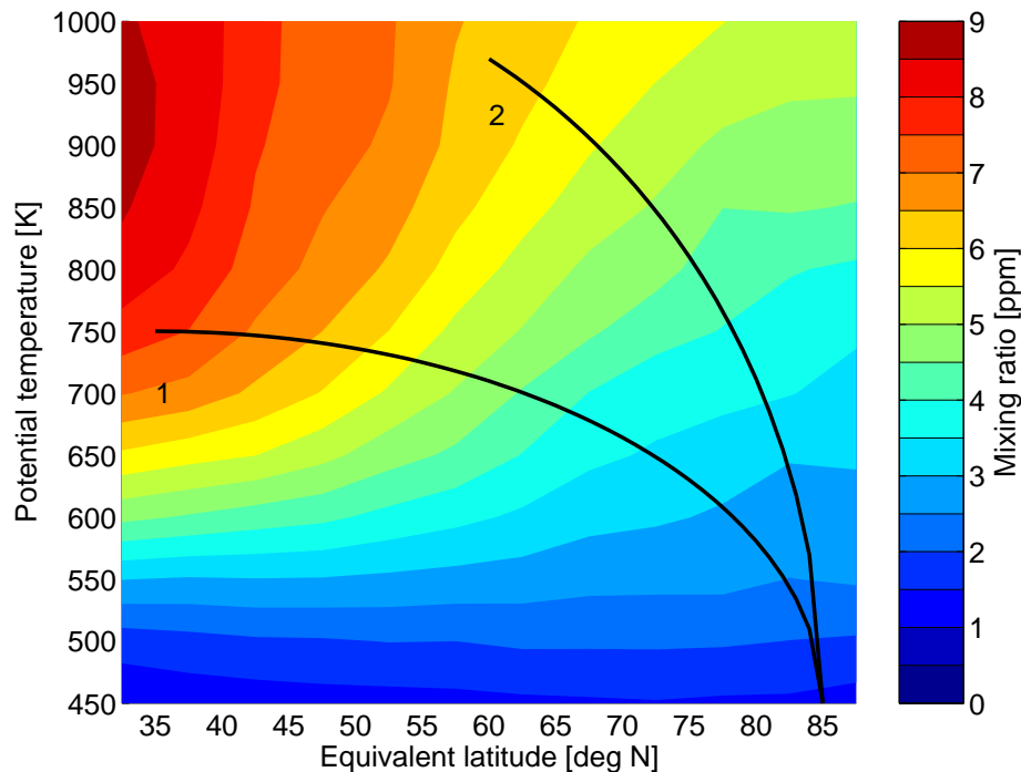
Fig. 12. Schematical illustration of the pathway of air in two years with extreme conditions. Colors show the mean ozone distribution in September. Pathway 1 shows the situation in years with a high fraction of air from low latitudes enclosed in the vortex, which is typically also connected with low subsidence. Due to the mean ozone distribution, this leads to relatively high ozone values in the vortex. This situation is also typically connected with a strong Brewer-Dobson circulation and a high EP flux through the tropopause. Pathway 2 shows the situation in years with a low fraction of air from low latitudes enclosed in the vortex, which is typically connected with high subsidence, low ozone and a weak Brewer-Dobson circulation.
