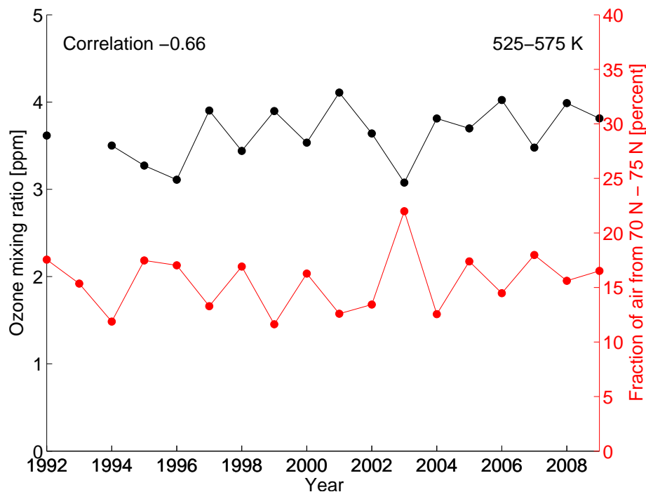
Fig. 7. Time series of vortex mean ozone mixing ratios at 525–575 K in early winter (30 December–8 January, 1992–2009, black), superimposed by a time series of the fraction of air in the polar vortex at 525–575 K which is originating from 70° N to 75° N equivalent latitude on 1 September (red).
