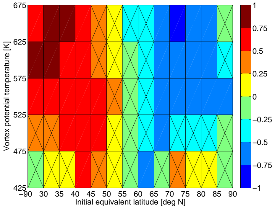
Fig. 9. Correlation of the origin of air inside the polar vortex and vortex mean ozone mixing ratios. Each colored box shows the correlation coefficient of a time series of vortex mean ozone mixing ratios in early winter and a time series of an origin tracer in early winter (1992–2009). The ozone time series is averaged over the potential temperature layers indicated at the vertical axis. The labels of the axis give the endpoints of the 50 K intervals. The time series of the origin tracer is the fraction of vortex air in early winter originating from the equivalent latitude intervals given at the horizontal axis on 1 September and averaged over the potential temperature intervals given at the vertical axis. Correlation coefficients not significant at the 95 % level are crossed out.
