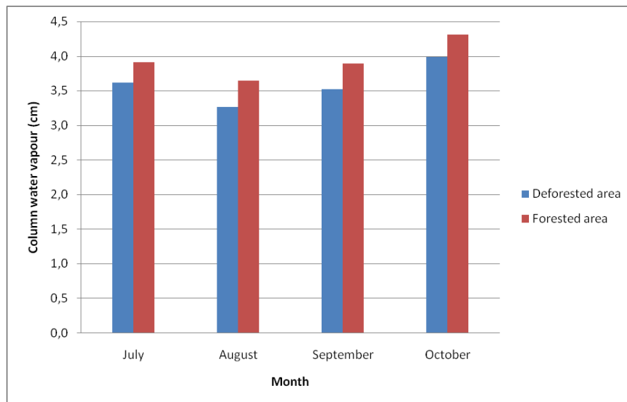
Fig. 7. Column water vapour content retrieved by AERONET sunphotometers at a deforested area (located at 10.76^{\circ} S, 62.36^{\circ} W) and a forested area (located at 10.08^{\circ} S, 61.93^{\circ} W) from July to October 2002.
