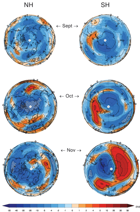
Fig. 7. Left column: polar stereographic projection of changes in total ozone (in DU) for the NH from September to November resulting from the Carrington-like event. Right column: same for the SH. Hatched areas show 95 % statistical significance.
