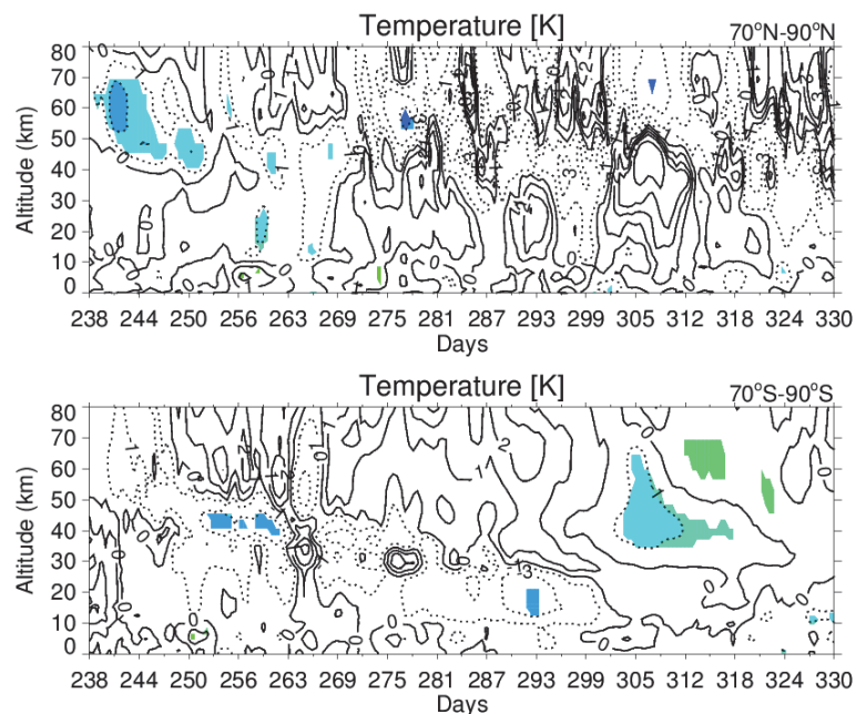
Fig. 5. Upper panel: evolution of changes in zonal mean temperature profile for the polar region (70–90° N) in Kelvin. Lower panel: same for 70–90° S. Colors indicate areas with at least 95% statistical significance. Contour levels: -10 , -6 , -3 , -1 , 0 , 1 , 2 , 3 , 5 , 10 K.
