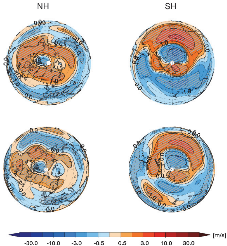
Fig. 6. Upper row: polar stereographic projection of zonal wind changes at 25 hPa from August to November given in \text{ms}^{-1} . Lower row: zonal wind changes at 63 hPa from August to November given in \text{ms}^{-1} . Left column: NH. Right column: SH. Hatched areas show 95 % statistical significance.
