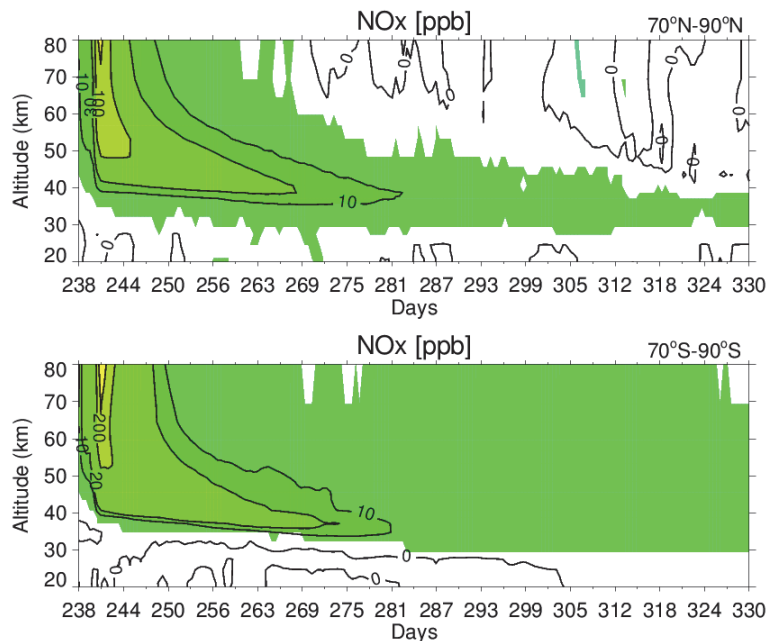
Fig. 2. Upper panel: evolution of changes in \text{NO}_x zonal mean mixing ratio profile in the polar regions ( 70\text{--}90^\circ\text{N} ). Lower panel: same for 70\text{--}90^\circ\text{S} . Colors indicate areas with at least 95% statistical significance. Upper panel contour levels: 10, 30, 100, 200 ppbv. Contour levels lower panel: 10, 20, 200, 300 ppbv.
