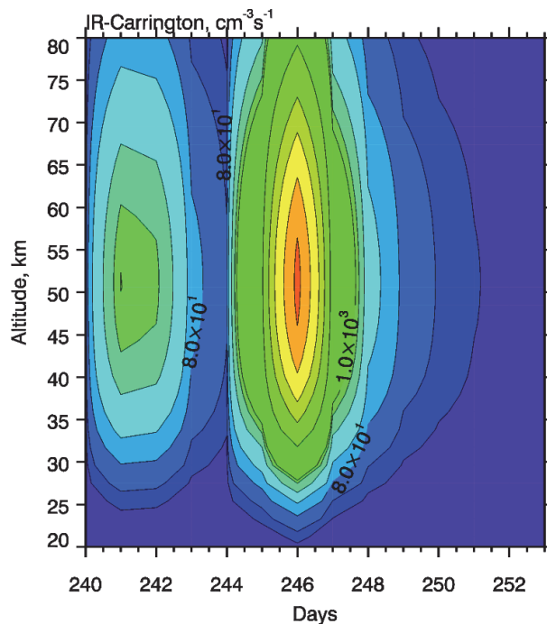
Fig. 1. Height versus time evolution of ionization rates for the investigated Carrington-like solar proton event. The particular shape with two major episodes within 5 days is taken from the event of August 1972. Contour levels: 0, 5, 20, 80, 200, 500, 800, 1000, 4000, 8000, 12 000, 18 000, 25 000, 30 000 ion pairs \text{cm}^{-3} \text{s}^{-1} .
