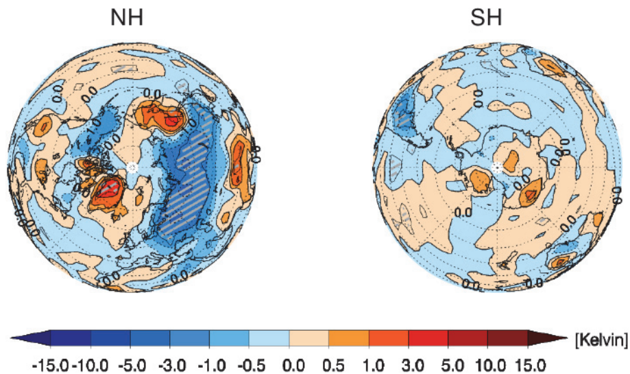
Fig. 8. Left panel: polar stereographic projection of changes in surface air temperature for the NH for November resulting from the Carrington-like event. Right panel: same for the SH. Hatched areas show 95 % statistical significance.
