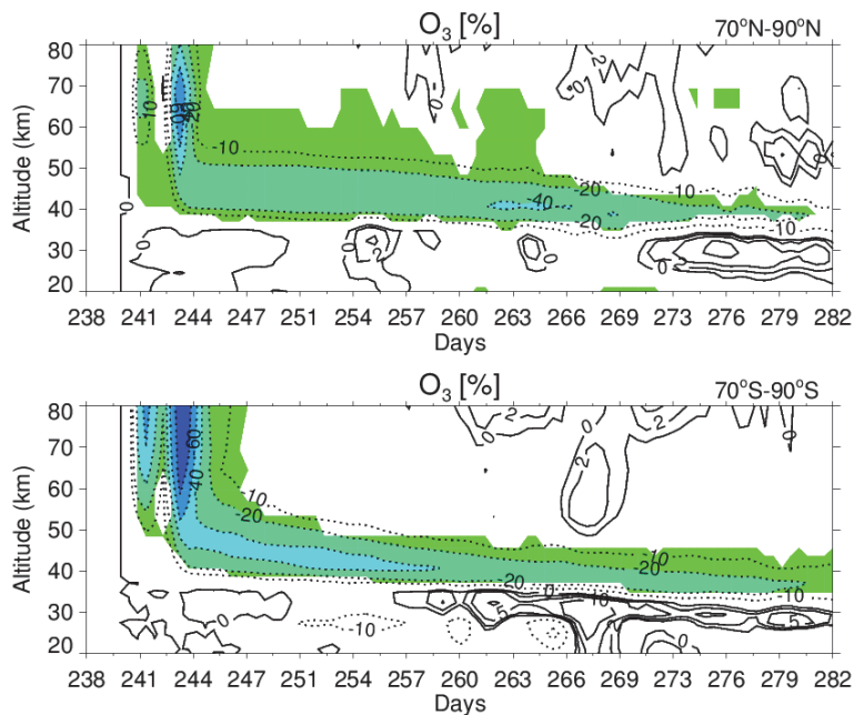
Fig. 4. Upper panel: evolution of changes in ozone zonal mean mixing ratio profile in the polar region (70–90° N) in percent. Lower panel: same for 70–90° S. Colors indicate areas with at least 95% statistical significance. Contour levels: –100, –80, –60, –40, –20, –10, 0, 2, 5, 10, 50%.
