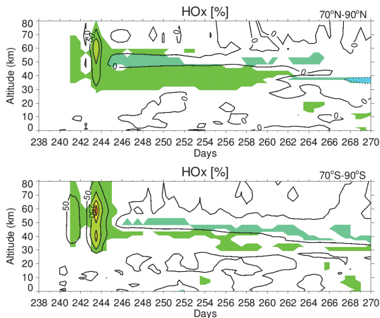
Fig. 3. Upper panel: evolution of changes in \text{HO}_x zonal mean mixing ratio profile in the polar region ( 70\text{--}90^\circ\text{N} ) in percent. Lower panel: same for 70\text{--}90^\circ\text{S} . Colors indicate areas with at least 95% statistical significance. Contour levels for upper panel: -20, 0, 50, 150, 300\% . Contour levels for lower panel: -20, 0, 50, 250, 700, 1000\% .
