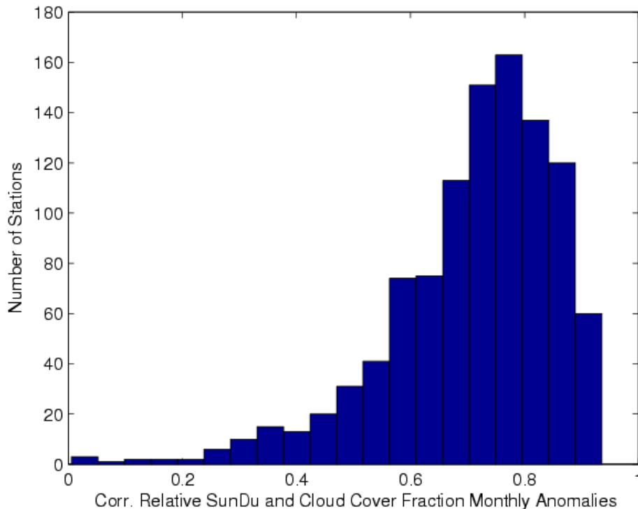
Fig. 10. Histogram of correlations between the relative SunDu (the ratio of measured SunDu to theoretical SunDu during a day) and monthly anomalies of total cloud cover fraction. Total cloud cover fraction is observed visually by trained technicians at weather stations. The plot shows that relative SunDu is highly correlated with cloud cover fraction on a monthly scale at most stations.
