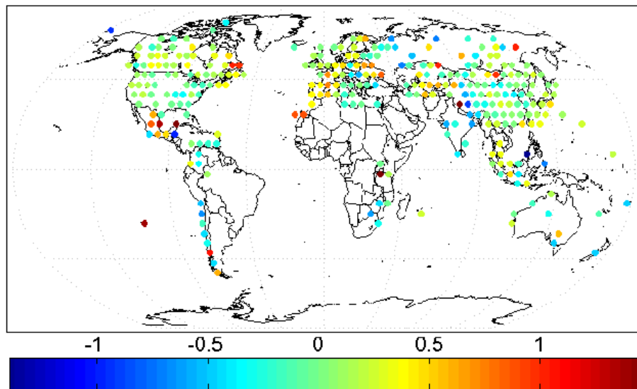
Fig. 13. The linear trend of R_s from 1982 to 2008 (unit: \text{Wm}^{-2} per year) by merging SunDu-derived values and direct measurements collected by GEBA. The trends are first calculated at each station and then aggregated into a 5^\circ \times 5^\circ grid and the averages are shown. There are 302 such grids obtained and shown.
