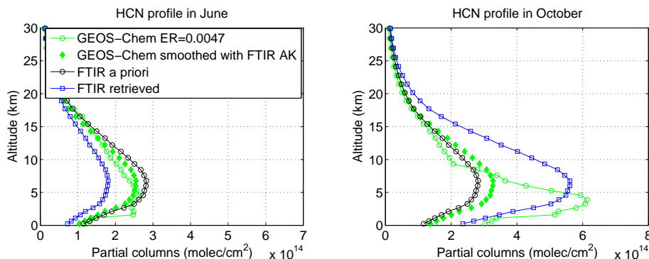
Fig. 6. Example of FTIR and GEOS-Chem HCN profiles (in Partial Columns, molec cm -2 ) in June and October.
