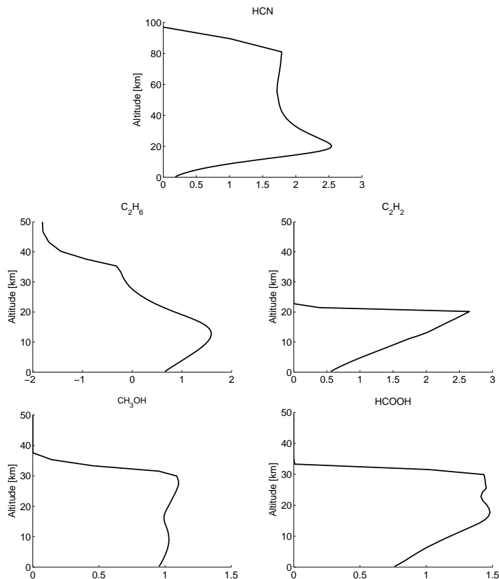
Fig. 3. FTIR total column averaging kernels (molec cm -2 molec cm -2 ) of the five retrieved species.
