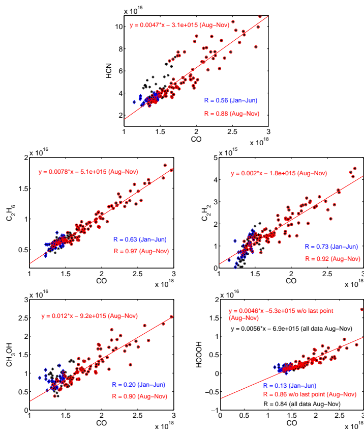
Fig. 5. Correlation plots of daily mean total columns of the five retrieved species versus CO (molec cm -2 ). The correlation coefficient ( R ) is given for the periods from January to June (blue), and from August to November (red). For the latter period, the slope ( \Delta X/\Delta \text{CO} ) and the intercept from a linear least-squares fit of the data are also given.
