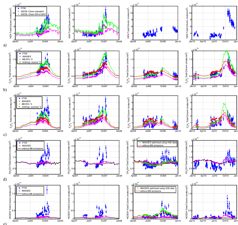
Fig. 4. Time-series of daily mean total columns at Reunion Island from: FTIR and GEOS-Chem HCN (a), FTIR and IMAGES C_2H_6 (b), C_2H_2 (c), CH_3OH (d), and HCOOH (e). From left to right, the columns cover the years 2004, 2007, 2009, and 2010. The FTIR data are represented by the blue filled circles, different model simulations with the coloured lines (magenta for the standard runs; green and red for the sensitivity tests: see Sect. 5), and the model data smoothed with the FTIR averaging kernels with the open circles. For CH_3OH and HCOOH , the model simulations obtained when the biomass burning contribution is removed are shown in black for the standard run, and in red for the inversion using IASI data. (BB: biomass burning; ER: emission ratio; EF: emission factor; Anthrop.: anthropogenic).
