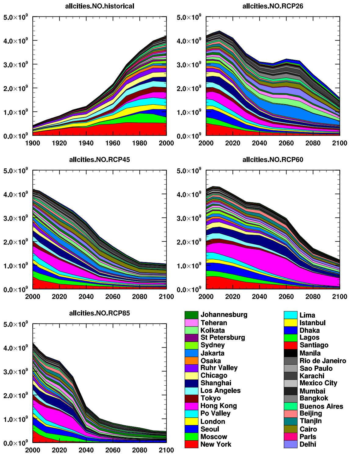
Figure S1: Emissions of NO (Tg yr -1 ) from megacities considered in this study
