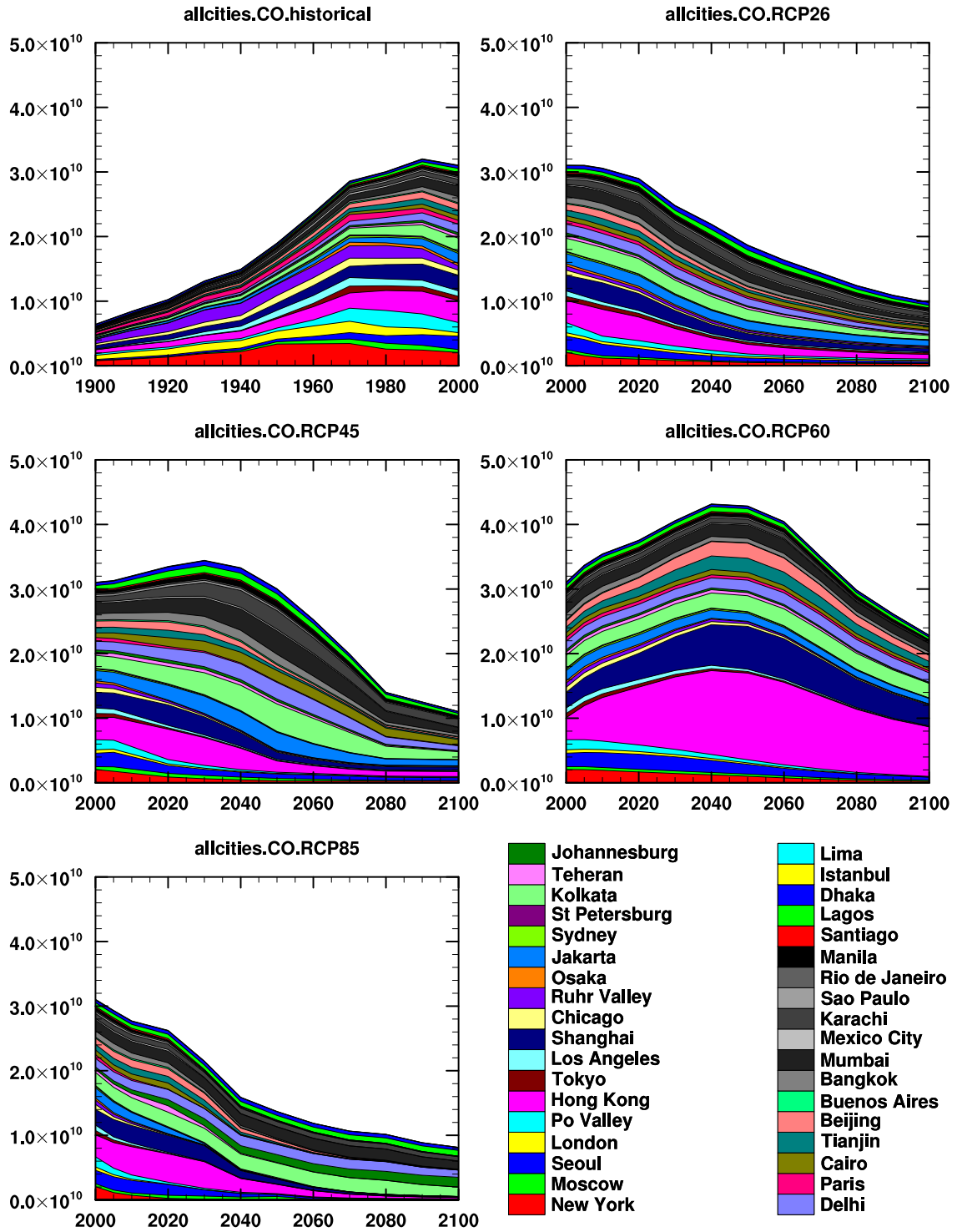
Figure S2: Emissions of CO ( \text{Tg yr}^{-1} ) from megacities considered in this study
