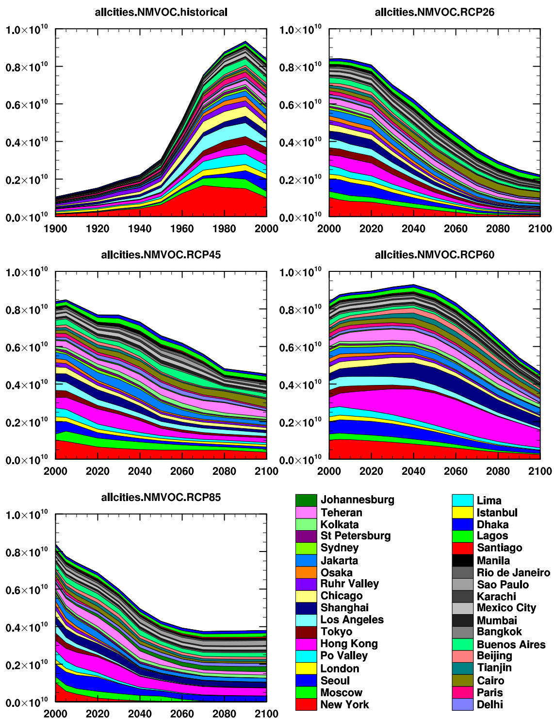
Figure S3: Emissions of NMVOC (Tg yr -1 ) from megacities considered in this study
