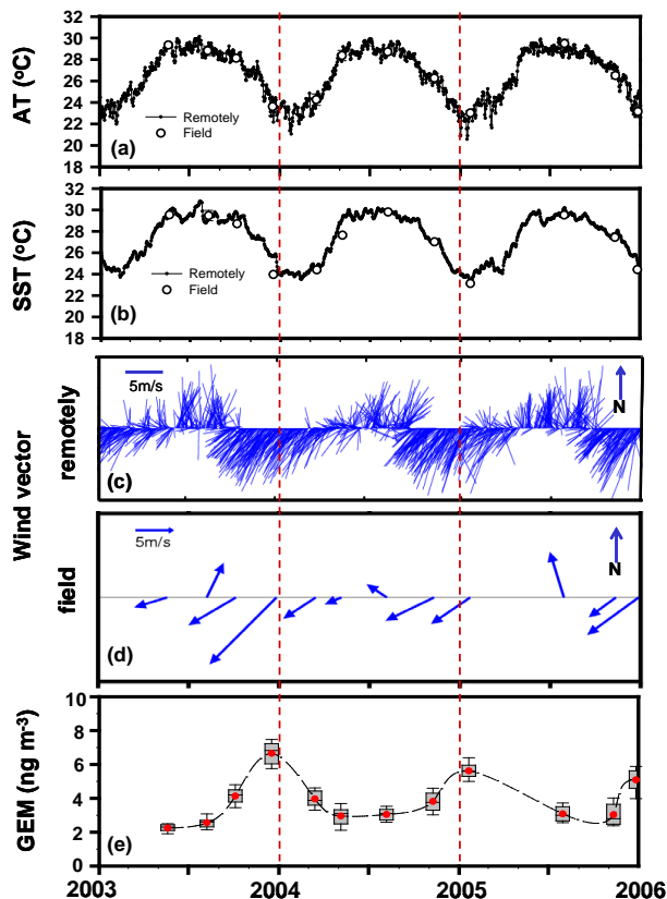
Fig. 2. Time-series of records obtained for the SEATS station over Northern South China Sea during the study period from August 2003 to December 2005. (a) Remotely sensed surface air temperature (AT • and field observed, ○); (b) remotely sensed sea surface temperature (SST • and field observed, ○); (c) remotely sensed wind vector and speed (WS); (d) field observed wind data; (e) averaged GEM. Boxes represent interquartile ranges, bars delineate upper and lower 10%, and the center line is the median; means are shown by red •.
