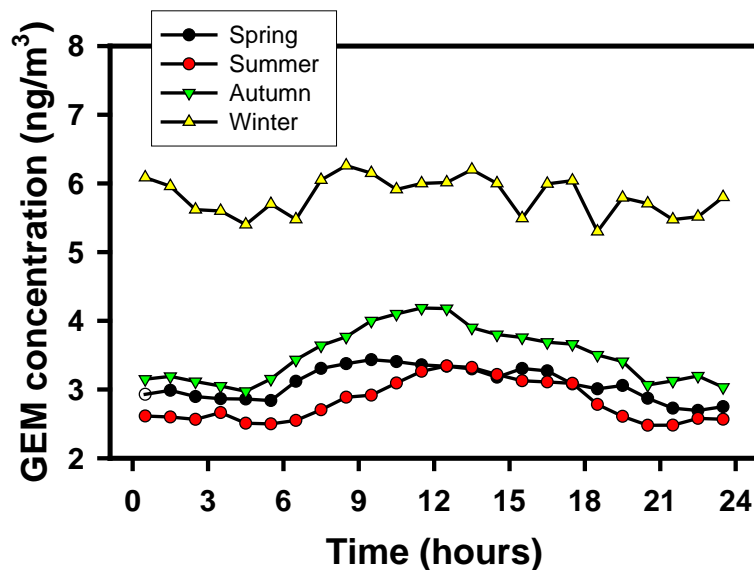
Fig. 3. Seasonal changes in diurnal GEM cycle over the Northern SCS based on seasonal average concentrations for each hour. Each seasonally diurnal plot has an average of 3 cruises.
