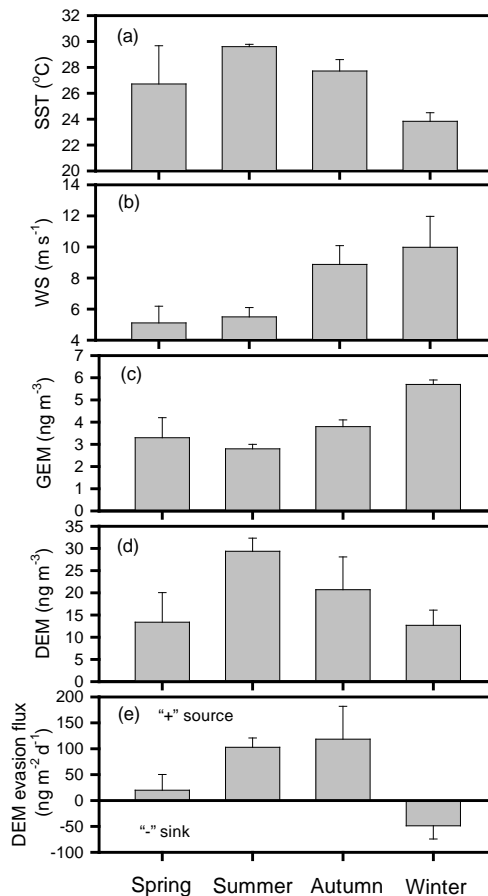
Fig. 4. Summary of seasonal average data for (a) SST; (b) WS; (c) GEM; (d) DEM and (e) air-sea Hg 0 exchange flux between 2003 and 2005 at SEATS station in the SCS. Each seasonal bar has an average of 3 cruises with an error of \pm 1 SD ( n = 3 ).
