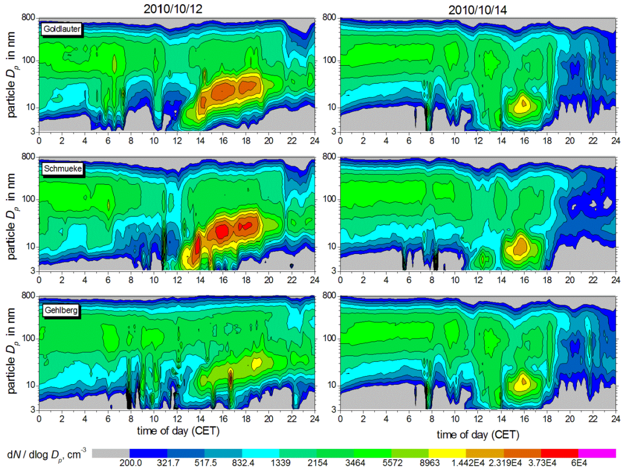
Fig. S1: The particle number size distributions at upwind (Goldlauter), summit (Schmueke), and downwind (Gehlberg) sites.
