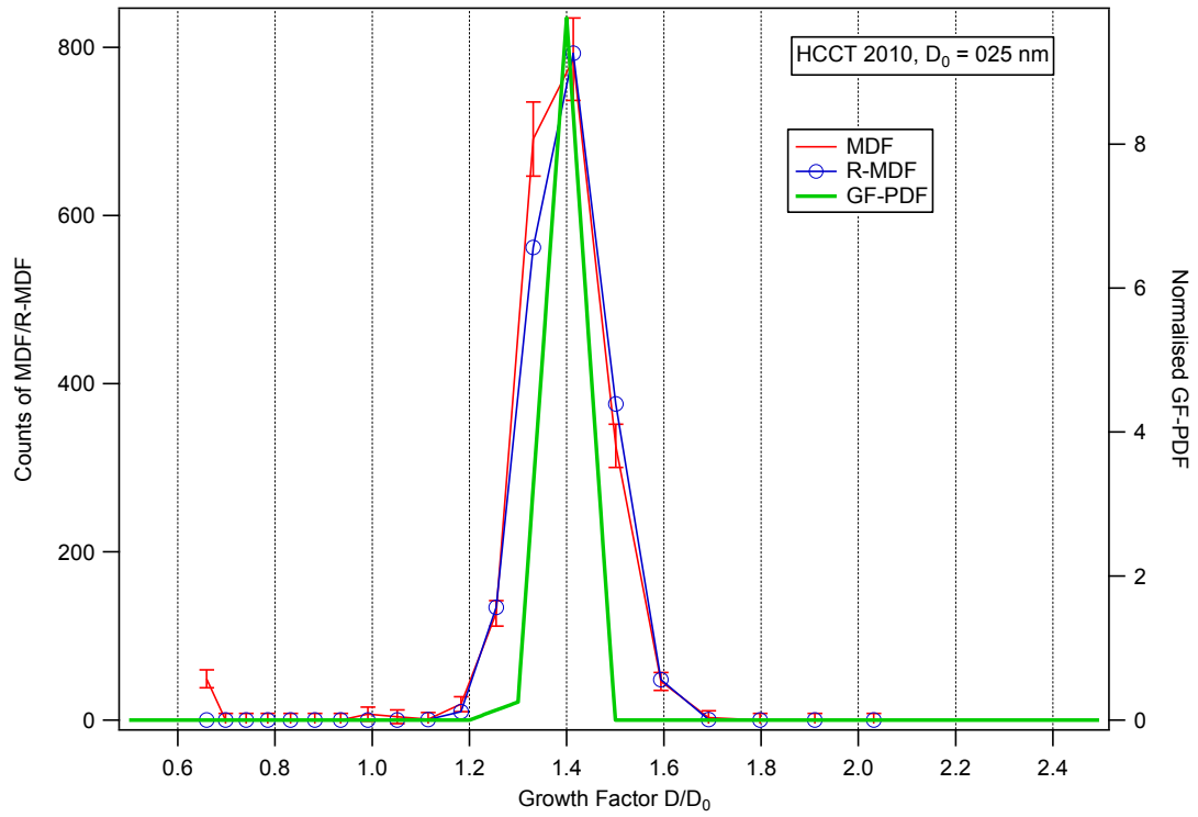
Fig. S2: An example of hygroscopic growth probability distribution (GF-PDF) during the NPF event.
