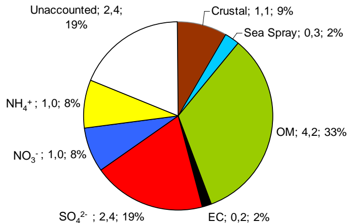
Fig. 3. Mean PM 2.5 composition ( \mu\text{g m}^{-3} ) at MSY for the study period (2002–2010).
