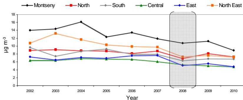
Fig. 1. PM 2.5 concentrations measured at RB sites across Spain from 2002–2010 (year of most significant decrease highlighted).
