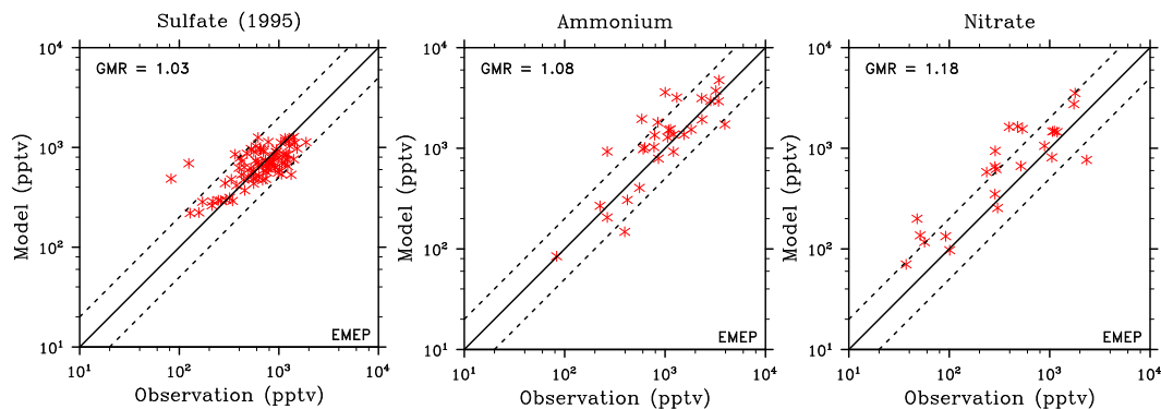
Fig. A2. Modeled and observed annual average concentrations for sulfate, ammonium and nitrate aerosols from the EMEP (Europe) network.
