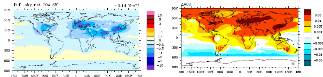
Fig. 8. Annual mean distribution of the simulated radiative effects of nitrate and ammonium at the top of atmosphere (TOA) for the full-sky condition for the PD simulation (left) and global annual mean distribution of the difference in aerosol optical depth at 550 nm ( \Delta\text{AOD} ) between the simulations with and without ammonium and nitrate aerosols for the PD scenario (right).
