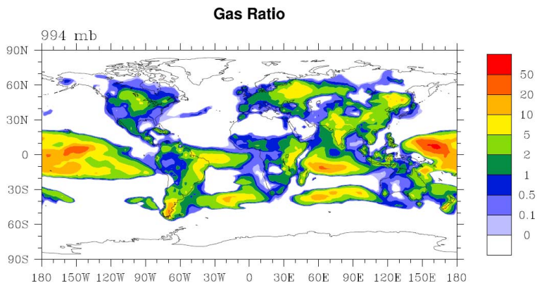
Fig. 4. Annual average molar ratio of total ammonium to total sulfate (top) and gas ratio (bottom) in the the surface layer. See text for the definition of the gas ratio.
