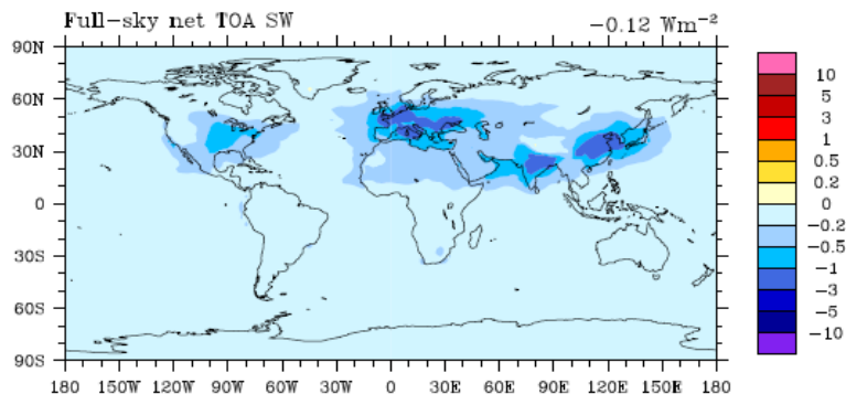
Fig. 9. Annual mean direct anthropogenic forcing of nitrate and ammonium from the PI to PD scenario for full-sky conditions.
