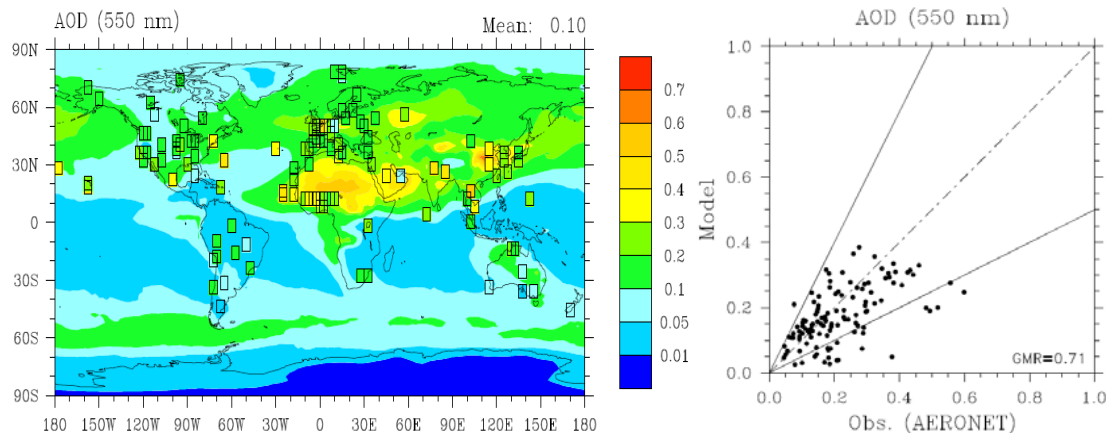
Fig. 6. Global annual mean distribution (left) and scatter plot (right) of modeled aerosol optical depth and observational data from AERONET at 550 nm. The geometric mean ratio (GMR) between modeled and observed values is given.
