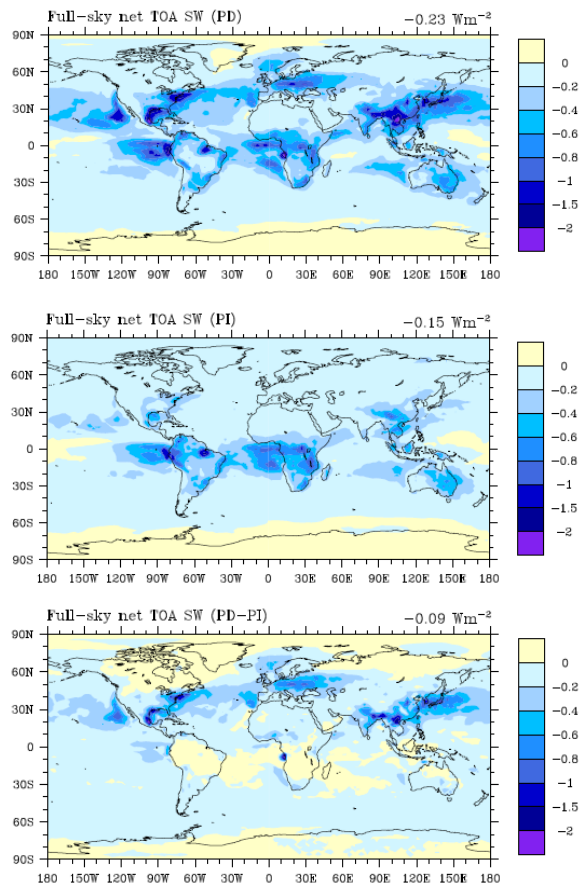
Fig. 16. The first aerosol indirect effect of total nitrate (gas plus aerosol) and ammonium for the PD (top), PI (middle) simulation and the PD-PI anthropogenic aerosol indirect forcing (bottom) at the top of atmosphere (TOA). The mean forcing value is indicated in each panel.
