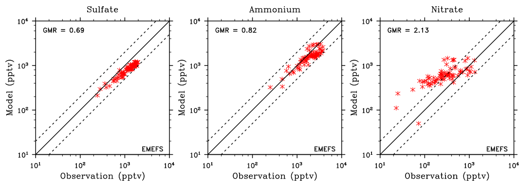
Fig. A1. Modeled and observed annual average concentrations for sulfate, ammonium and nitrate aerosols from the EMEFS (North America) network.
