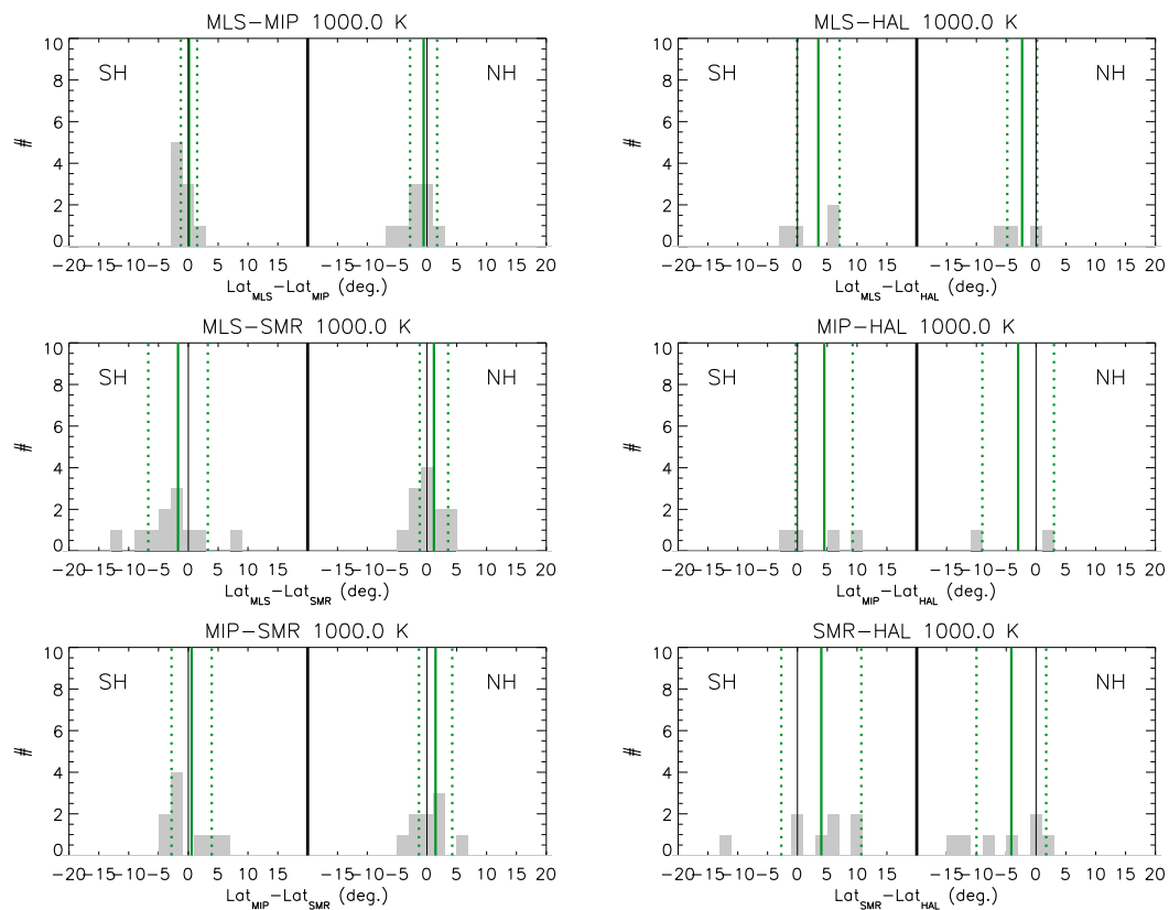
Fig. 7. the same as Fig. 1 at 1000 K
