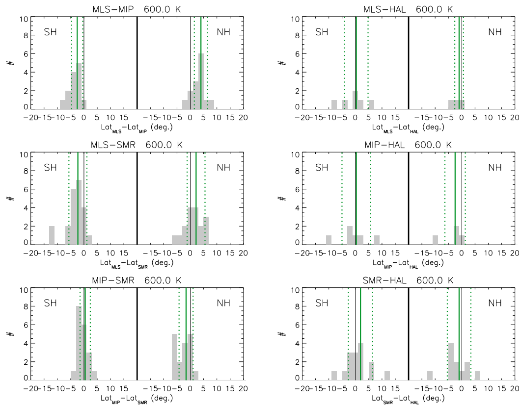
Fig. 2. the same as Fig. 1 at 600 K.
