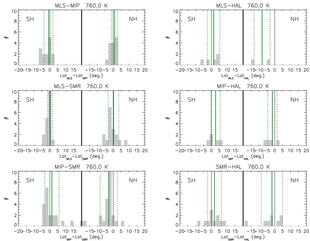
Fig. 4. the same as Fig. 1 at 760 K
