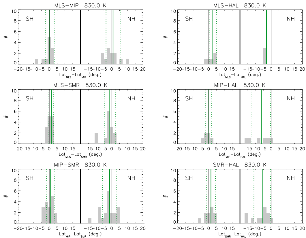
Fig. 5. the same as Fig. 1 at 830 K.
