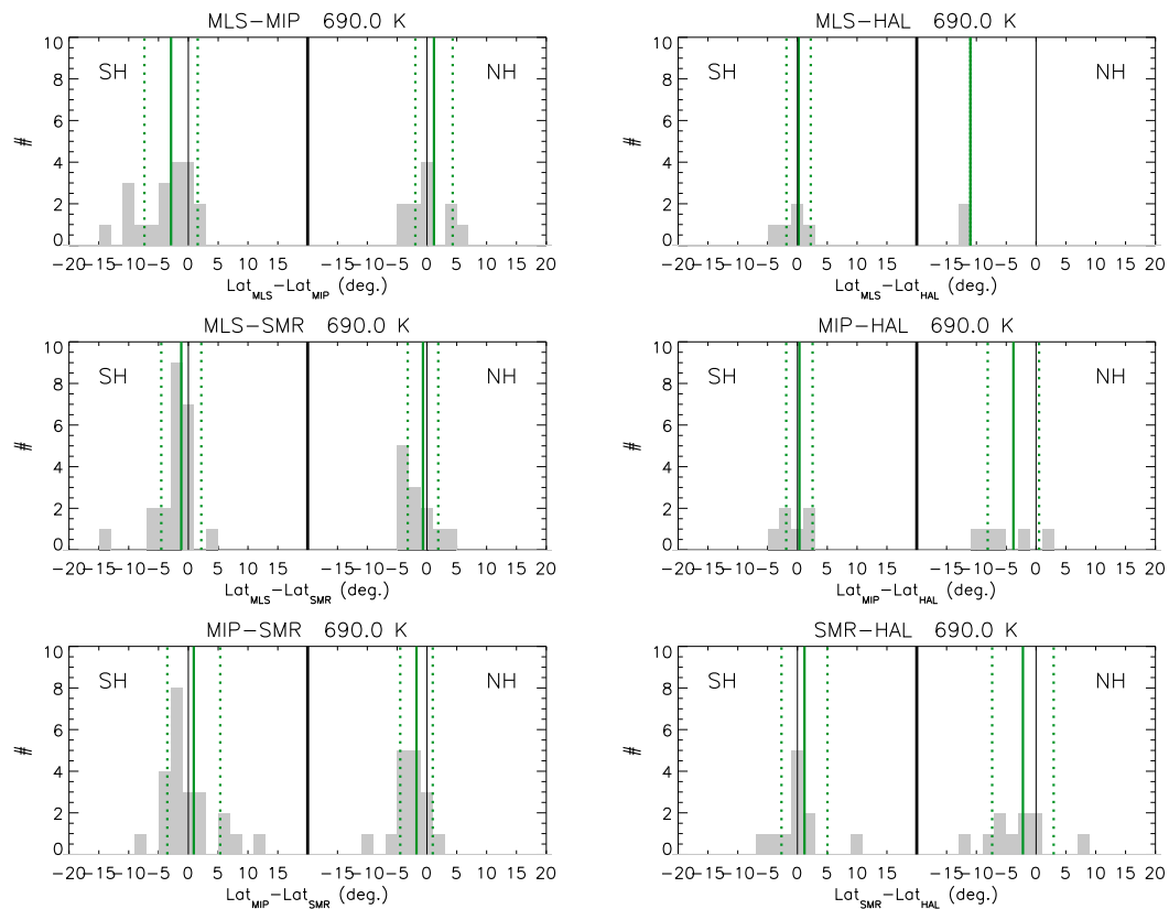
Fig. 3. the same as Fig. 1 at 690 K.
