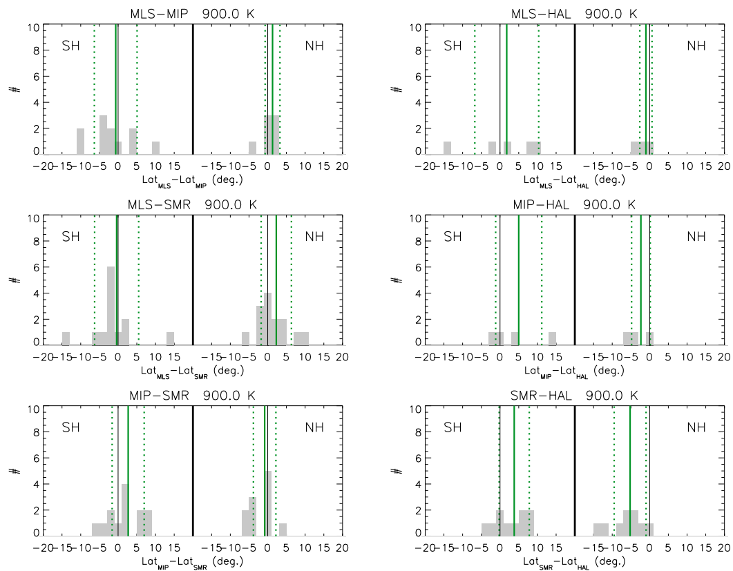
Fig. 6. the same as Fig. 1 at 900 K
