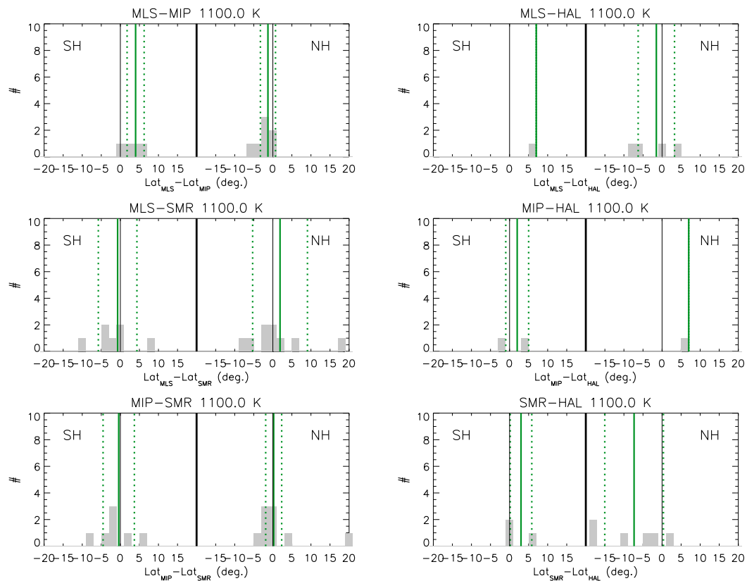
Fig. 8. the same as Fig. 1 at 1100 K
