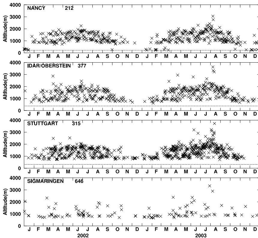
Fig. 3. BLH estimated from radiosonde (IGRA) data in 2002 and 2003.
