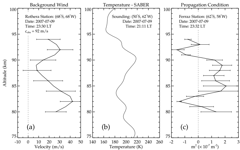
Fig. 2. (a) Wind profile in the bore propagation direction. (b) Temperature profile obtained by SABER on 09 July 2007. (c) Vertical wavenumber squared ( m^2 ).
