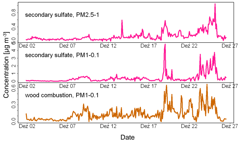
Figure 2: Comparison of time series of secondary sulfate in the smallest and intermediate size range as well as wood burning in the smallest size range.
