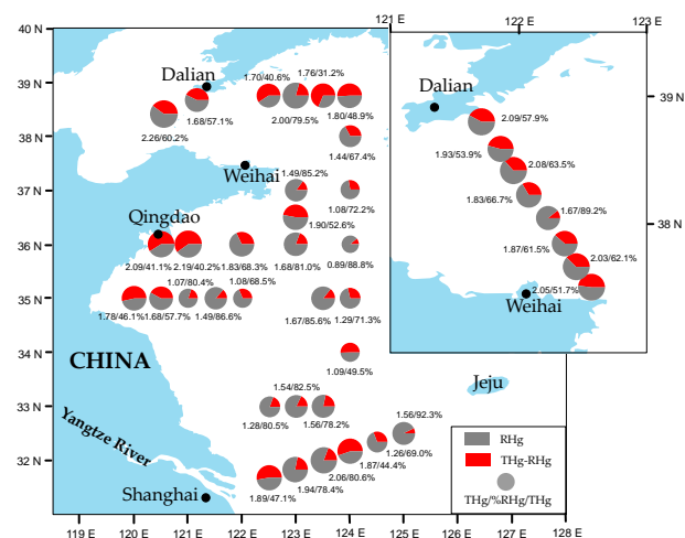
Figure 5. Spatial distribution of the total Hg (THg, unit in ng l -1 ) and reactive Hg (RHg) and RHg/THg ratios in the surface waters of the Yellow Sea during the cruise in July 2010.
