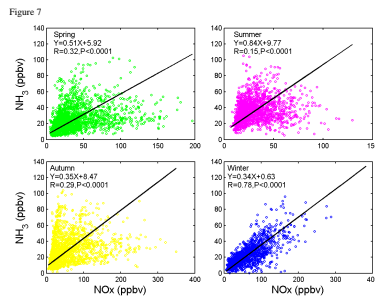
Fig.7 The 2-sided regression of \text{NH}_3 versus \text{NO}_x at CMA from June 2009 to May 2010.
