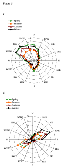
Fig.5 Seasonal average \text{NH}_3 concentrations at CMA (a), wind frequency at CMA (b), wind speed at CMA (c) and wind frequency at SDZ (d) distributions in different wind direction sectors during 2009-2010.
